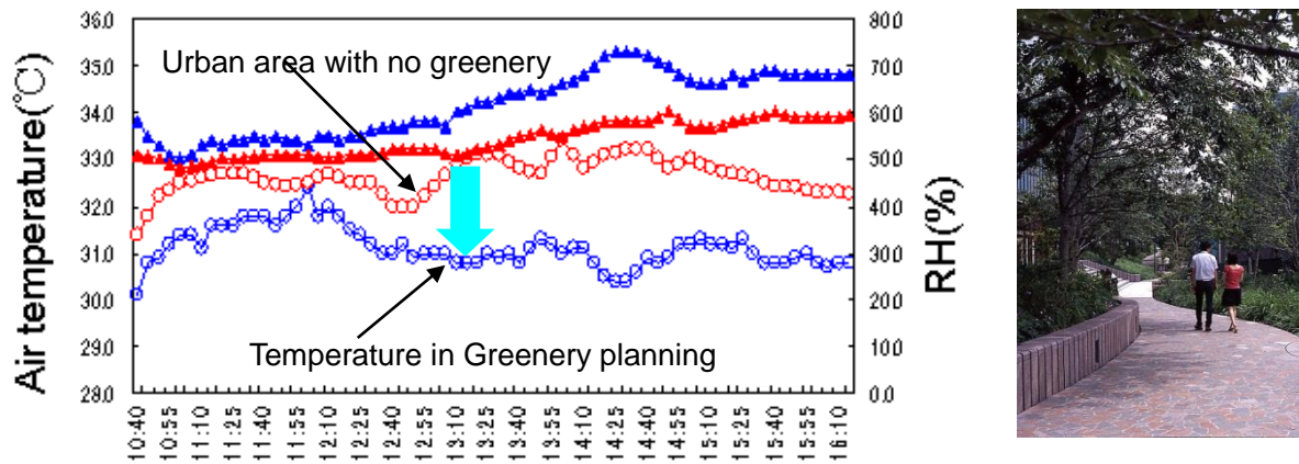
Figure 18 Mitigation effect of air temperature by greenery area (12:00, September, Tokyo, 2005)
