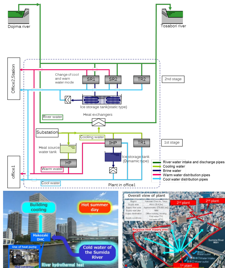
Fig.3.2-4. High Efficient DHC system Using Thermal Energy of River Water in Hakozi, Japan Source: NSRI
