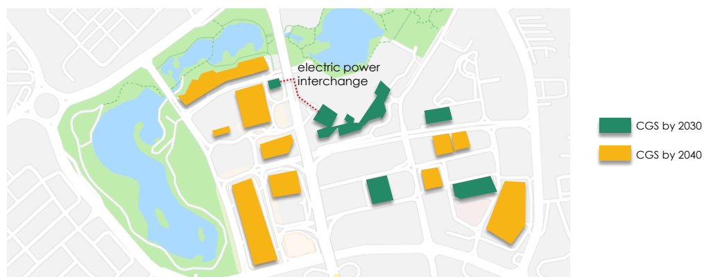
Fig. 5.3-10. Introduction plan for Cogeneration system
