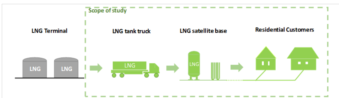
Figure 3-16 Illustration of SSLNG in the residential sector
