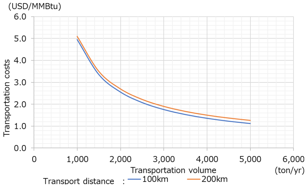
Figure 3-7 Influence of changes in transportation distance and volume in the transport unit price in the model case
