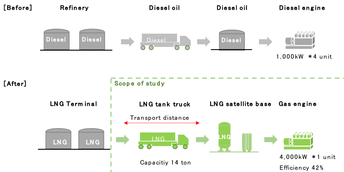
Figure 3-8 Illustration of diesel replacement in power generation
