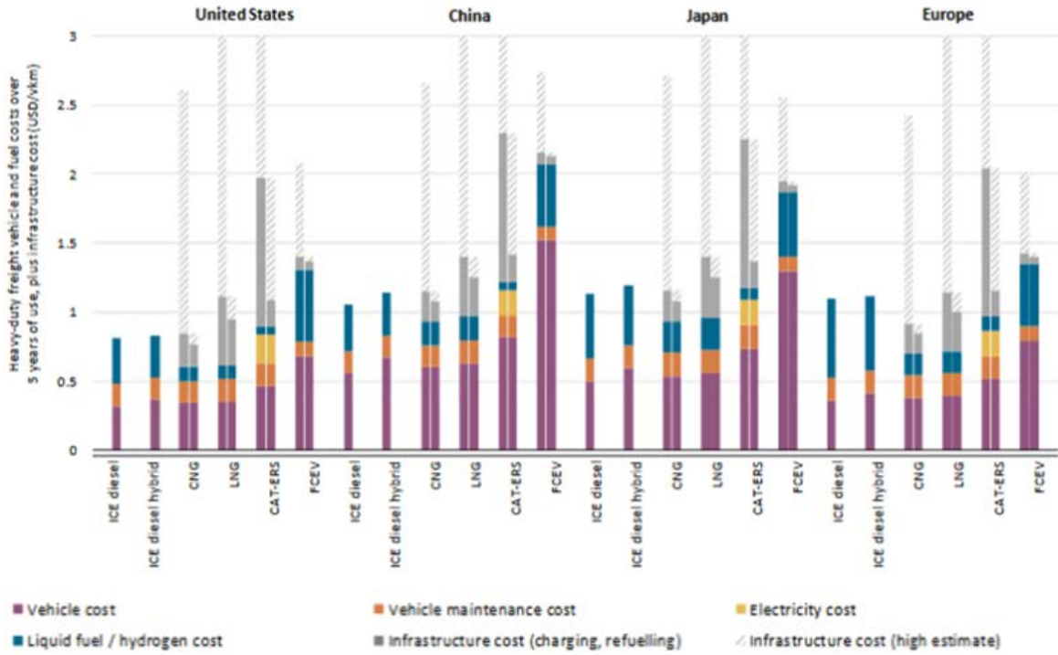
Figure 3-17 Cost of alternative fuelled vehicles in each region
