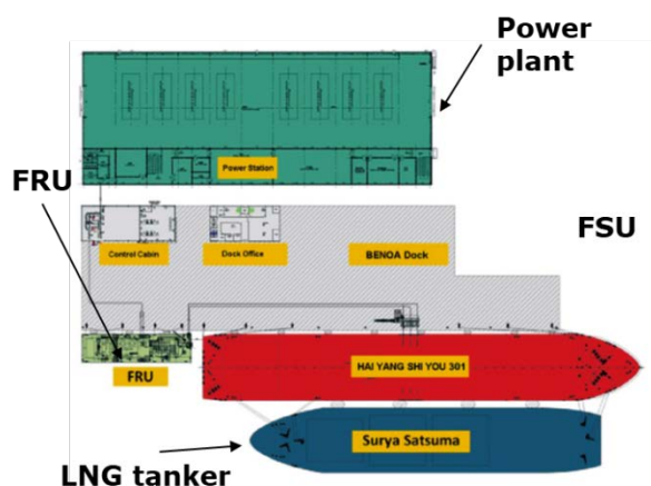
Figure 5-3 Layout of SSLNG assets in Benoa
