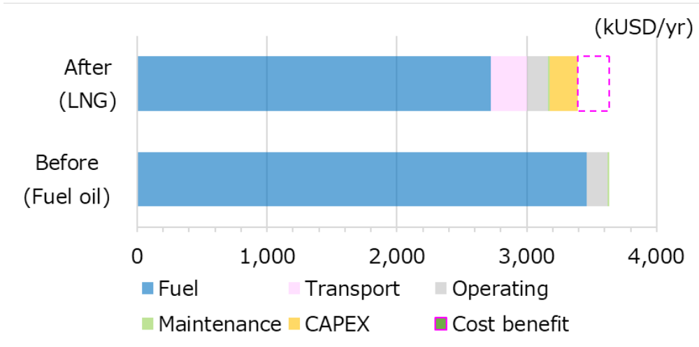
Figure 3-14 Cost reductions in the industrial sector
