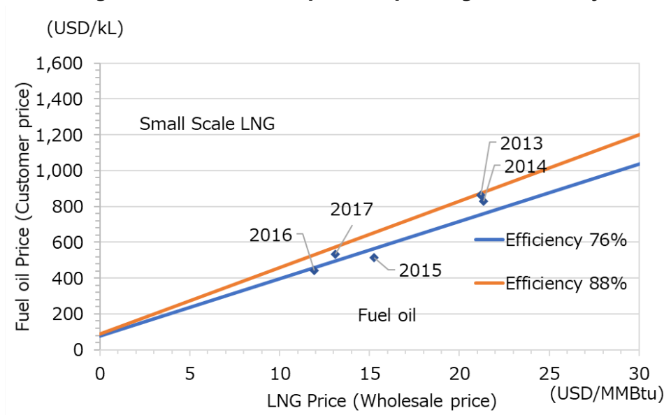
Figure 3-15 Break-even prices depending on efficiency
