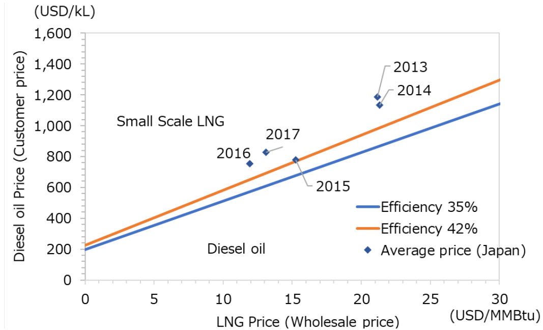
Figure 3-11 Break-even prices depending on efficiency
