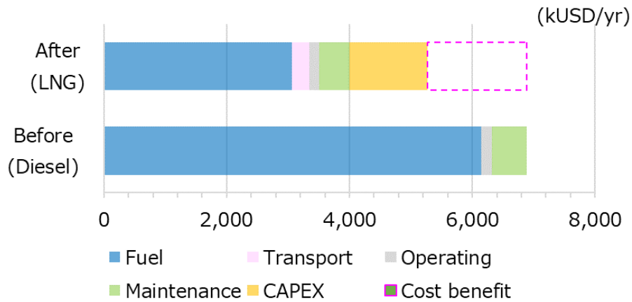
Figure 3-10 Cost reductions in power generation
