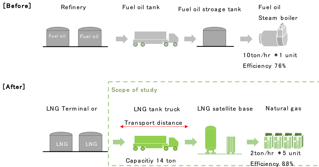
Figure 3-12 Replacement for SSLNG in the industrial sector
