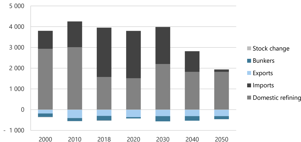
Figure 11-38. Refined product production, imports, and exports in CN, 2000-2050 (PJ).
