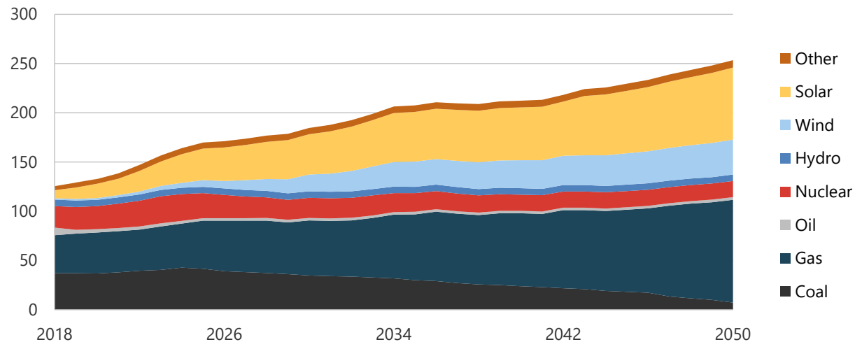
Figure 9-15. Generation capacity in REF, 2018-2050 (GW).
