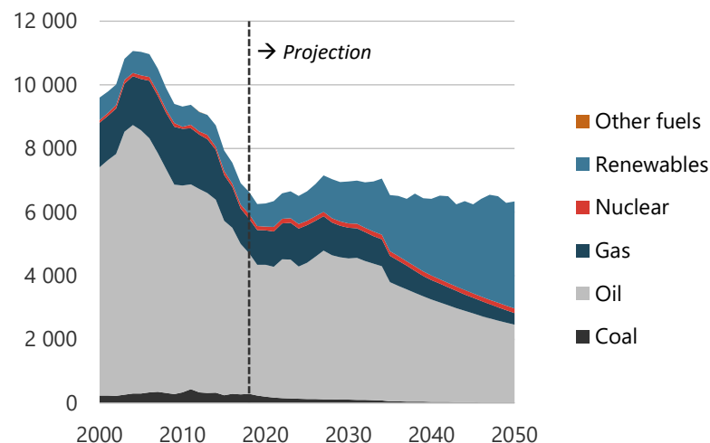
Figure 11-21. Energy production in CN, 2000-2050 (PJ).
