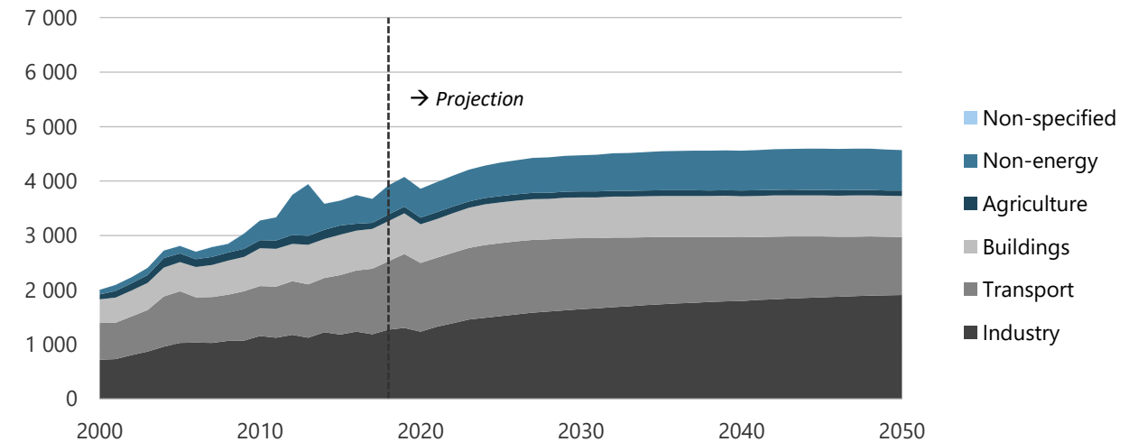
Figure 19-6. Energy demand by sector in CN, 2000-2050 (PJ).
