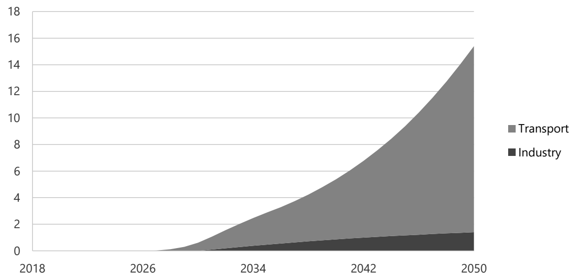
Figure 18-41. Hydrogen consumption by sector in REF, 2000-2050 (PJ).
