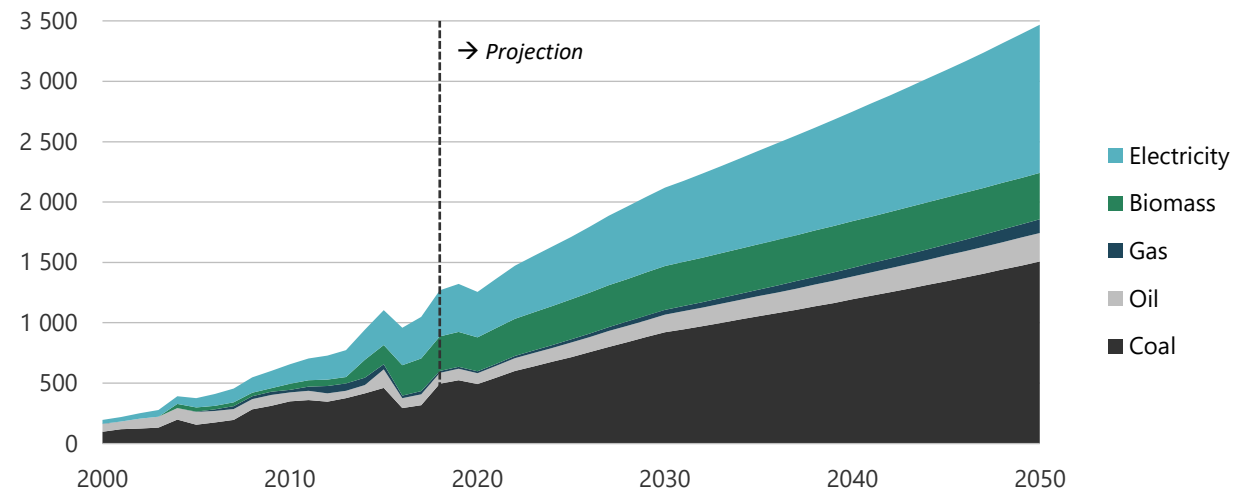
Figure 21-9. Industry energy demand in REF, 2000-2050 (PJ).
