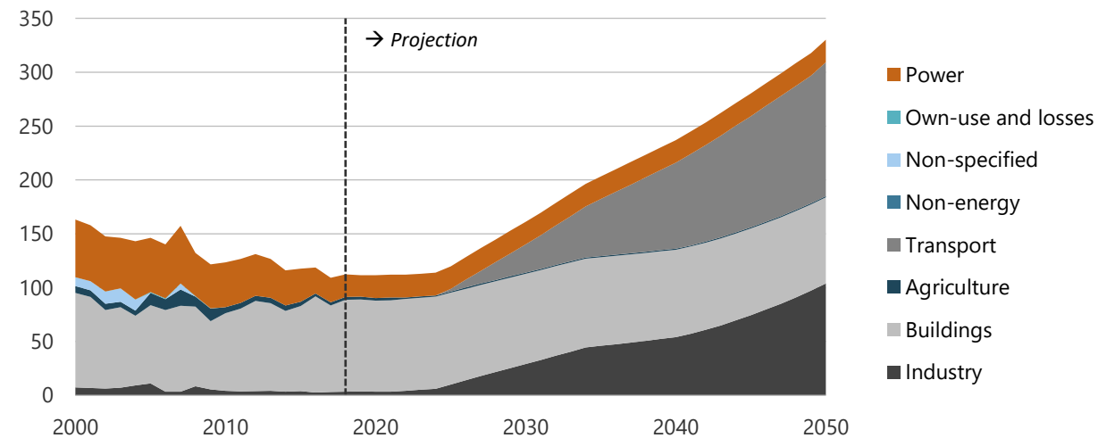
Figure 16-42. Bioenergy consumption by sector in CN, 2000-2050 (PJ).
