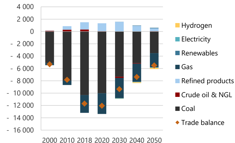
Figure 1-24. Net energy trade in CN, 2000-2050 (PJ).
