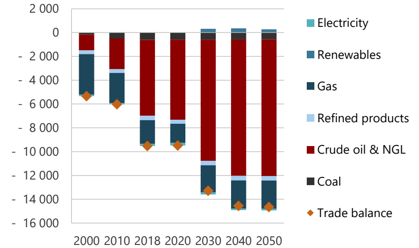
Figure 3-21. Net energy trade in REF, 2000-2050 (PJ).
