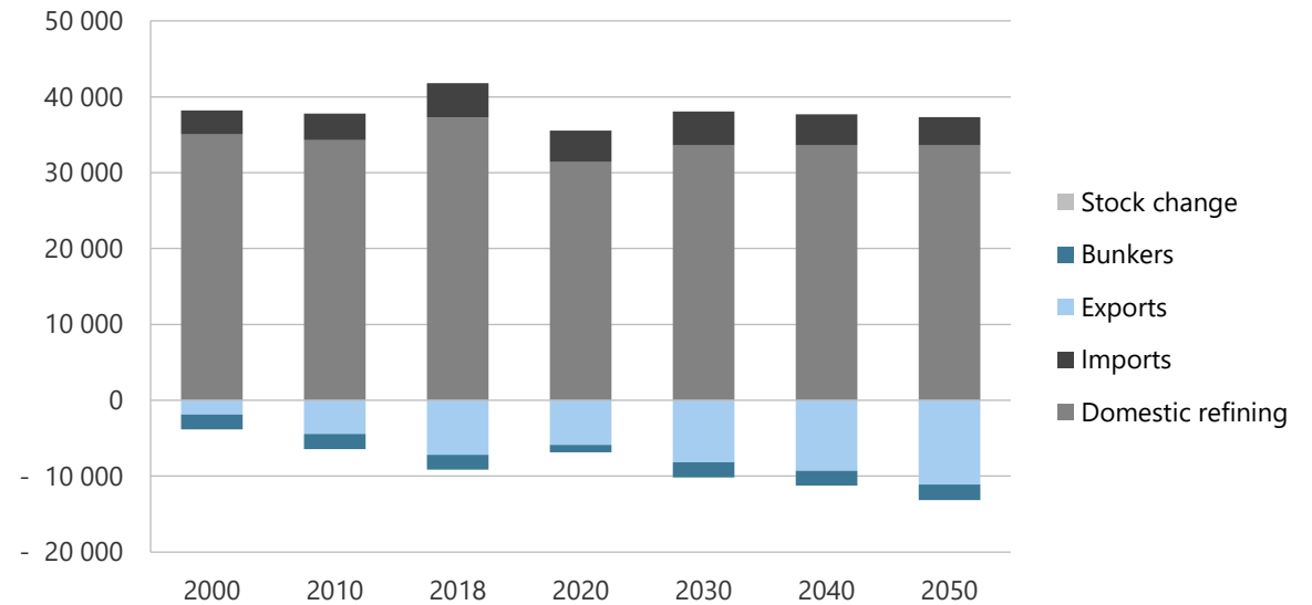
Figure 20-38. Refined products production, imports, and exports in REF, 2000-2050 (PJ).
