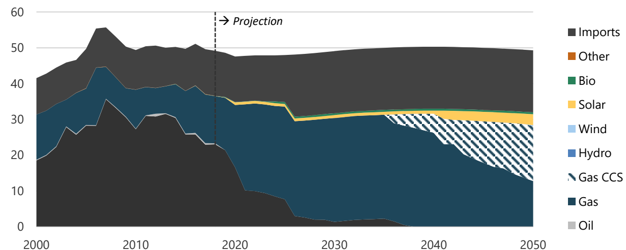
Figure 6-14. Electricity generation in CN, 2000-2050 (TWh).
