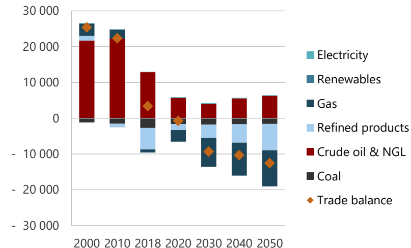
Figure 20-21. Net energy trade in REF, 2000-2050 (PJ).
