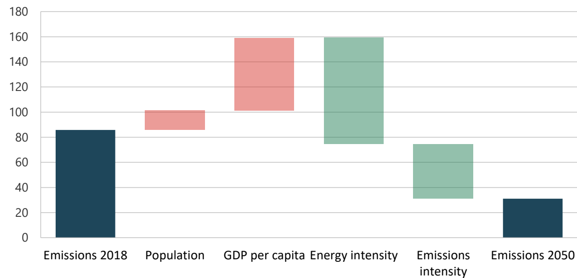
Figure 4-54. CO 2 emissions components in CN, 2018 and 2050 (million tonnes).
