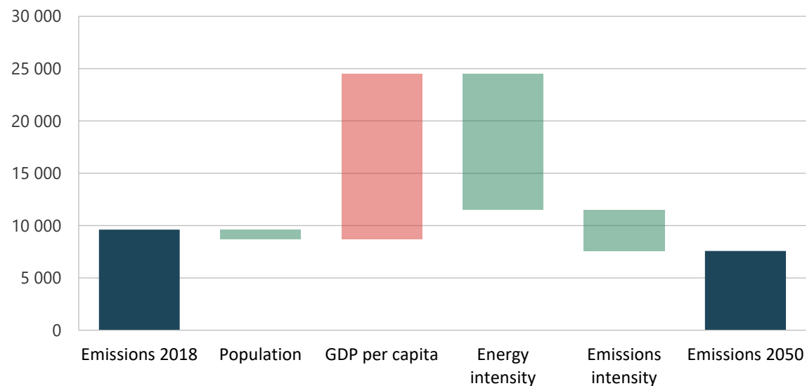
Figure 5-49. CO 2 emissions components in REF, 2018 and 2050 (million tonnes).
