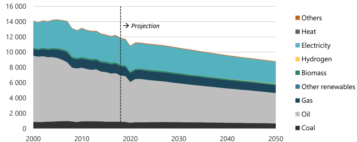
Figure 8-3. Energy demand in REF, 2000-2050 (PJ).
