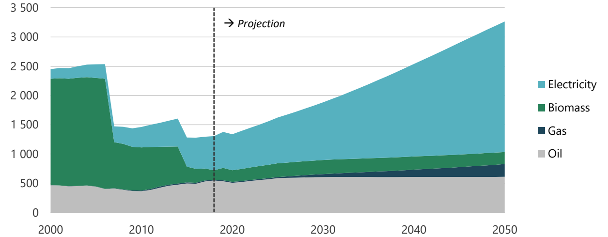
Figure 7-7. Buildings energy demand in REF, 2000-2050 (PJ).
