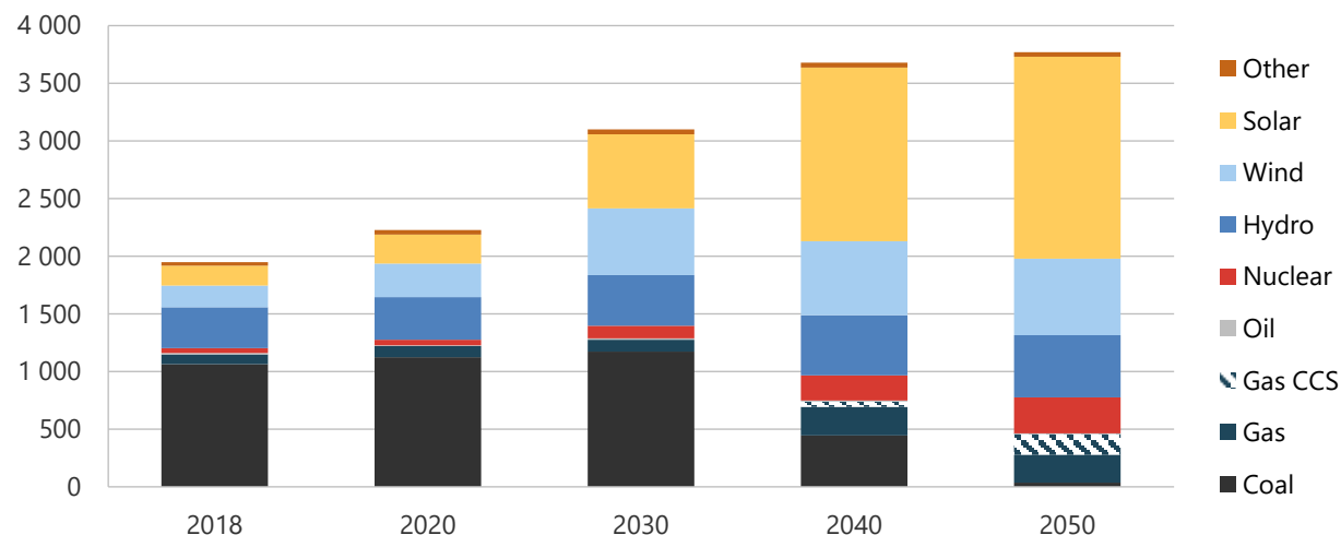
Figure 5-16. Generation capacity in CN, 2018-2050 (GW).
