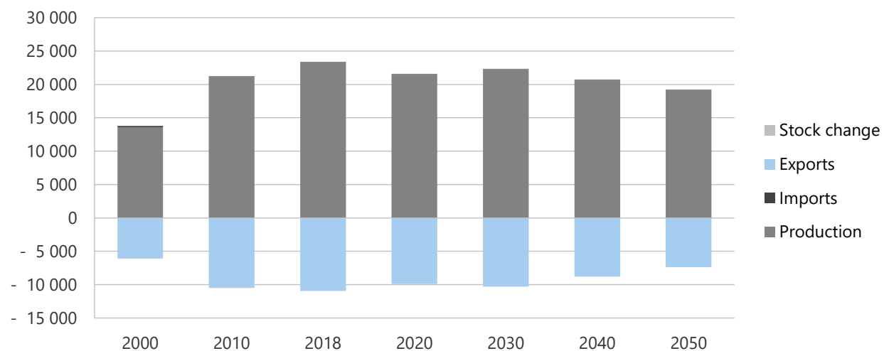
Figure 16-33. Crude oil and NGLs production, imports, and exports in REF, 2000-2050 (PJ).
