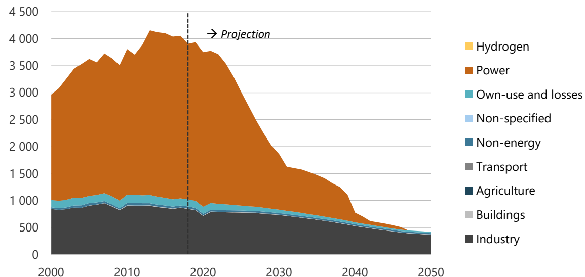
Figure 8-25. Coal consumption by sector in CN, 2000-2050 (PJ).
