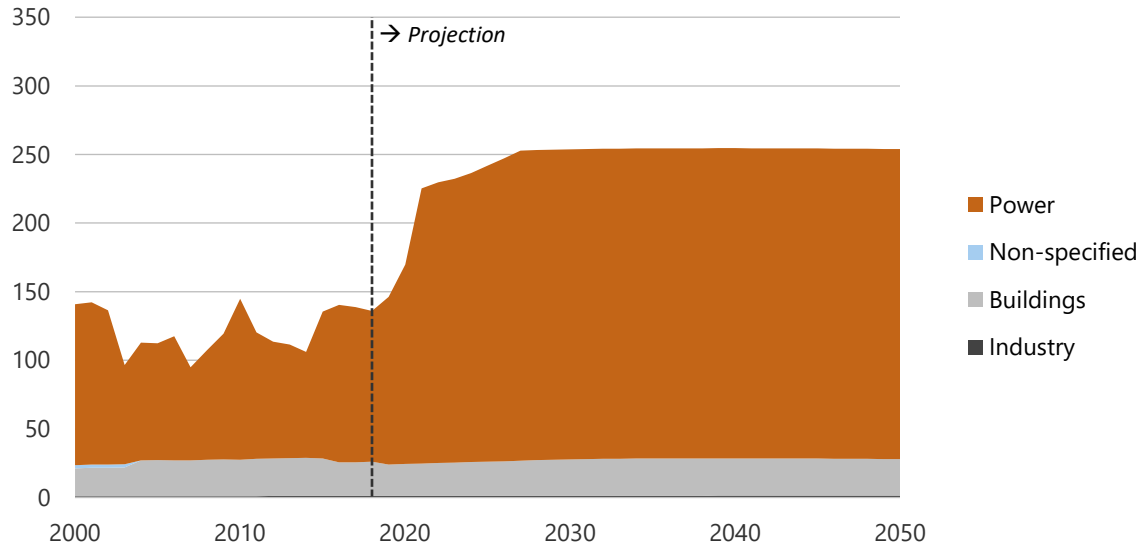
Figure 6-29. Natural gas consumption by sector in REF, 2000-2050 (PJ).
