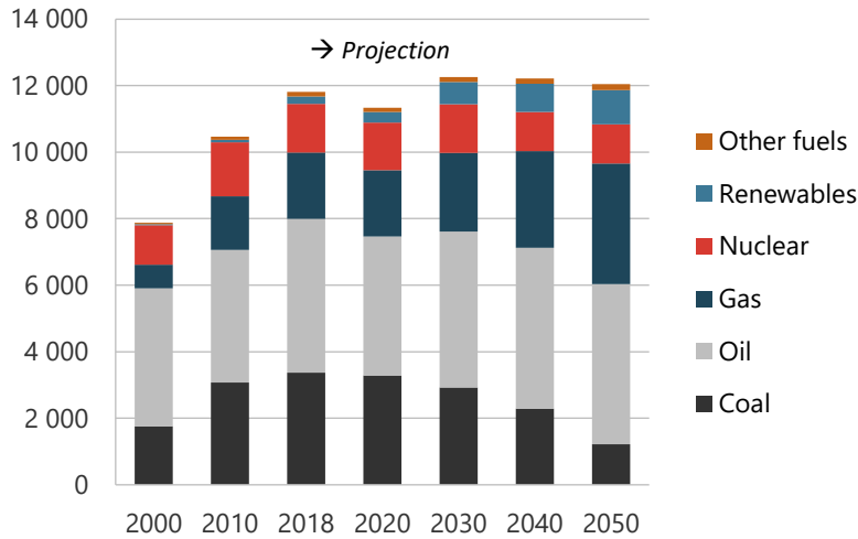
Figure 9-19. Total energy supply in REF, 2000-2050 (PJ).
