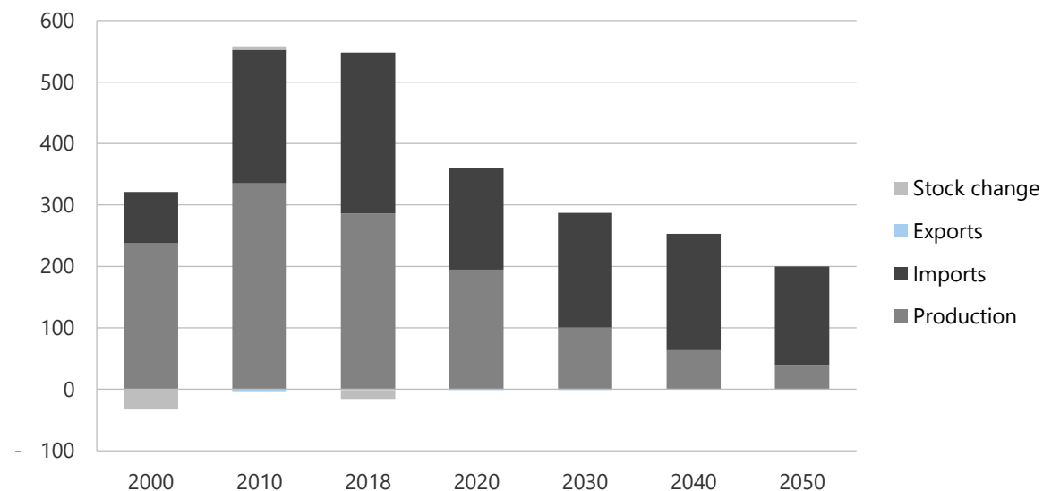
Figure 11-24. Coal production, imports, and exports in REF, 2000-2050 (PJ).
