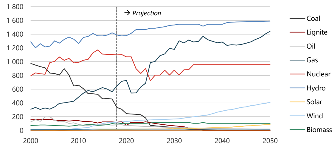
Figure 3-17. Fuel consumption by the power sector in REF, 2000-2050 (PJ).
