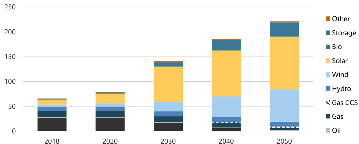
Figure 1-16. Generation capacity in CN, 2018-2050 (GW).
