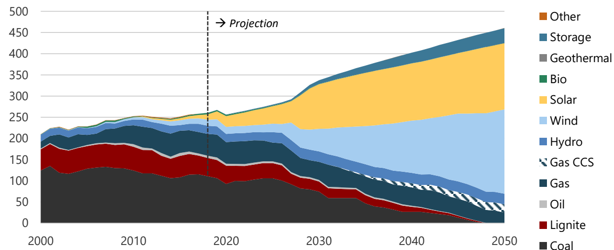
Figure 1-14. Electricity generation in CN, 2000-2050 (TWh).
