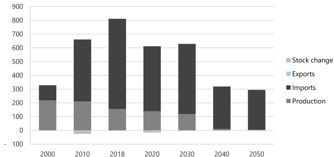
Figure 19-28. Coal production, imports, and exports in CN, 2000-2050 (PJ).
