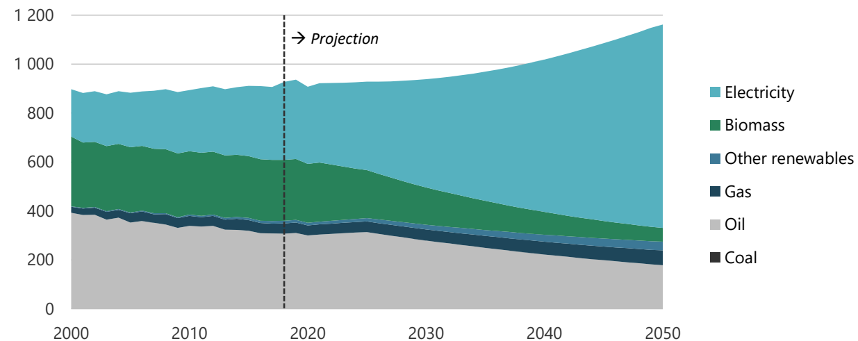
Figure 11-7. Buildings energy demand in REF, 2000-2050 (PJ).
