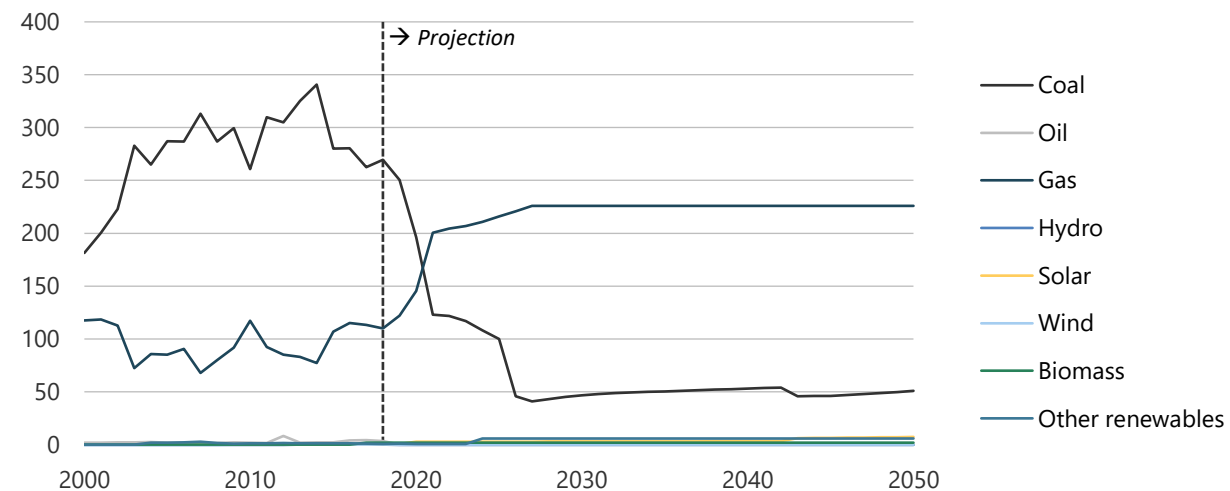
Figure 6-17. Fuel consumption by the power sector in REF, 2000-2050 (PJ).
