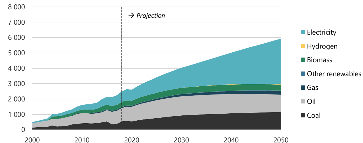
Figure 21-4. Energy demand in CN, 2000-2050 (PJ).
