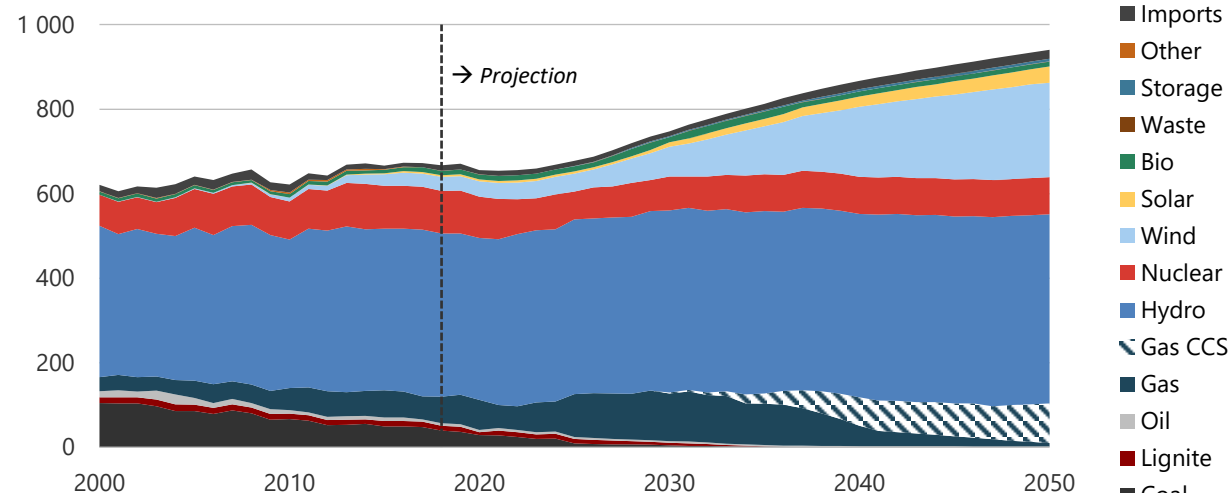
Figure 3-14. Electricity generation in CN, 2000-2050 (TWh).
