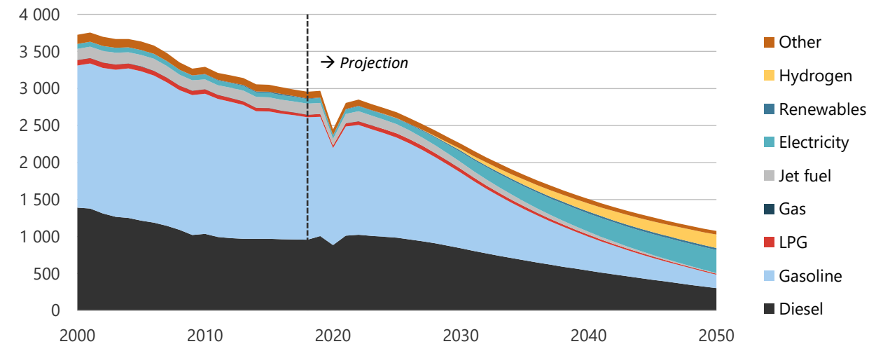
Figure 8-12. Transport energy demand in CN, 2000-2050 (PJ).
