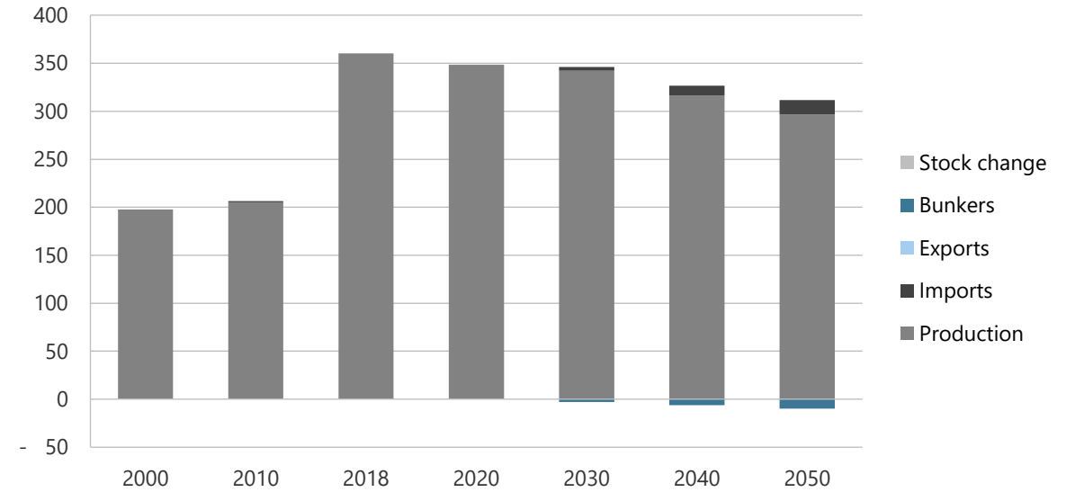
Figure 4-48. Bioenergy production, imports, and exports in CN, 2000-2050 (PJ).
