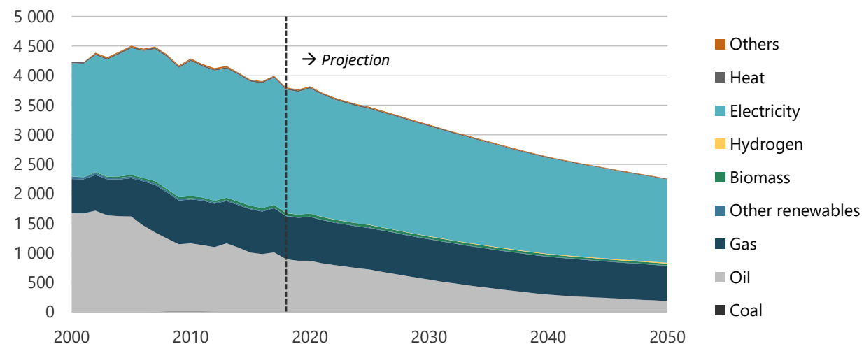
Figure 8-8. Buildings energy demand in CN, 2000-2050 (PJ).
