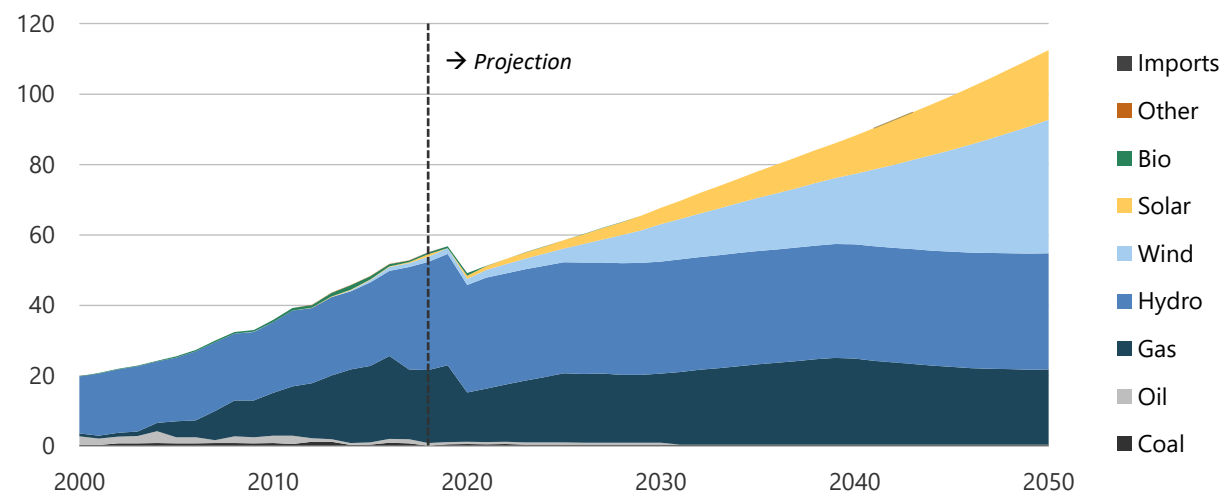
Figure 14-14. Electricity generation in CN, 2000-2050 (TWh).
