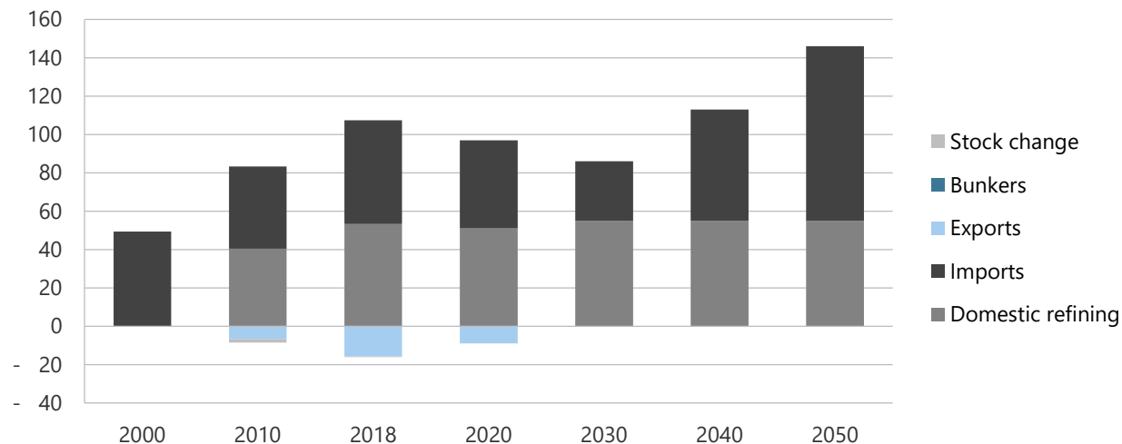
Figure 13-29. Refined product production, imports, and exports in REF, 2000-2050 (PJ).
