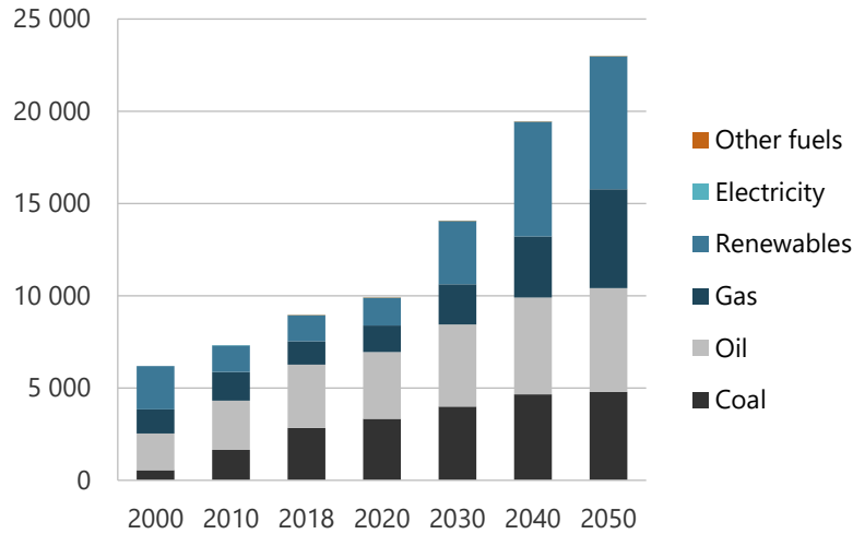
Figure 7-19. Total energy supply in REF, 2000-2050 (PJ).
