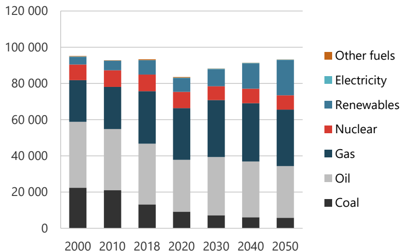
Figure 20-19. Total energy supply in REF, 2000-2050 (PJ).
