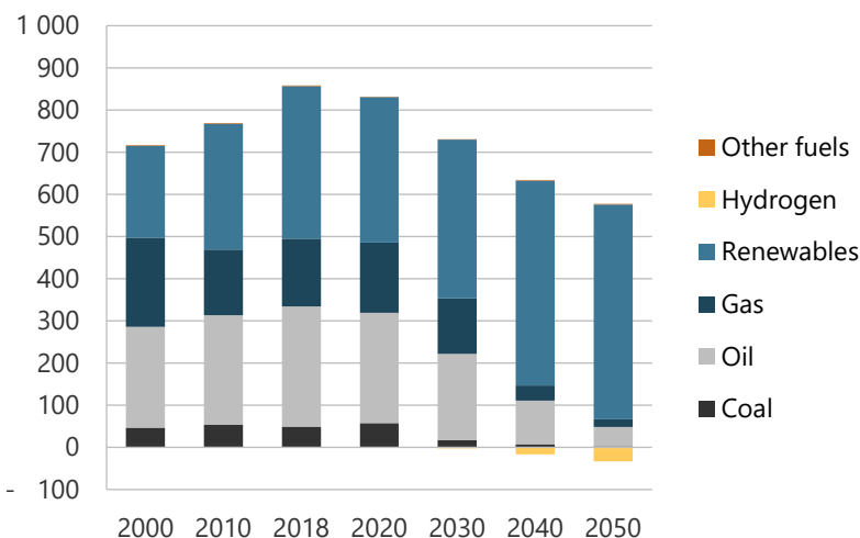
Figure 12-22. Total energy supply in CN, 2000-2050 (PJ).
