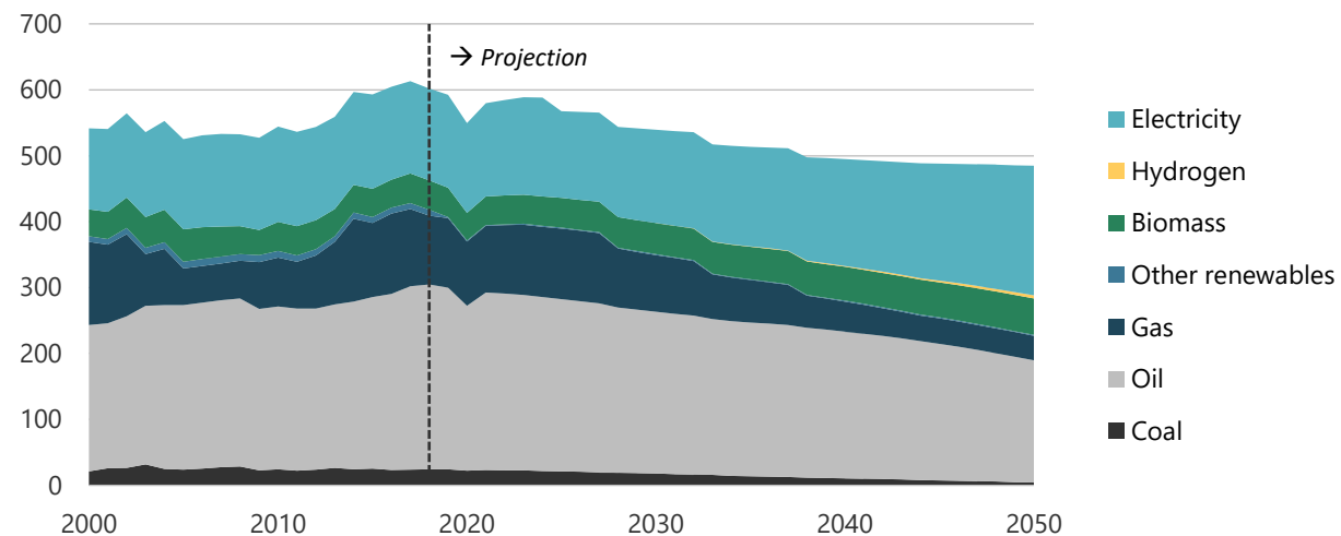
Figure 12-3. Energy demand in REF, 2000-2050 (PJ).
