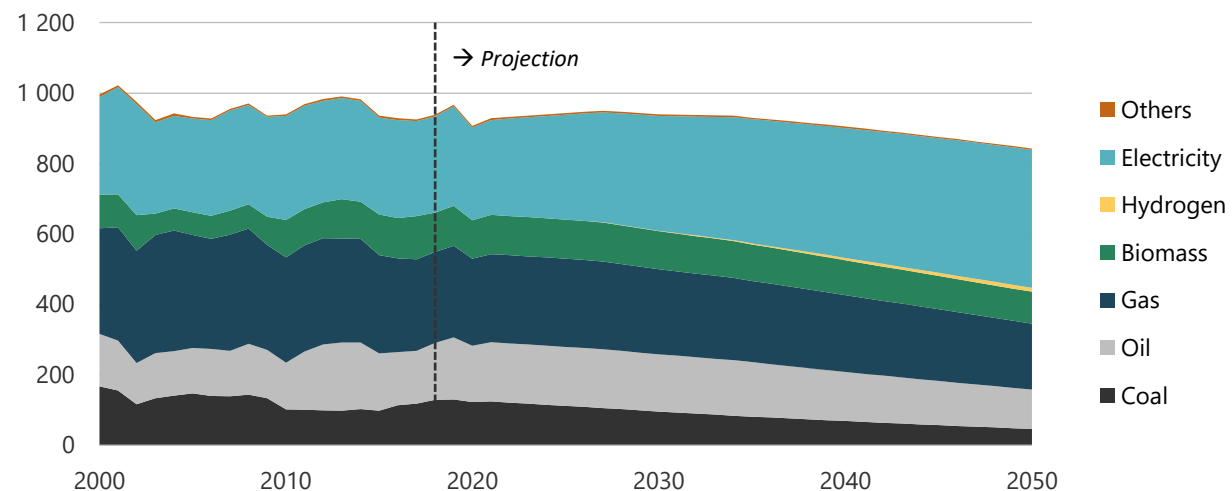
Figure 1-10. Industry energy demand in CN, 2000-2050 (PJ).
