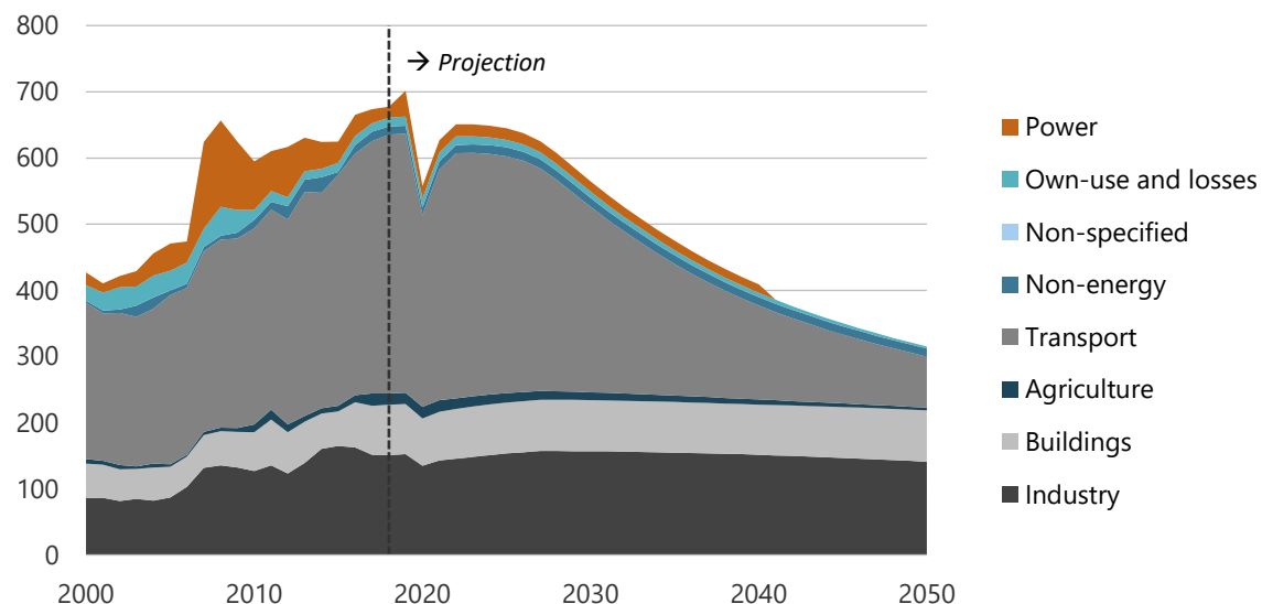
Figure 4-39. Refined products consumption by sector in CN, 2000-2050 (PJ).
