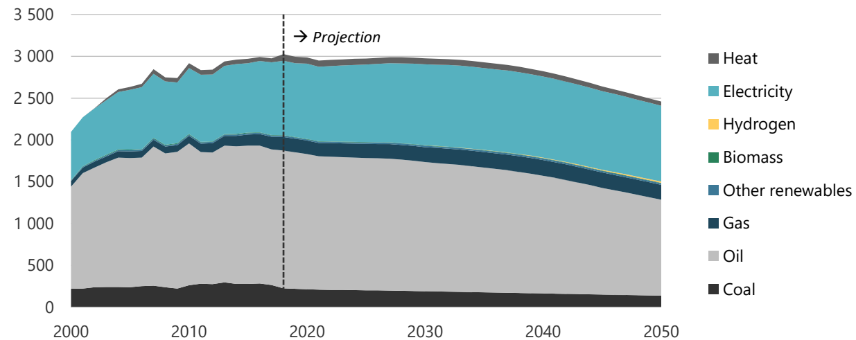
Figure 18-3. Energy demand in REF, 2000-2050 (PJ).
