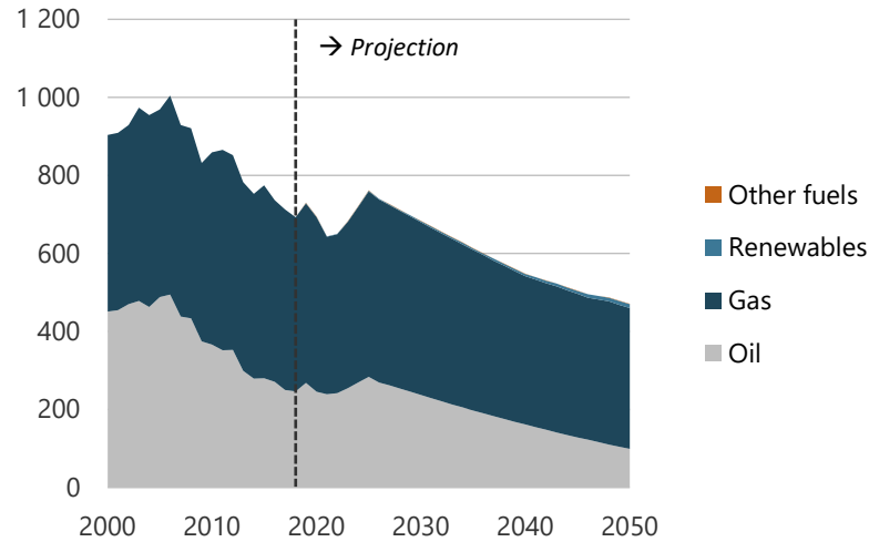
Figure 2-23. Energy production in CN, 2000-2050 (PJ).
