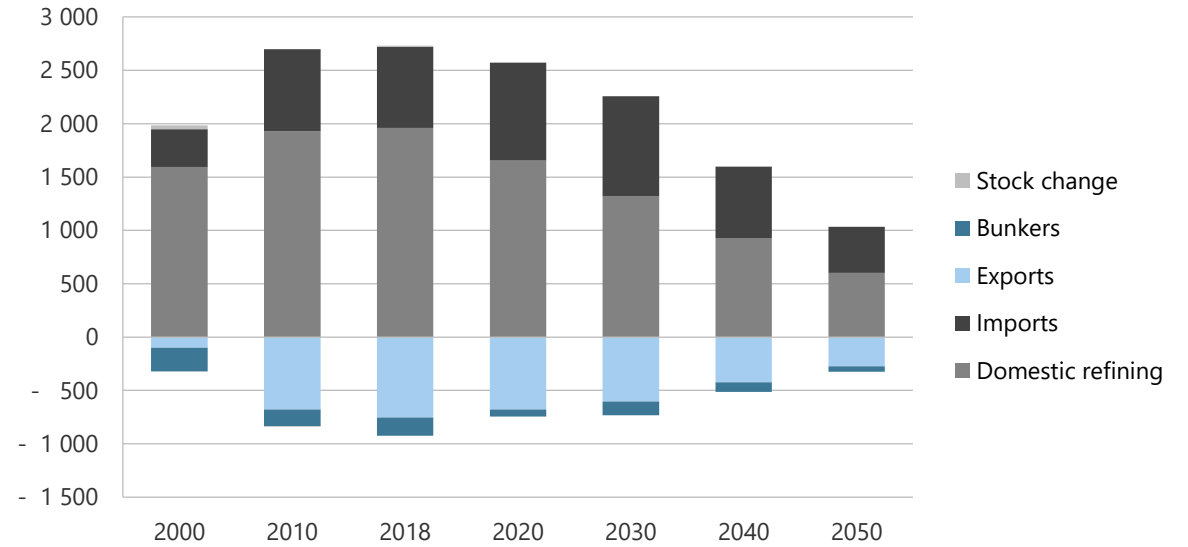
Figure 18-40. Refined products production, imports, and exports in CN, 2000-2050 (PJ).
