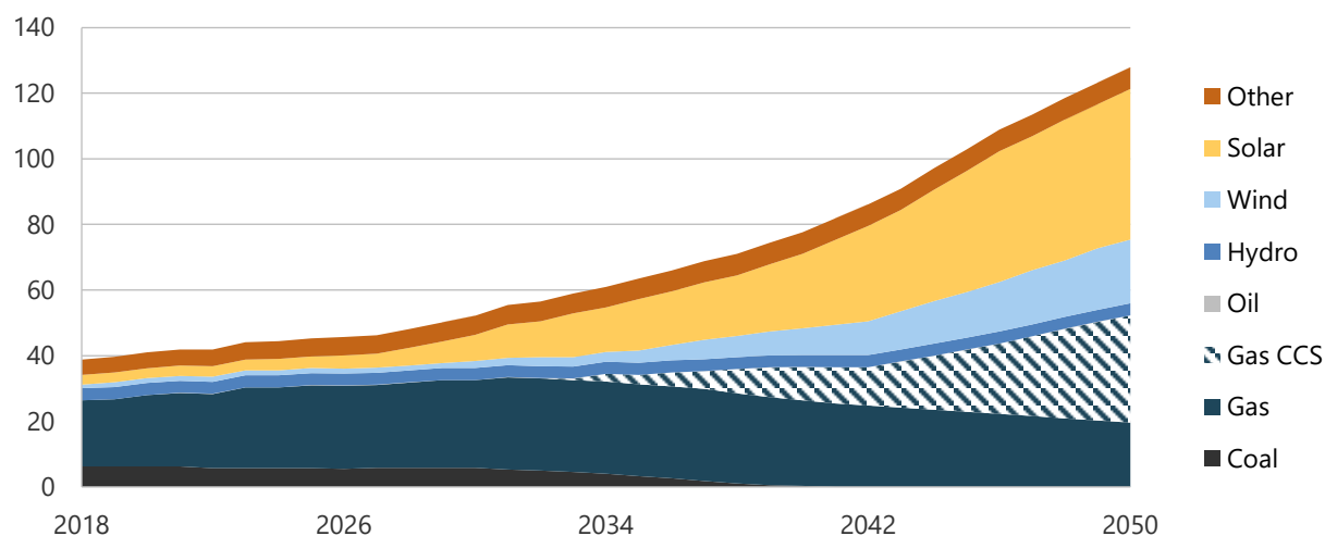
Figure 19-16. Generation capacity in CN, 2018-2050 (GW).
