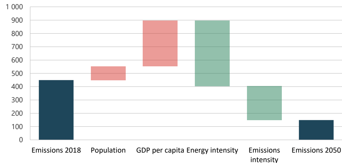
Figure 11-52. CO 2 emissions components in CN, 2018 and 2050 (million tonnes).
