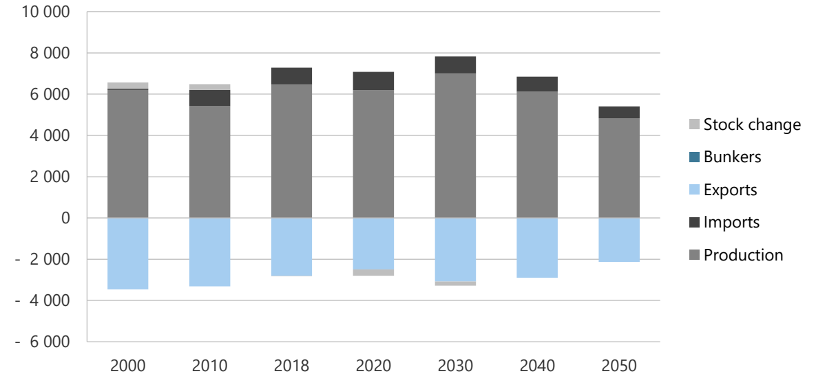
Figure 3-32. Natural gas production, imports, and exports in CN, 2000-2050 (PJ).
