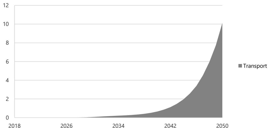
Figure 15-41. Hydrogen consumption by sector in REF, 2000-2050 (PJ).
