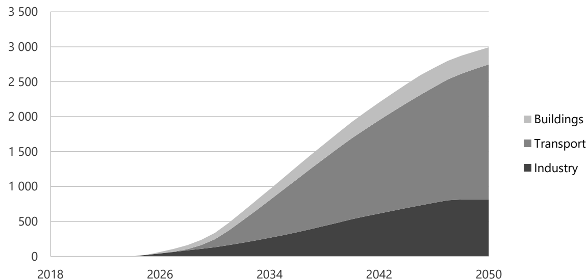
Figure 20-43. Hydrogen consumption by sector in CN, 2000-2050 (PJ).
