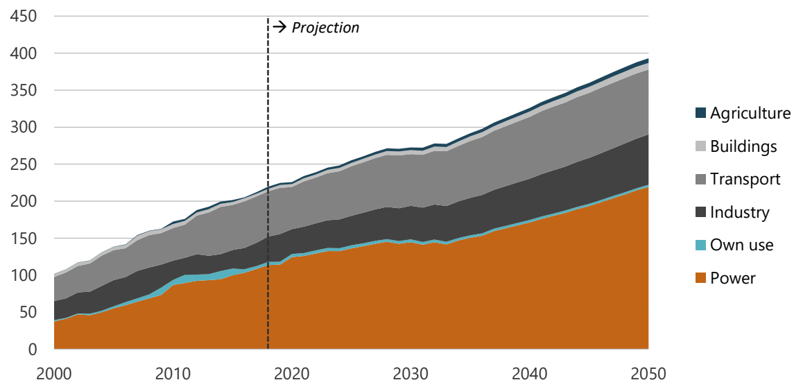
Figure 10-51. Gross CO 2 emissions in REF, 2000-2050 (million tonnes).
