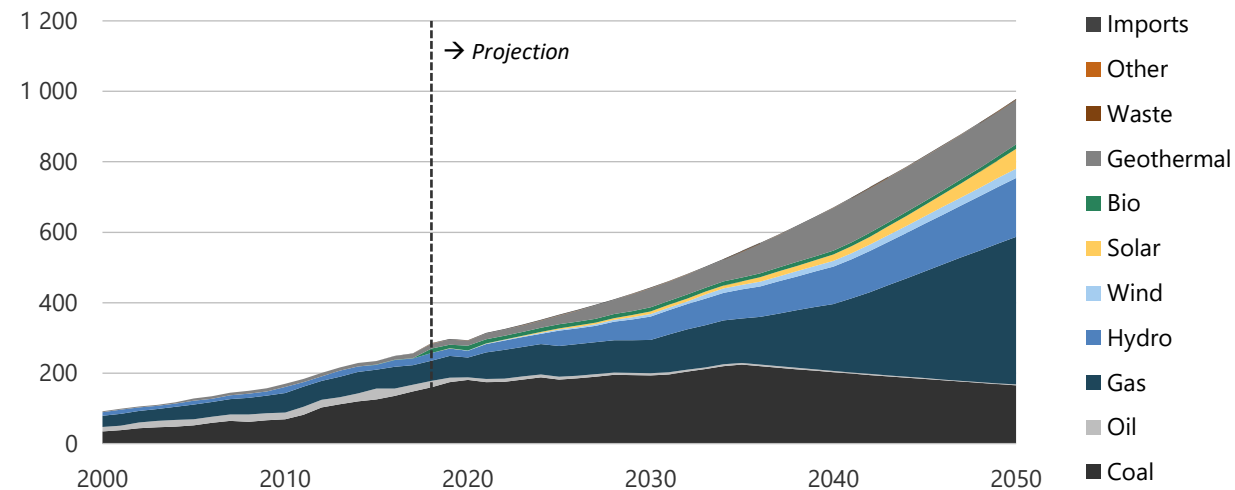
Figure 7-13. Electricity generation in REF, 2000-2050 (TWh).
