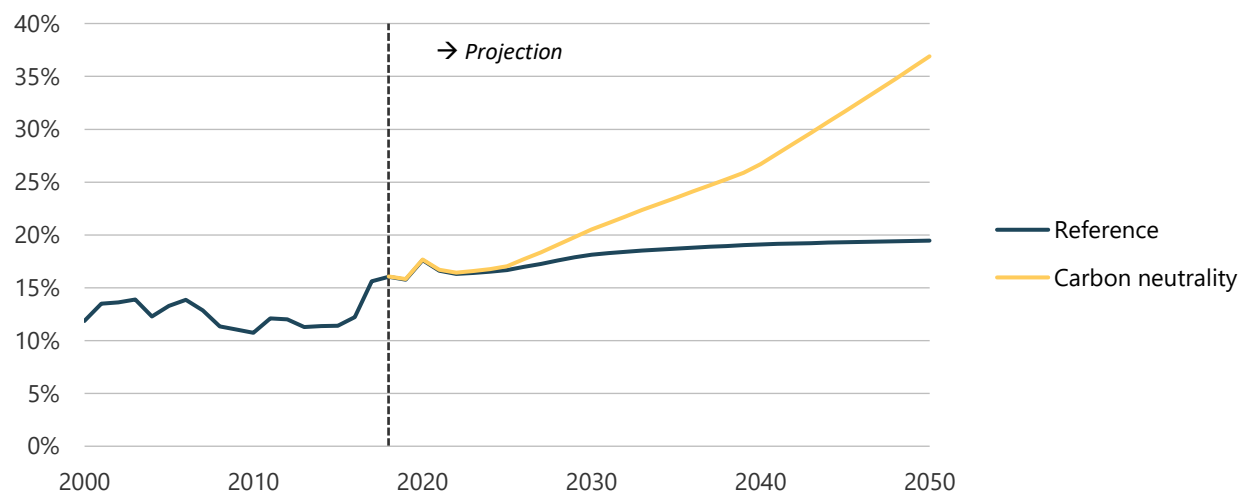
Figure 14-46. Modern renewables share in REF and CN, 2000-2050.
