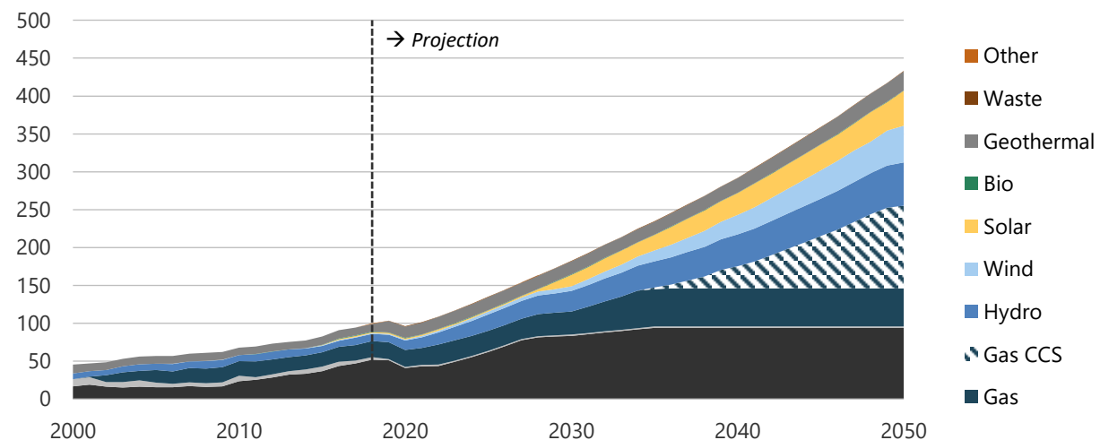
Figure 15-14. Electricity generation in CN, 2000-2050 (TWh).
