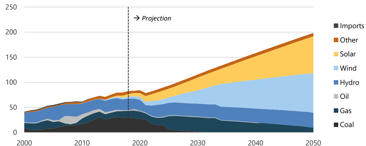
Figure 4-14. Electricity generation in CN, 2000-2050 (TWh).
