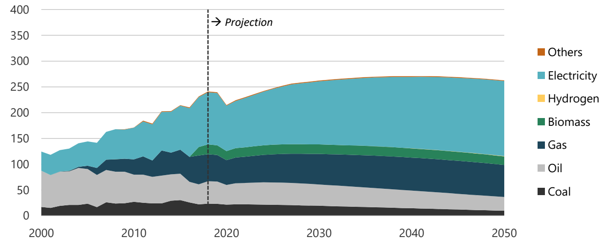
Figure 14-10. Industry energy demand in CN, 2000-2050 (PJ).
