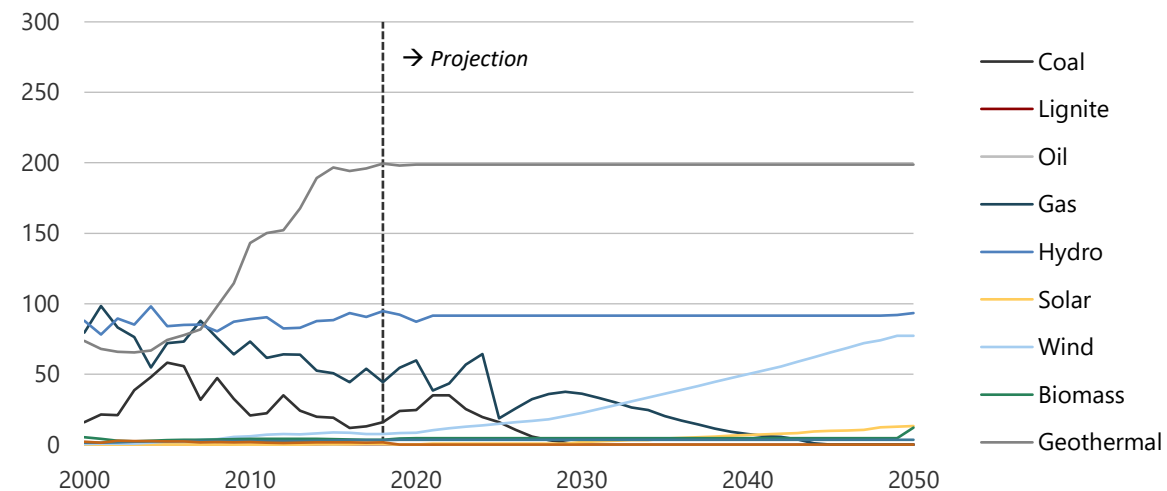
Figure 12-17. Fuel consumption by the power sector in REF, 2000-2050 (PJ).
