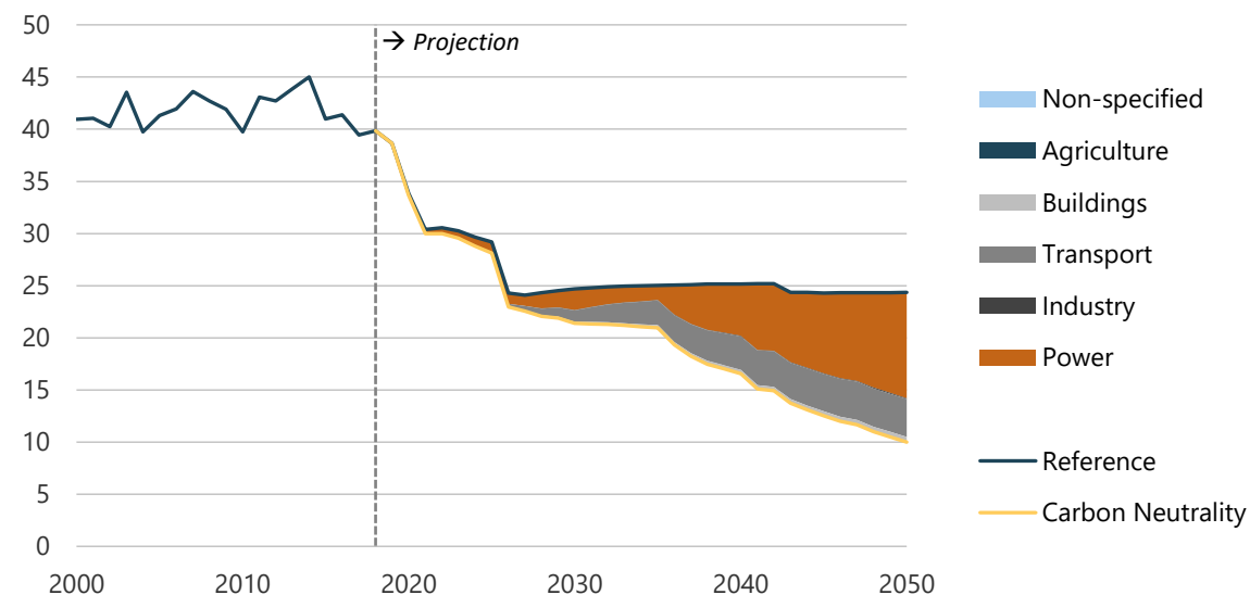
Figure 6-52. Change in gross CO 2 emissions, 2000-2050 (million tonnes).
