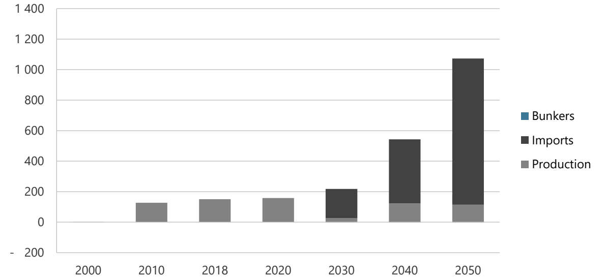
Figure 15-32. Natural gas production, imports, and exports in CN, 2000-2050 (PJ).
