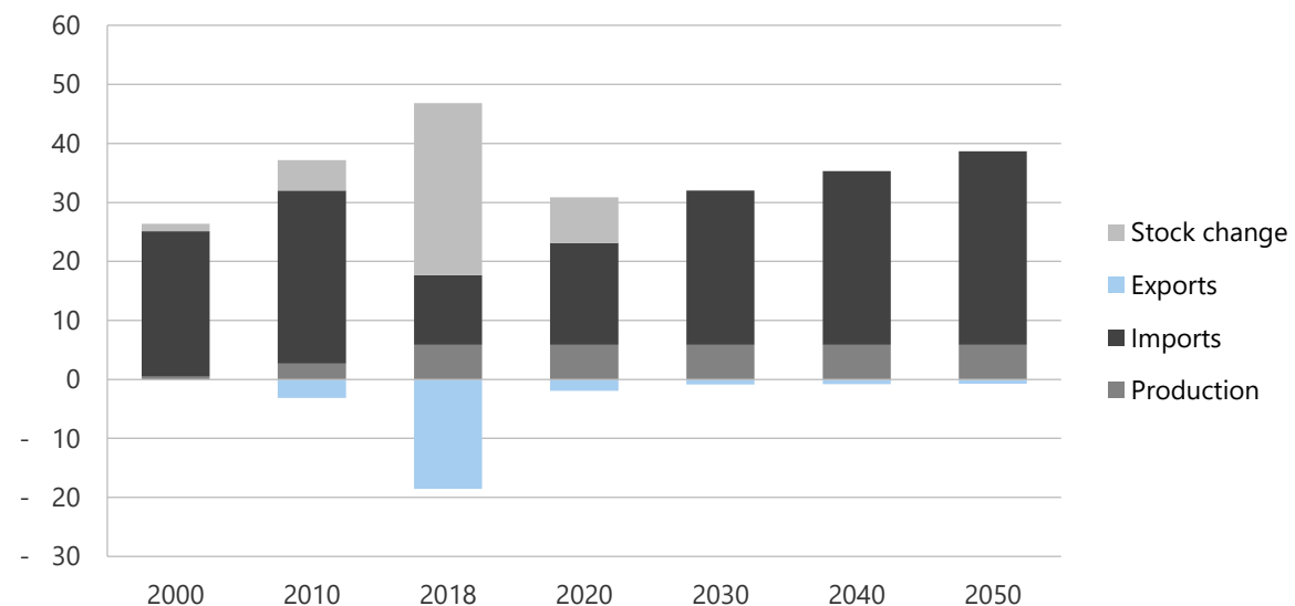
Figure 14-24. Coal production, imports, and exports in REF, 2000-2050 (PJ).
