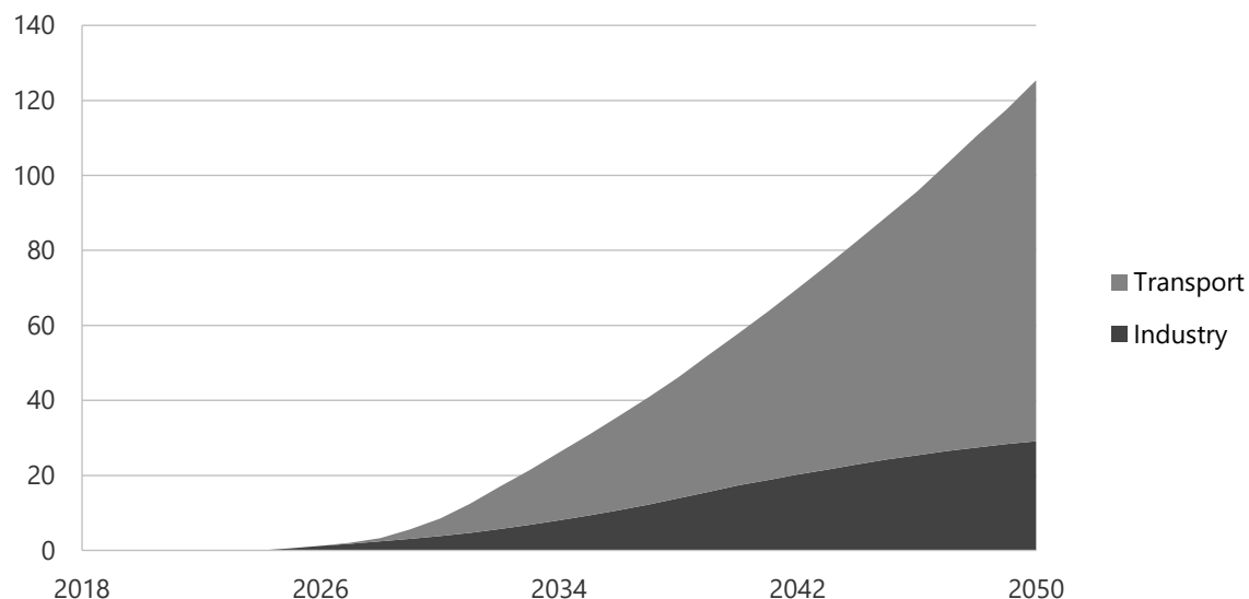
Figure 19-43. Hydrogen consumption by sector in CN, 2000-2050 (PJ).
