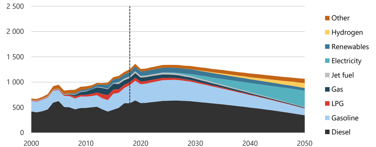
Figure 19-12. Transport energy demand in CN, 2000-2050 (PJ).
