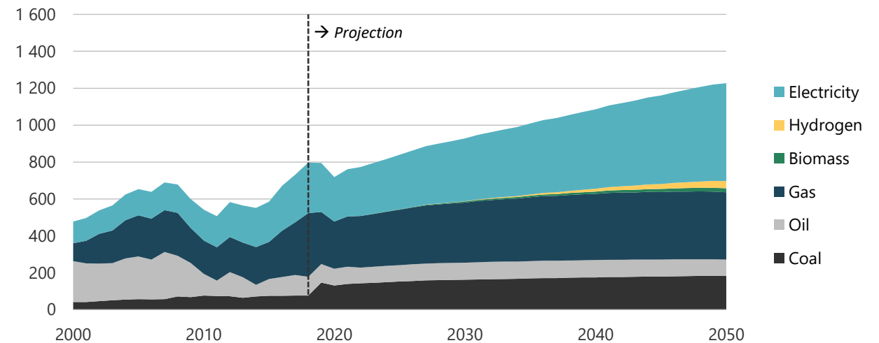
Figure 10-10. Industry energy demand in CN, 2000-2050 (PJ).
