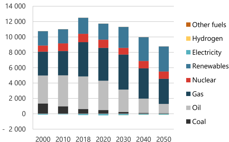
Figure 3-22. Total energy supply in CN, 2000-2050 (PJ).
