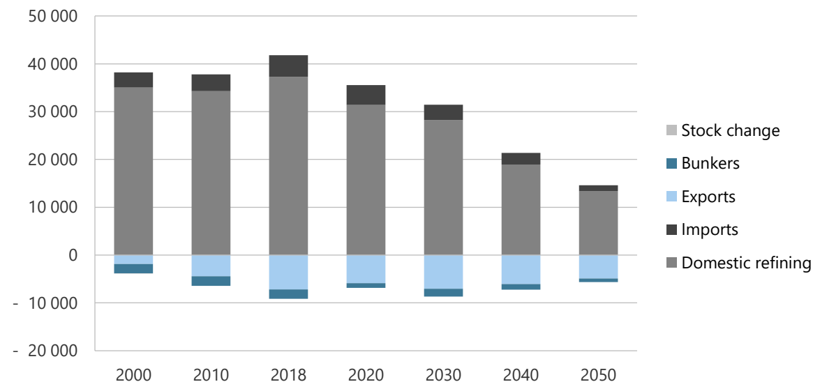
Figure 20-40. Refined products production, imports, and exports in CN, 2000-2050 (PJ).
