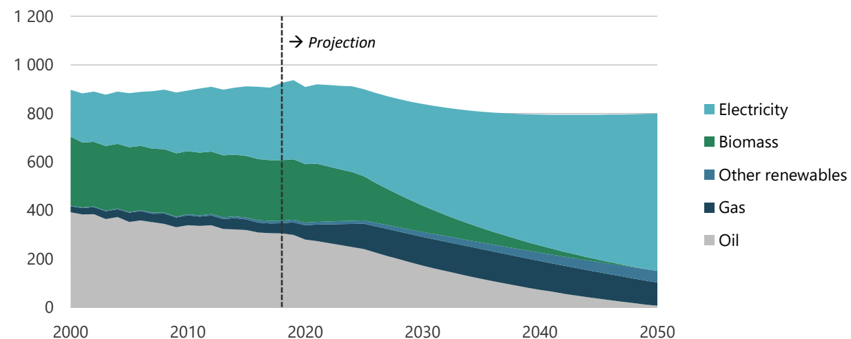
Figure 11-8. Buildings energy demand in CN, 2000-2050 (PJ).
