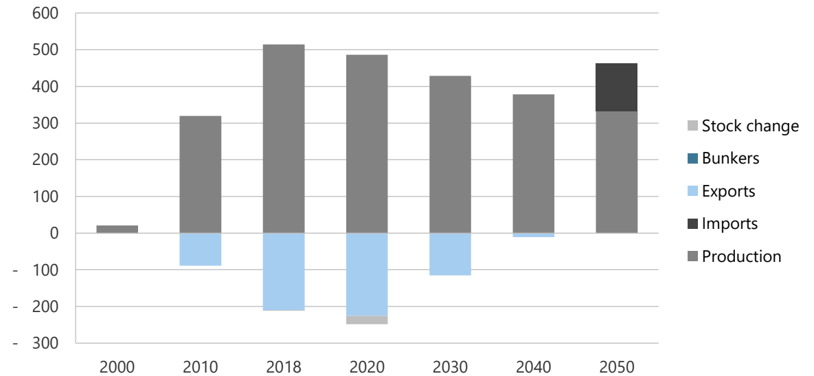
Figure 14-28. Natural gas production, imports, and exports in REF, 2000-2050 (PJ).
