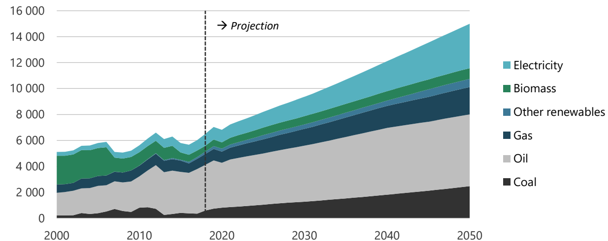
Figure 7-3. Energy demand in REF, 2000-2050 (PJ).
