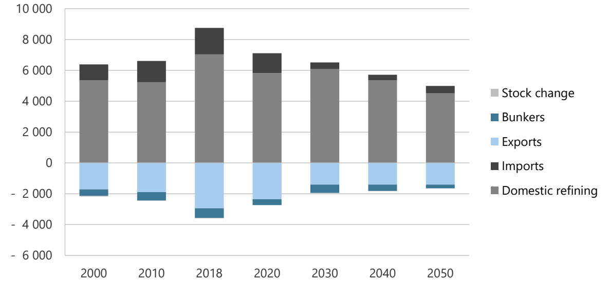
Figure 9-40. Refined products production, imports, and exports in CN, 2000-2050 (PJ).
