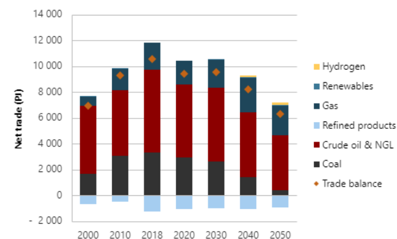
Figure 9-24. Energy trade in CN, 2000-2050 (PJ).
