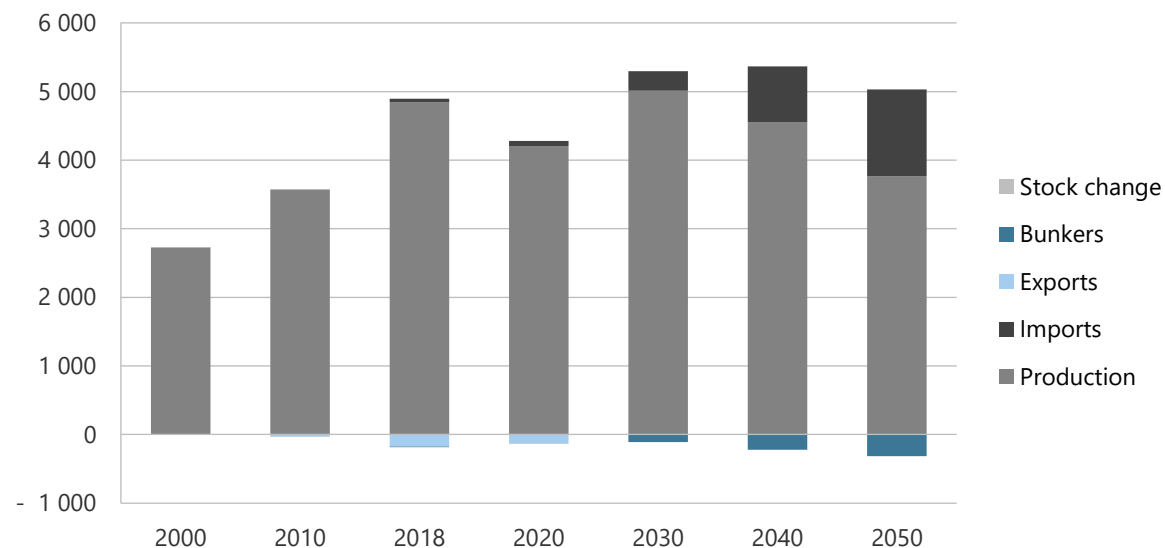
Figure 20-48. Bioenergy production, imports, and exports in CN, 2000-2050 (PJ).
