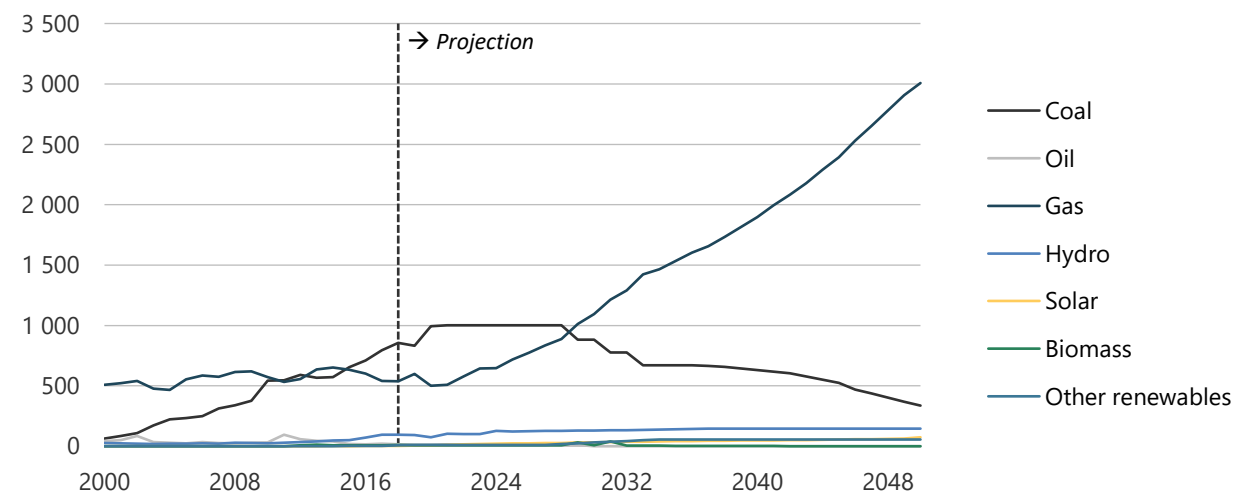
Figure 10-18. Fuel consumption by the power sector in CN, 2000-2050 (PJ).
