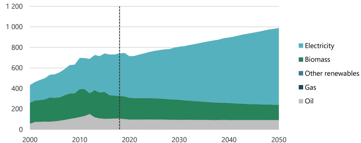
Figure 19-7. Buildings energy demand in REF, 2000-2050 (PJ).
