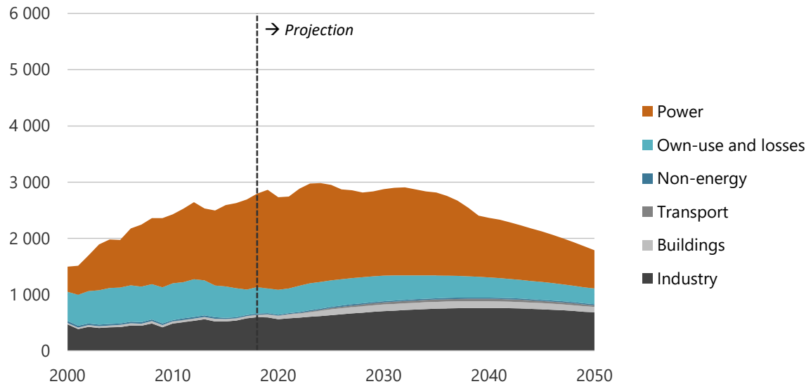
Figure 11-29. Natural gas consumption by sector in CN, 2000-2050 (PJ).
