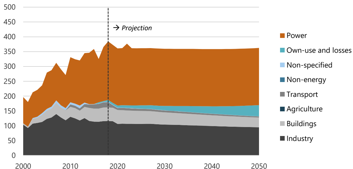
Figure 8-41. Bioenergy consumption by sector in REF, 2000-2050 (PJ).
