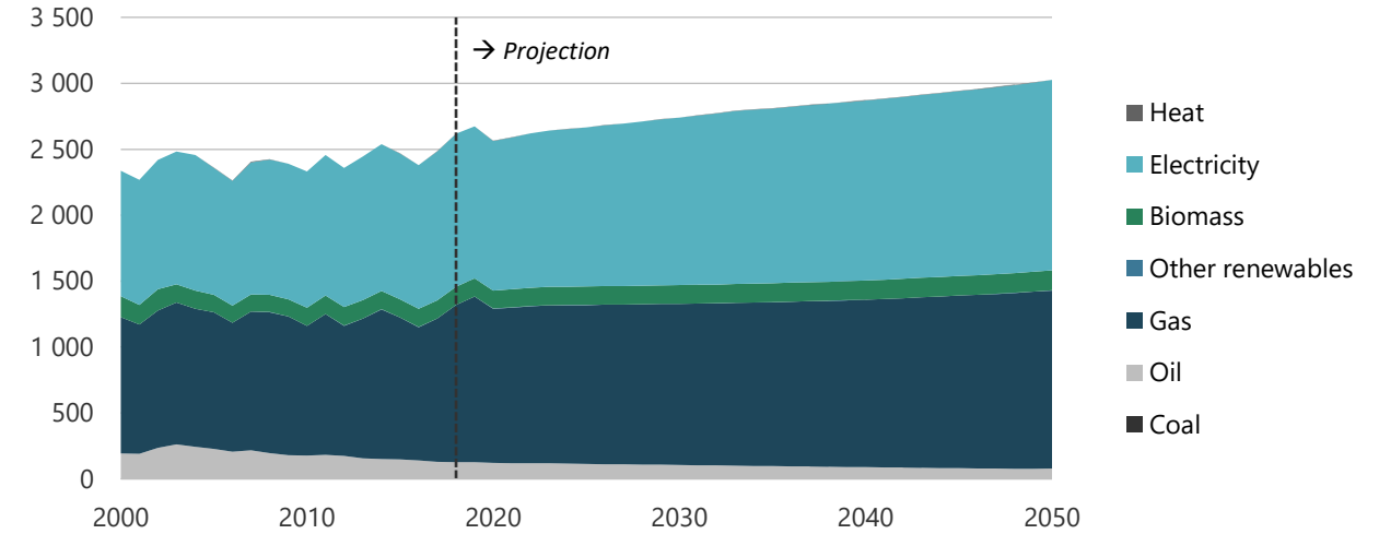
Figure 3-7. Buildings energy demand in REF, 2000-2050 (PJ).
