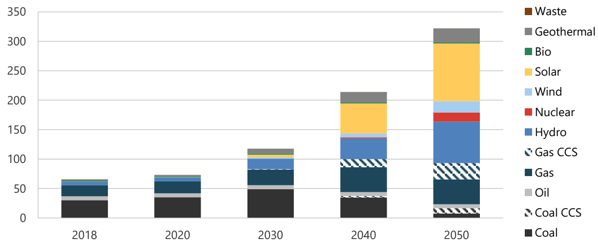
Figure 7-16. Generation capacity in CN, 2018-2050 (GW).
