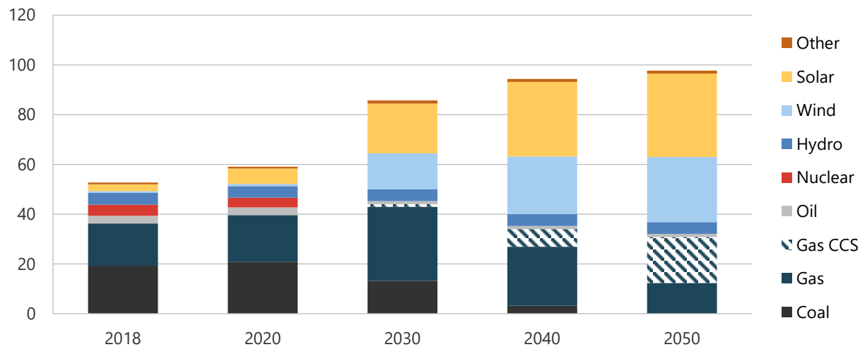
Figure 18-16. Generation capacity in CN, 2018-2050 (GW).
