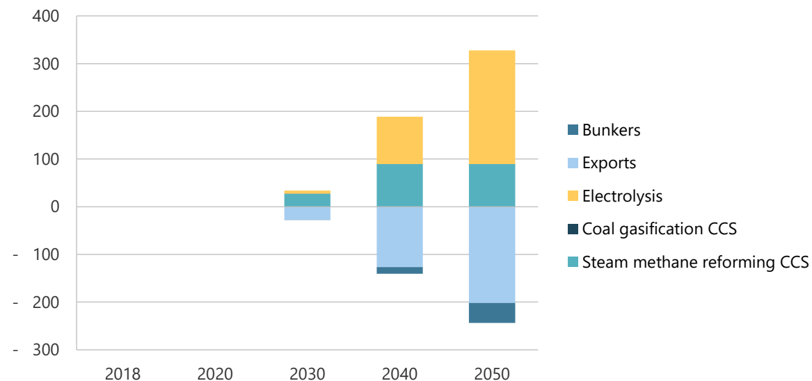
Figure 1-44. Hydrogen production, imports, and exports in CN, 2000-2050 (PJ).
