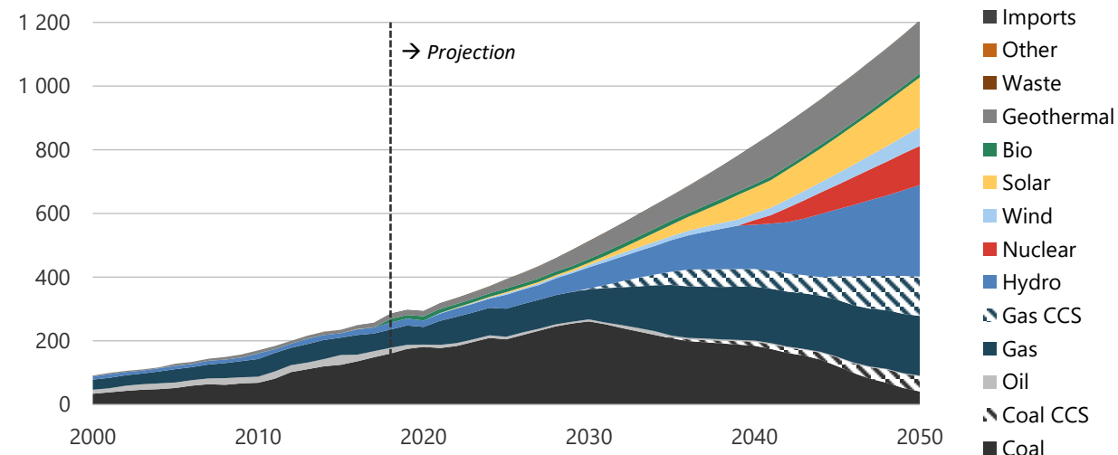
Figure 7-14. Electricity generation in CN, 2000-2050 (TWh).
