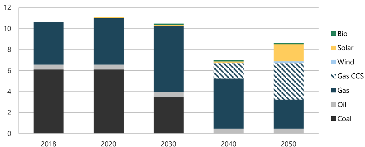
Figure 6-16. Generation capacity in CN, 2018-2050 (GW).
