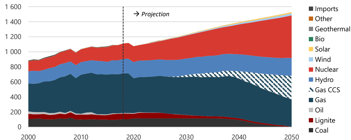
Figure 16-14. Electricity generation in CN, 2000-2050 (TWh).
