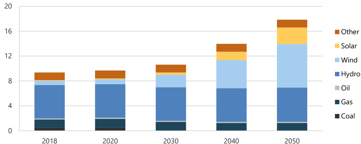
Figure 12-15. Technology capacity in REF, 2017-2050 (GW).
