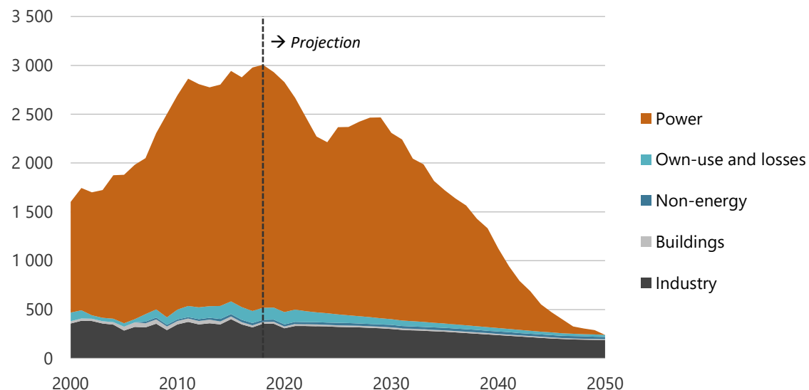
Figure 9-27. Coal consumption by sector in CN, 2000-2050 (PJ).
