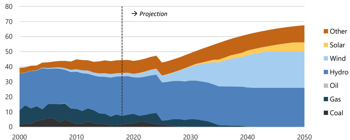
Figure 12-14. Electricity generation in CN, 2000-2050 (TWh).
