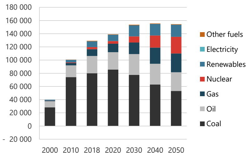
Figure 5-17. Total energy supply in REF, 2000-2050 (PJ).
