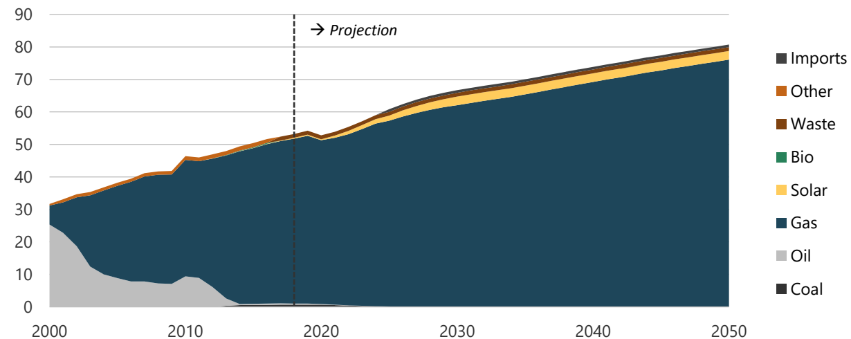
Figure 17-13. Electricity generation in REF, 2000-2050 (TWh).
