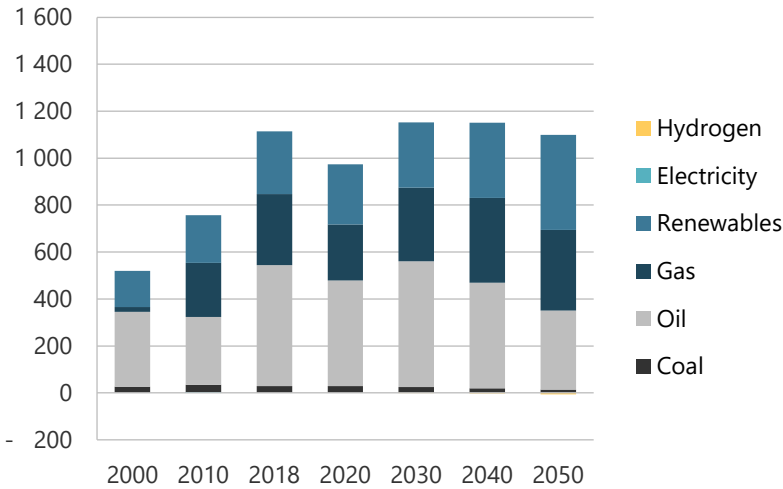
Figure 14-20. Total energy supply in CN, 2000-2050 (PJ).
