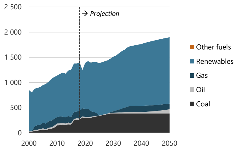
Figure 15-20. Energy production in REF, 2000-2050 (PJ).
