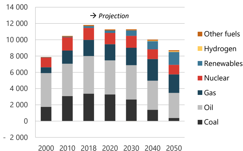
Figure 9-22. Total energy supply in CN, 2000-2050 (PJ).
