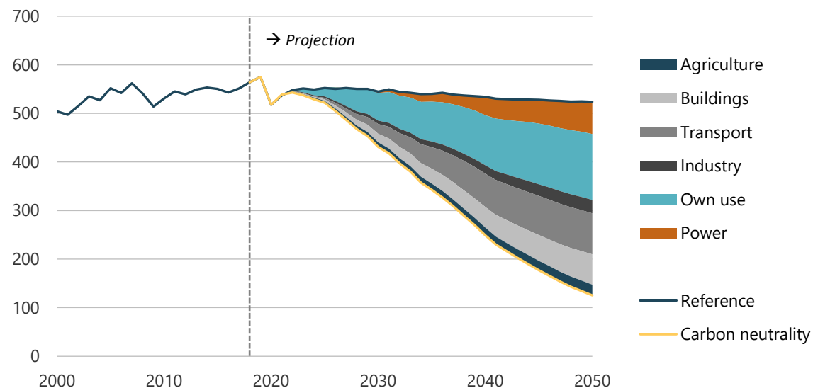
Figure 3-52. Change in gross CO 2 emissions, 2000-2050 (million tonnes).
