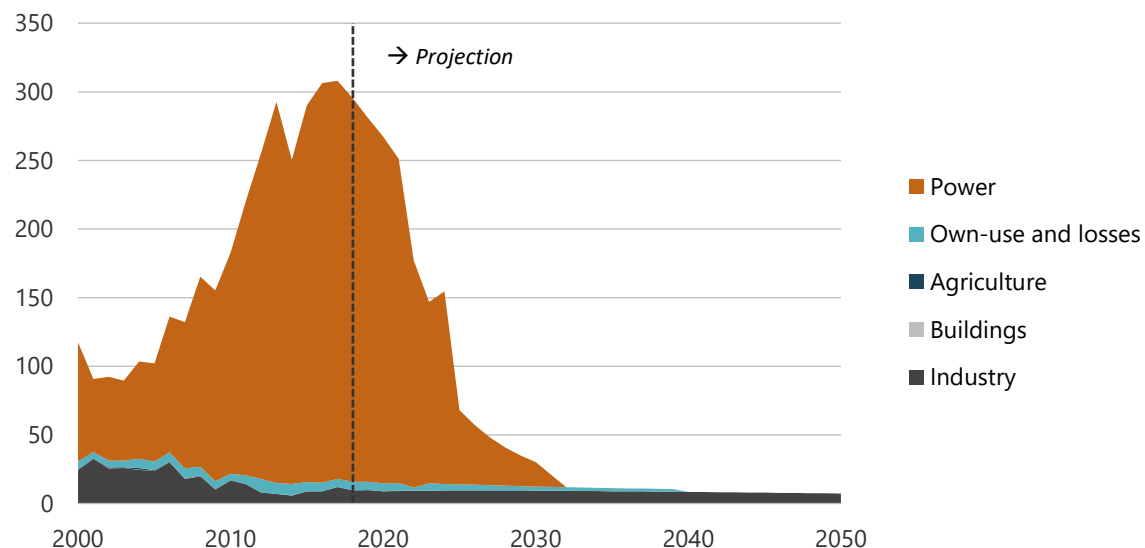
Figure 4-27. Coal consumption by sector in CN, 2000-2050 (PJ).
