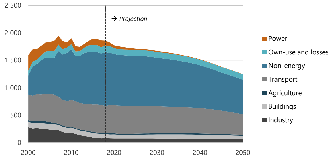
Figure 18-37. Refined products consumption by sector in REF, 2000-2050 (PJ).
