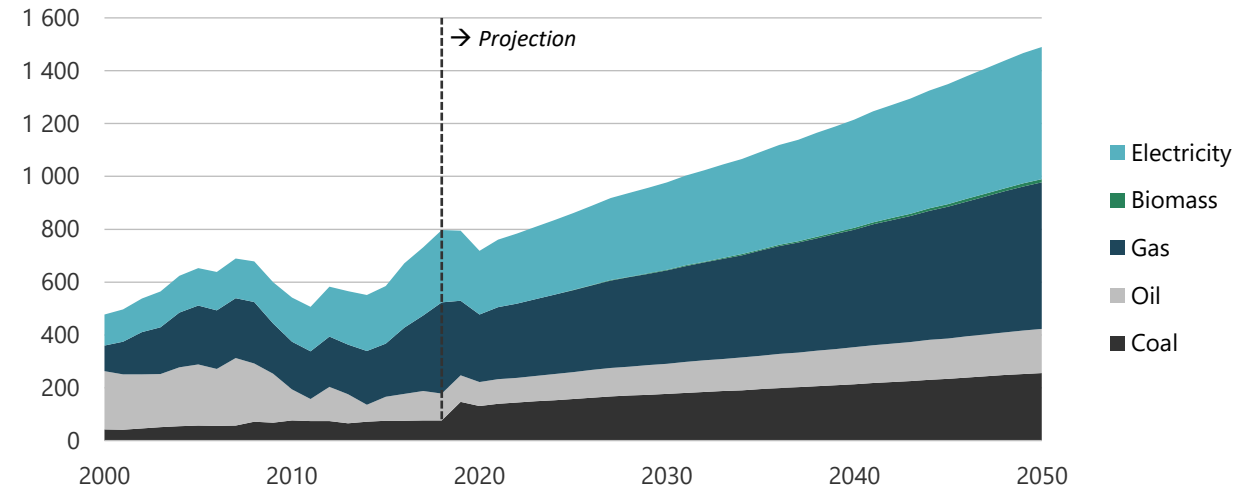
Figure 10-9. Industry energy demand in REF, 2000-2050 (PJ).
