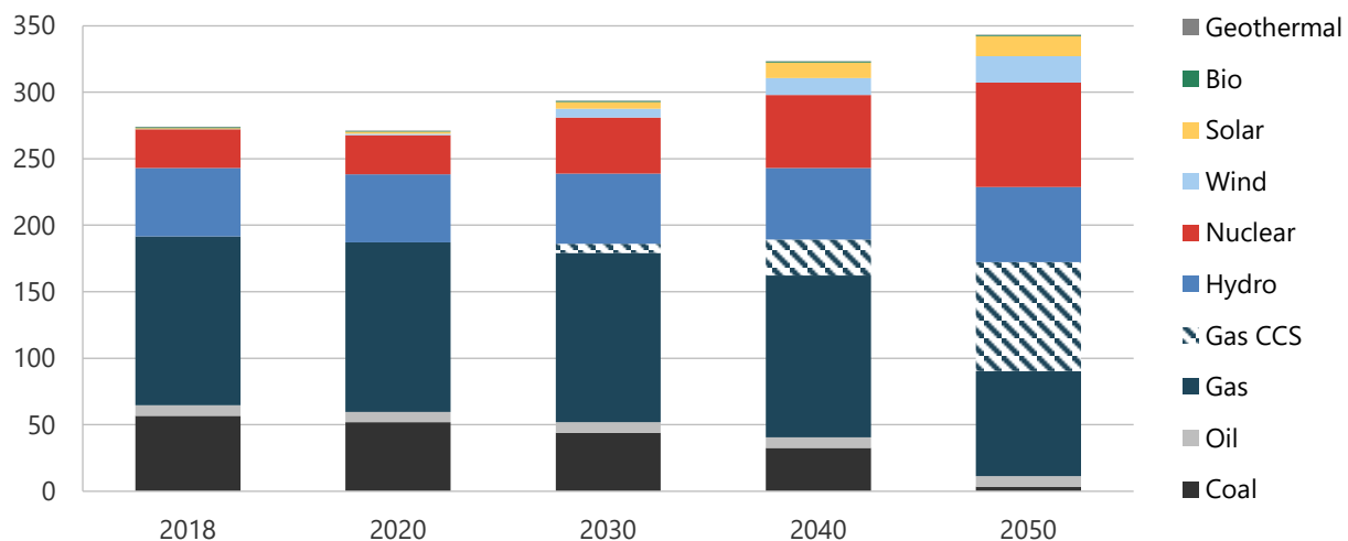
Figure 16-18. Generation capacity in CN, 2018-2050 (GW).
