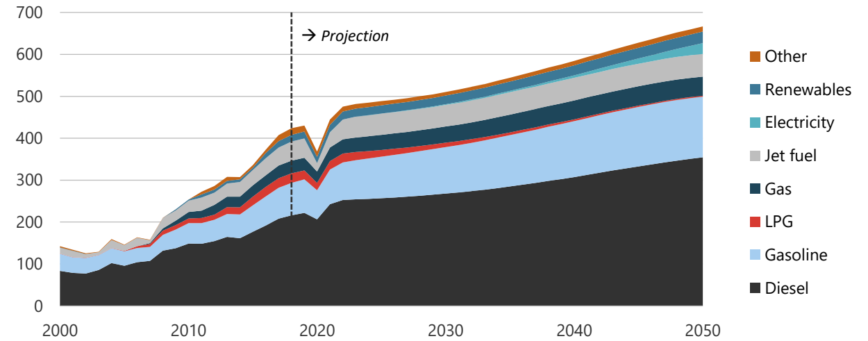
Figure 14-11. Transport energy demand in REF, 2000-2050 (PJ).
