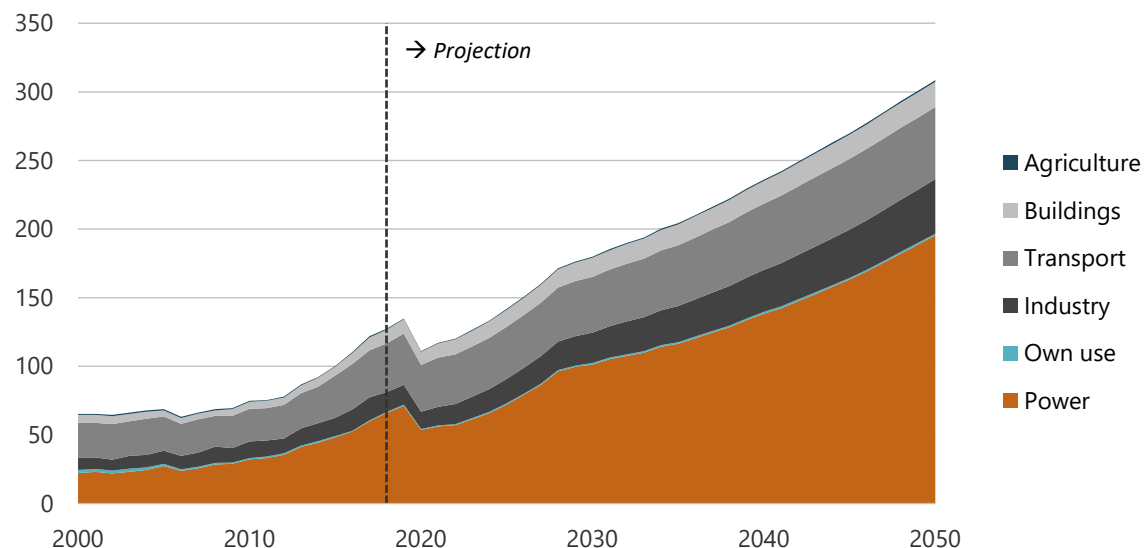
Figure 15-51. Gross CO 2 emissions in REF, 2000-2050 (million tonnes).
