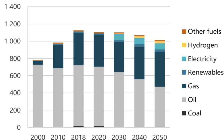
Figure 17-22. Total energy supply in CN, 2000-2050 (PJ).
