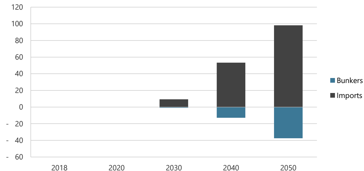
Figure 18-44. Hydrogen production, imports, and exports in CN, 2000-2050 (PJ).
