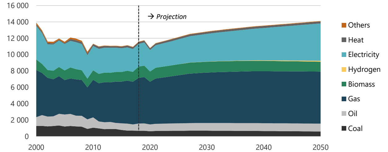
Figure 20-9. Industry energy demand in REF, 2000-2050 (PJ).
