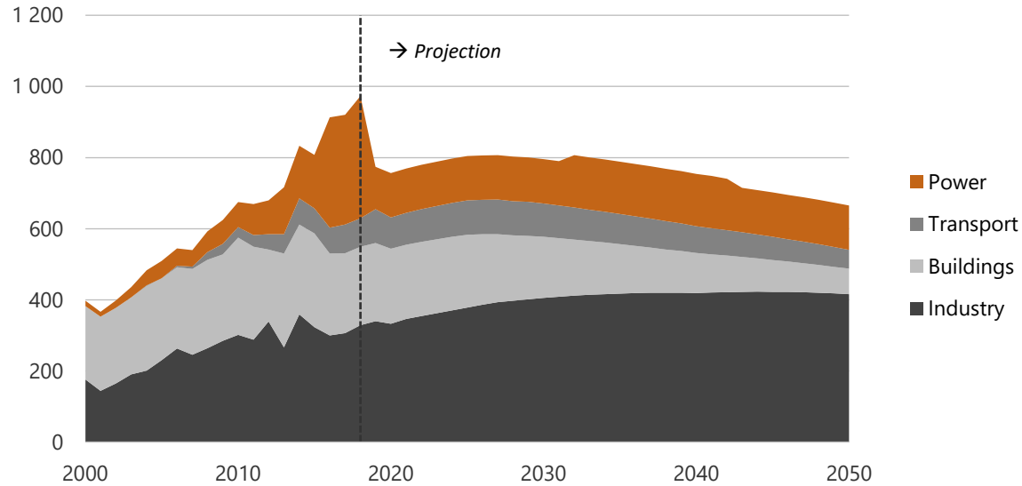
Figure 19-47. Bioenergy consumption by sector in CN, 2000-2050 (PJ).
