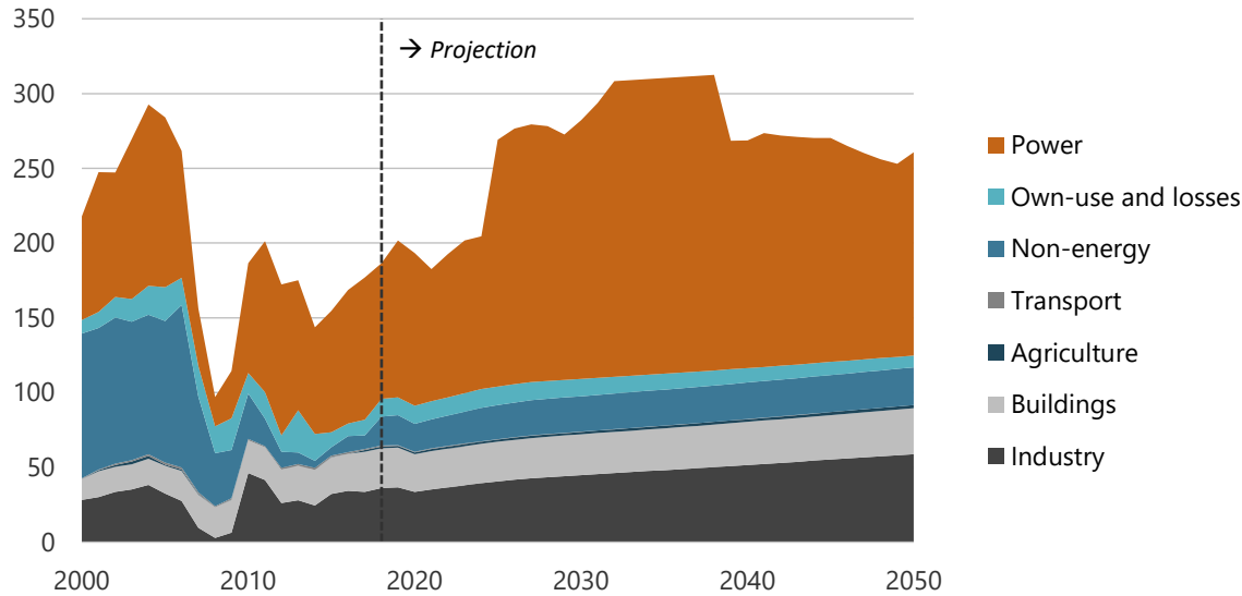
Figure 4-29. Natural gas consumption by sector in REF, 2000-2050 (PJ).
