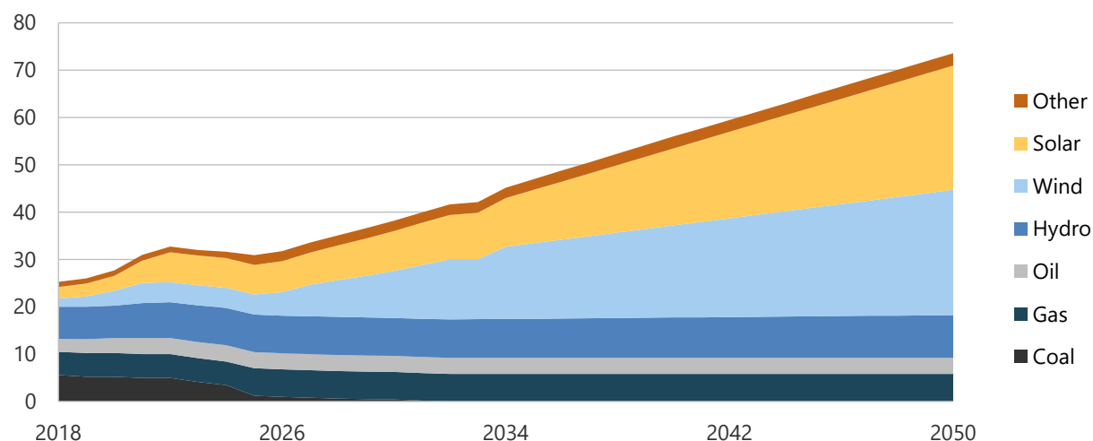
Figure 4-16. Generation capacity in CN, 2018-2050 (GW).
