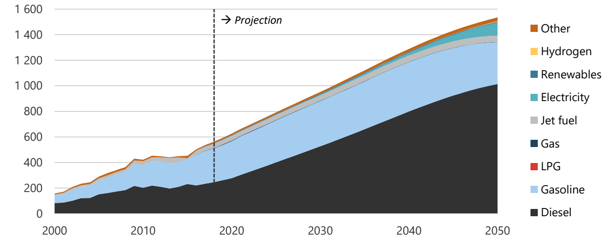
Figure 21-11. Transport energy demand in REF, 2000-2050 (PJ).
