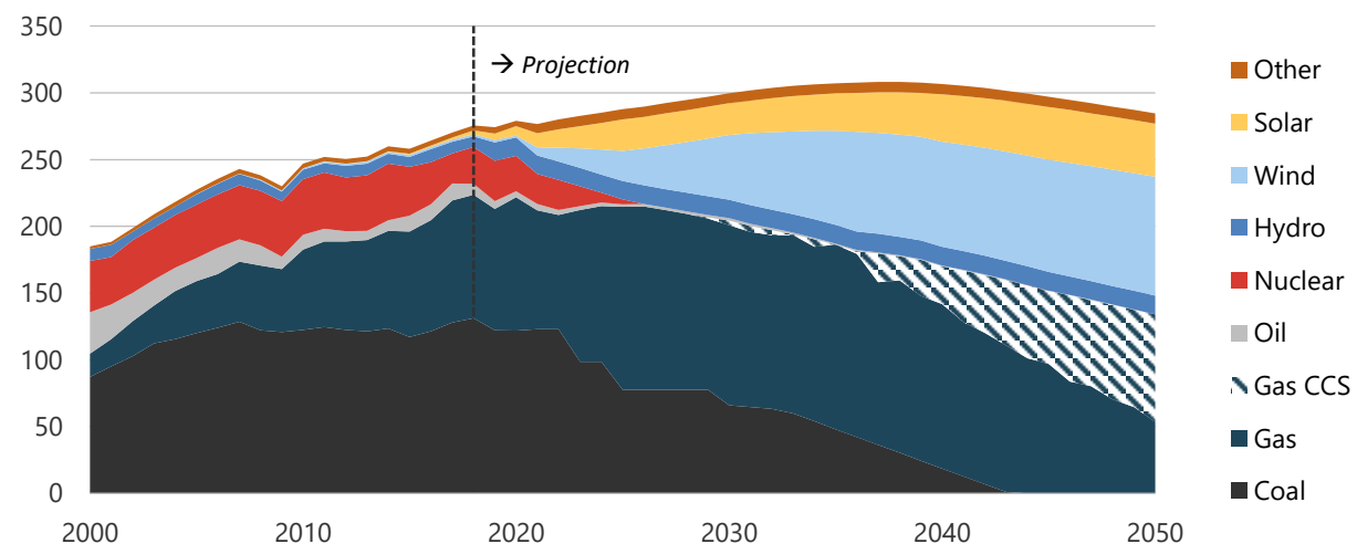
Figure 18-14. Electricity generation in CN, 2000-2050 (TWh).
