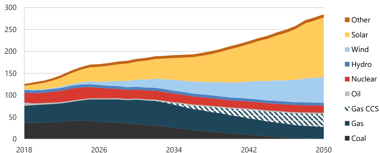
Figure 9-16. Generation capacity in CN, 2018-2050 (GW).
