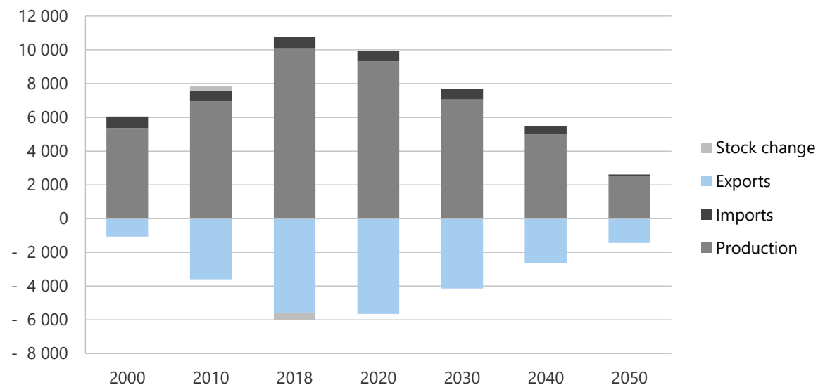
Figure 16-28. Coal production, imports, and exports in CN, 2000-2050 (PJ).
