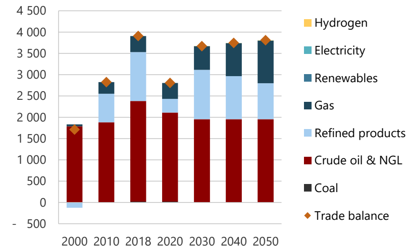
Figure 17-21. Net energy trade in REF, 2000-2050 (PJ).
