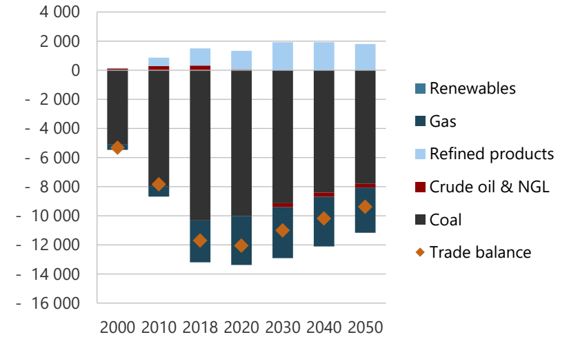
Figure 1-21. Net energy trade in REF, 2000-2050 (PJ).
