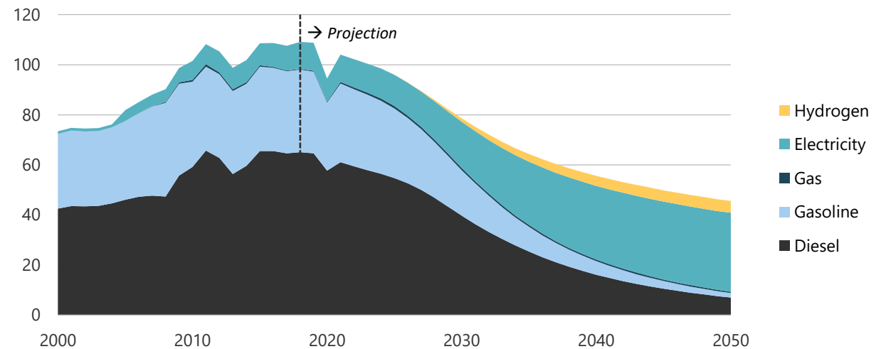
Figure 17-12. Transport energy demand in CN, 2000-2050 (PJ).
