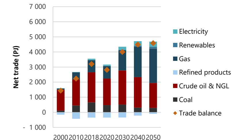
Figure 19-24. Net energy trade in CN, 2000-2050 (PJ).
