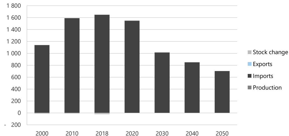
Figure 18-26. Coal production, imports, and exports in REF, 2000-2050 (PJ).
