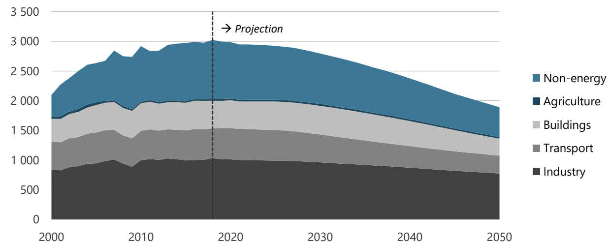
Figure 18-6. Energy demand by sector in CN, 2000-2050 (PJ).
