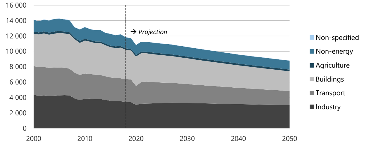
Figure 8-5. Energy demand by sector in REF, 2000-2050 (PJ).
