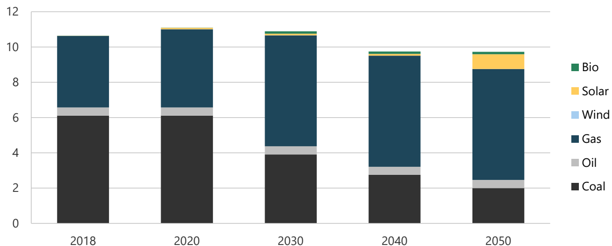
Figure 6-15. Generation capacity in REF, 2018-2050 (GW).
