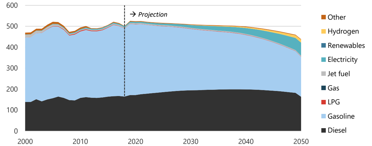
Figure 18-11. Transport energy demand in REF, 2000-2050 (PJ).
