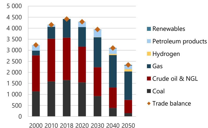
Figure 18-24. Net energy trade in CN, 2000-2050 (PJ).
