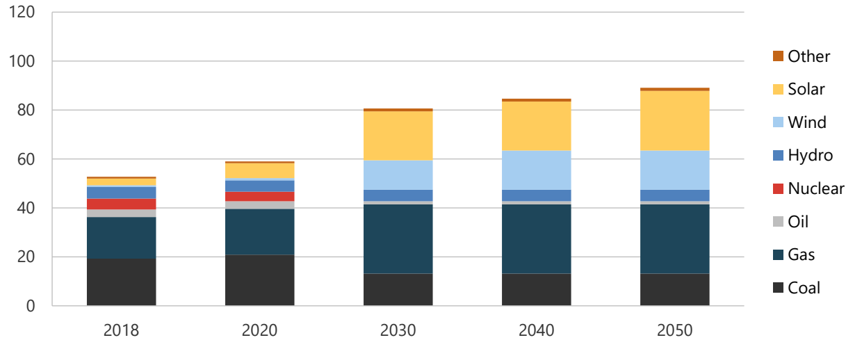
Figure 18-15. Generation capacity in REF, 2018-2050 (GW).
