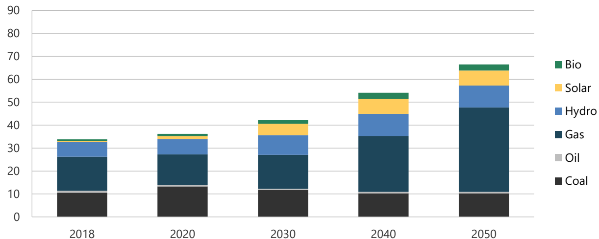
Figure 10-15. Generation capacity in REF, 2018-2050 (GW).
