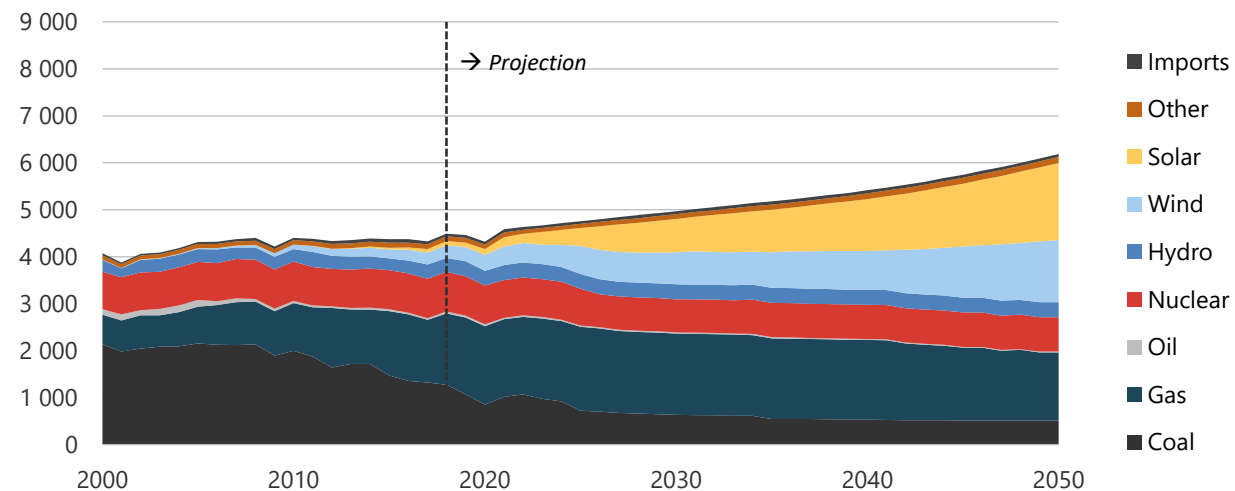
Figure 20-13. Electricity generation in REF, 2000-2050 (TWh).
