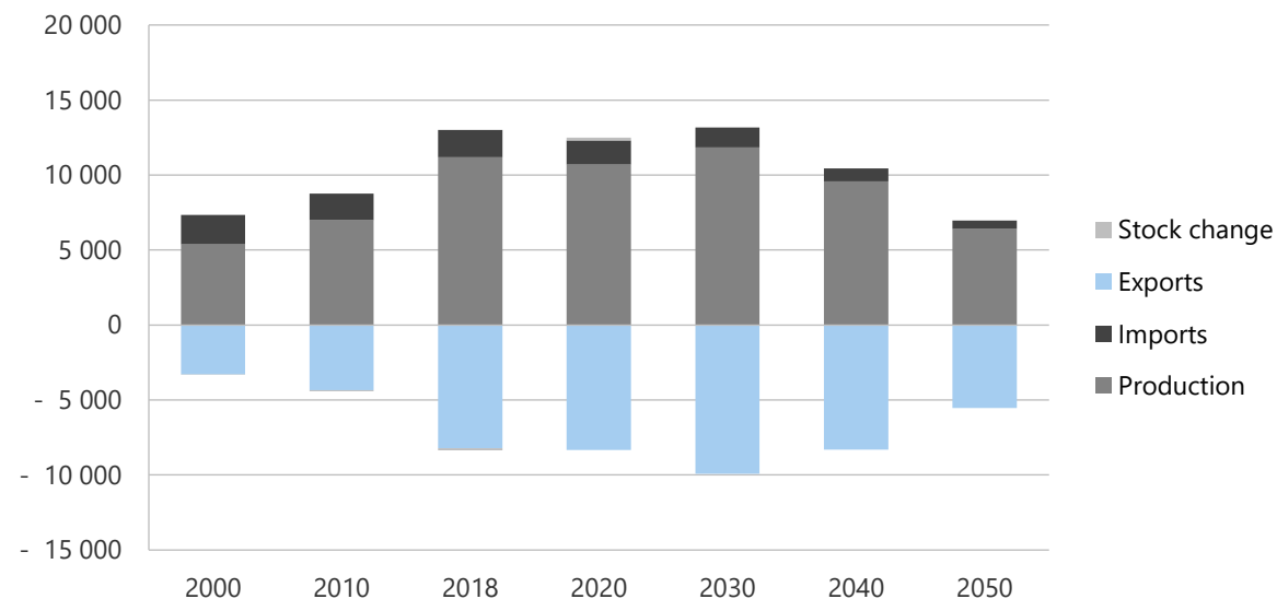
Figure 3-36. Crude oil and NGLs production, imports, and exports in CN, 2000-2050 (PJ).
