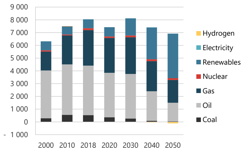
Figure 11-20. Total energy supply in CN, 2000-2050 (PJ).
