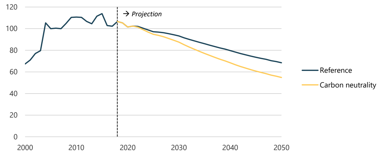
Figure 21-49. Final energy intensity in REF and CN (2005=100).
