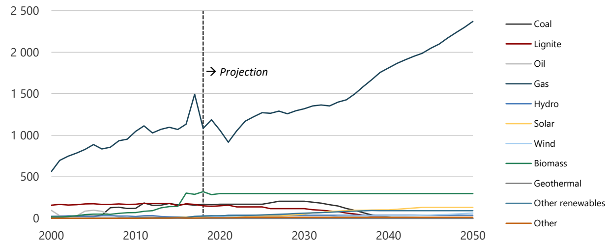
Figure 19-17. Fuel consumption by the power sector in REF, 2000-2050 (PJ).
