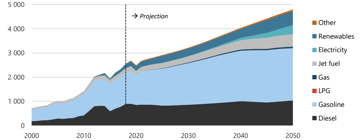
Figure 7-11. Transport energy demand in REF, 2000-2050 (PJ).
