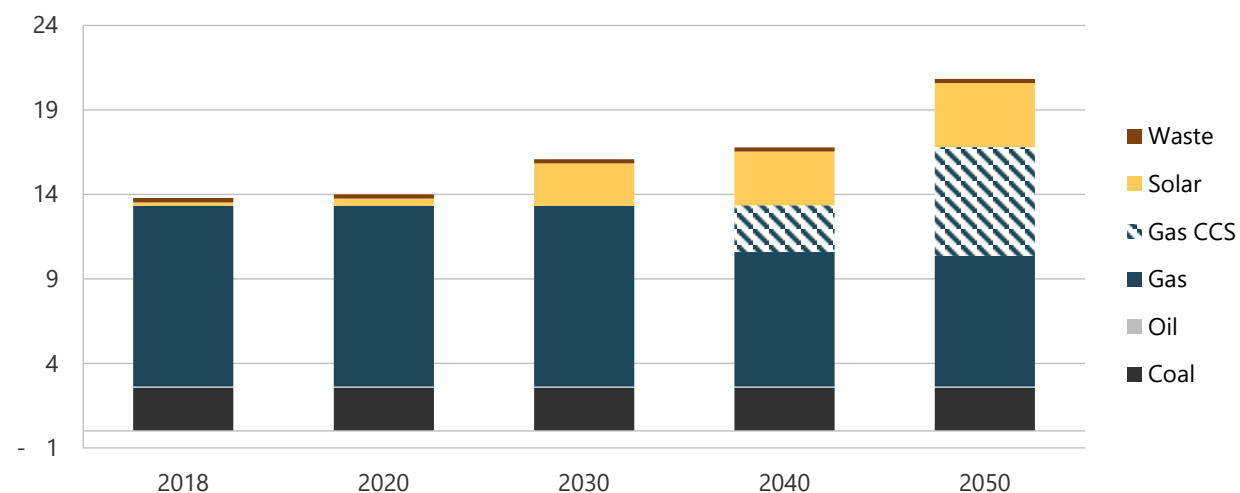
Figure 17-16. Generation capacity in CN, 2017-2050 (GW).
