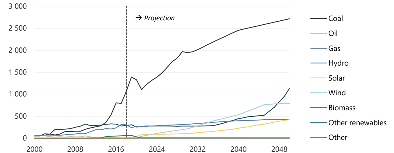
Figure 21-18. Fuel consumption by the power sector in CN, 2000-2050 (PJ).
