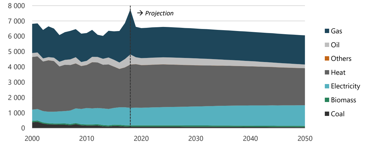
Figure 16-8. Buildings energy demand in CN, 2000-2050 (PJ).
