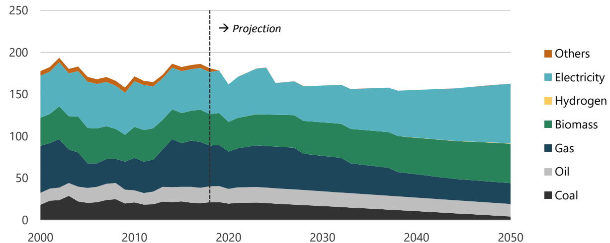
Figure 12-9. Industry energy demand in REF, 2000-2050 (PJ).
