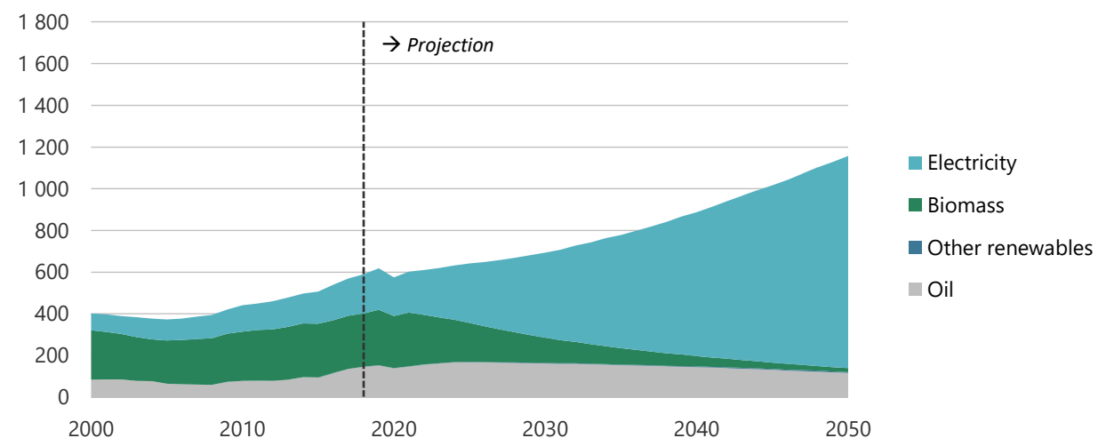
Figure 15-8. Buildings energy demand in CN, 2000-2050 (PJ).
