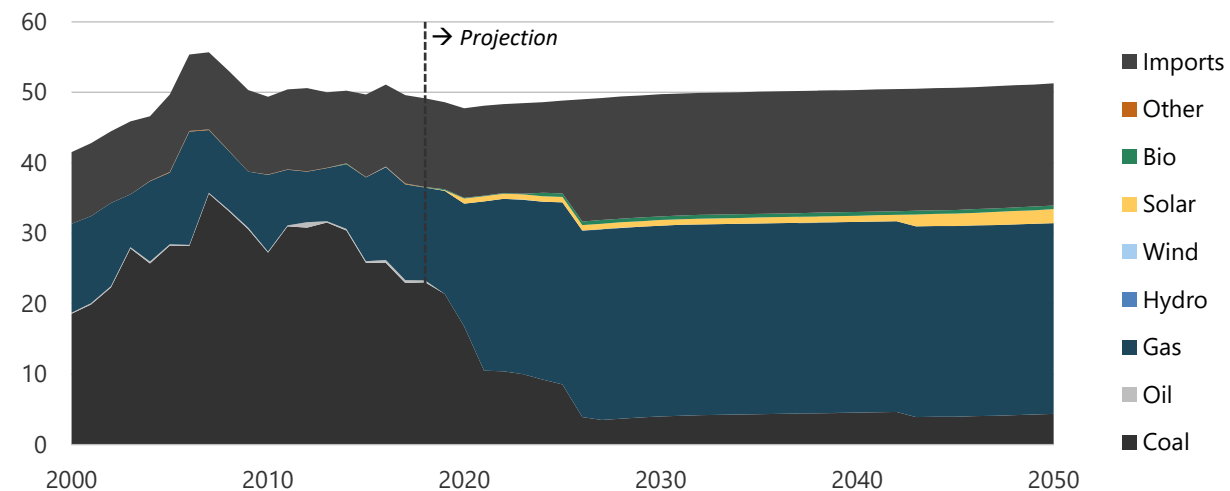
Figure 6-13. Electricity generation in REF, 2000-2050 (TWh).
