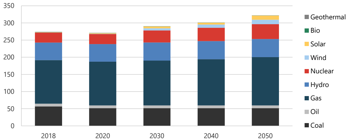
Figure 16-17. Generation capacity in REF, 2018-2050 (GW).
