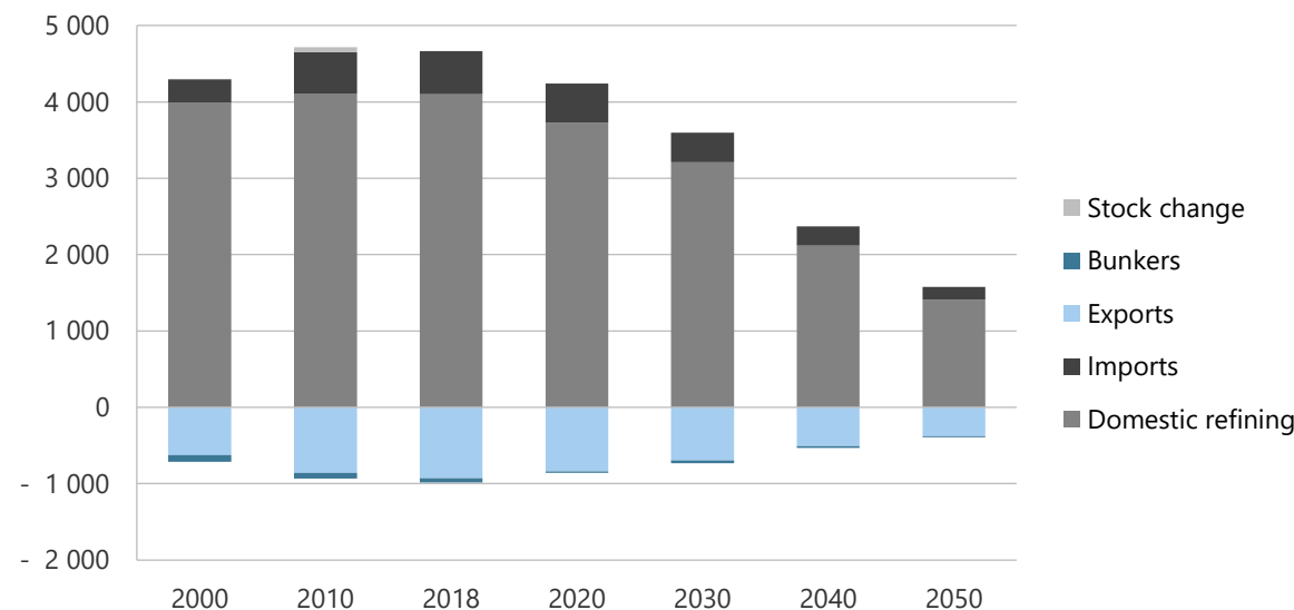
Figure 3-40. Refined products production, imports, and exports in CN, 2000-2050 (PJ).
