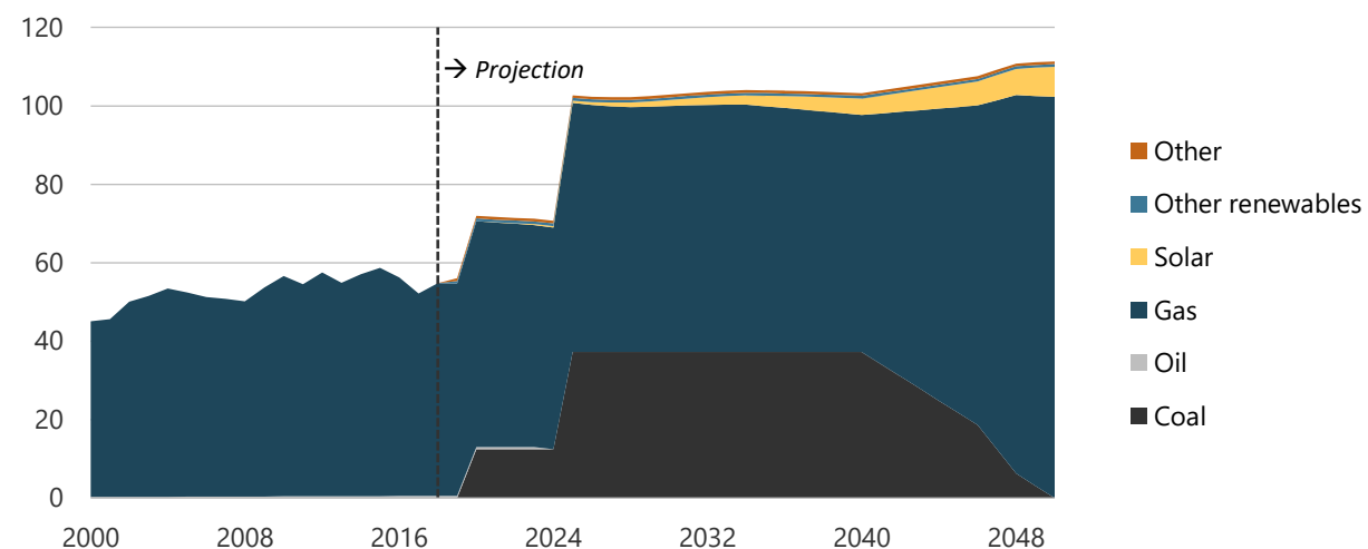
Figure 2-18. Fuel consumption by the power sector in CN, 2000-2050 (PJ).
