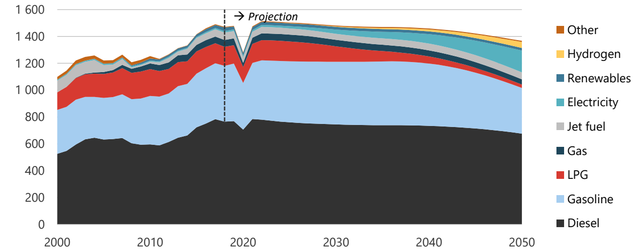
Figure 9-11. Transport energy demand in REF, 2000-2050 (PJ).
