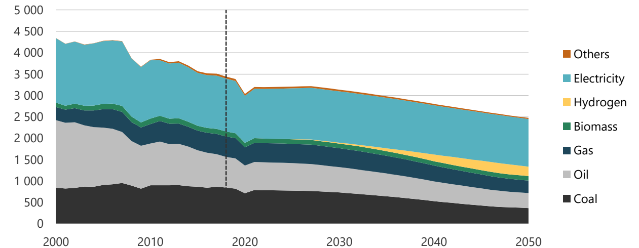
Figure 8-10. Industry energy demand in CN, 2000-2050 (PJ).
