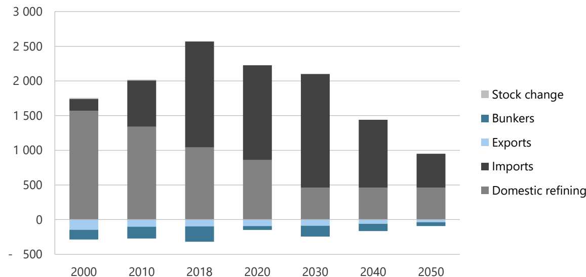
Figure 1-40. Refined products production, imports, and exports in CN, 2000-2050 (PJ).
