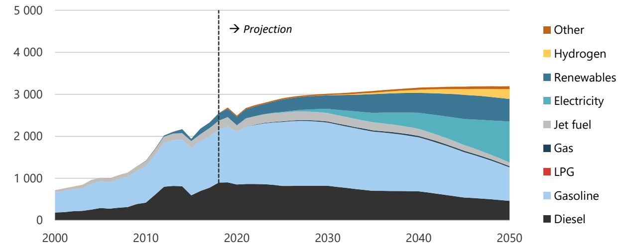
Figure 7-12. Transport energy demand in CN, 2000-2050 (PJ).
