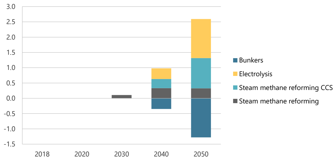
Figure 2-42. Hydrogen production, imports, and exports in CN, 2000-2050 (PJ).
