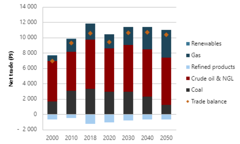
Figure 9-21. Energy trade in REF, 2000-2050 (PJ).
