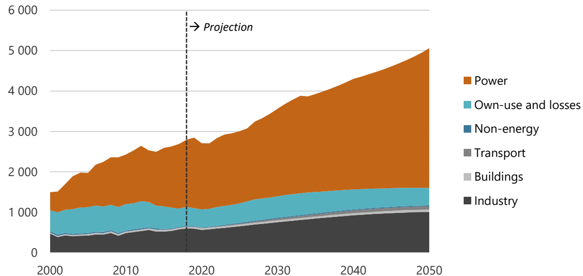
Figure 11-27. Natural gas consumption by sector in REF, 2000-2050 (PJ).
