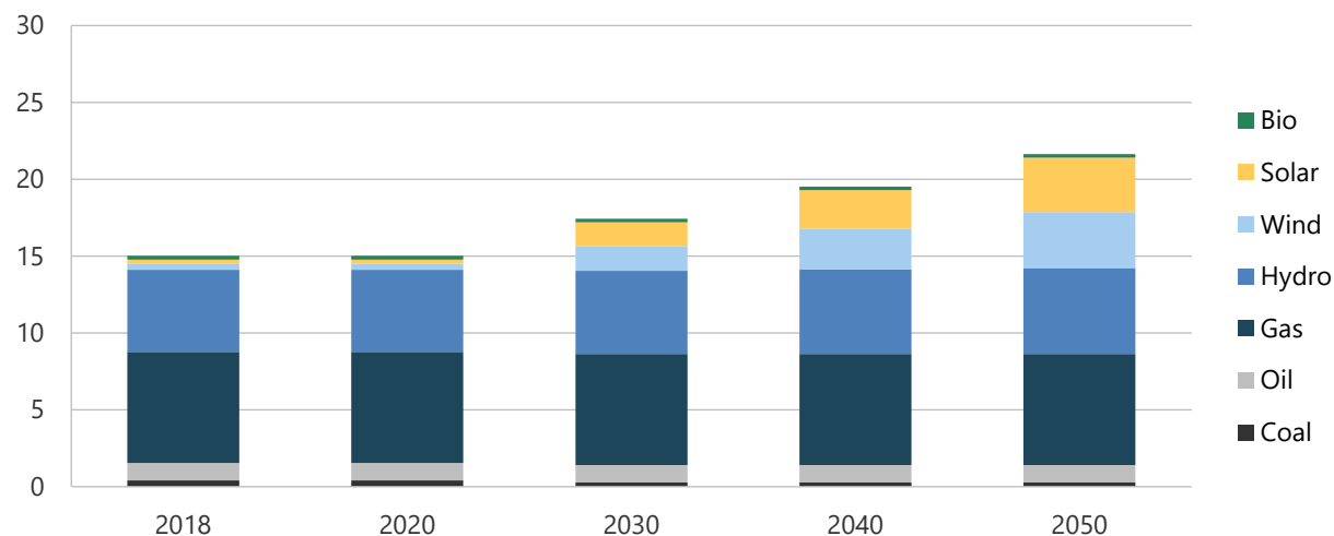
Figure 14-15. Generation capacity in REF, 2018-2050 (GW).
