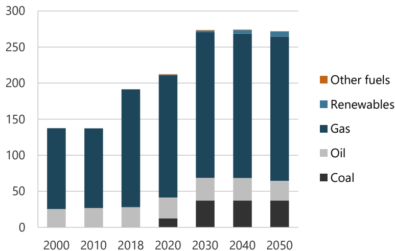
Figure 2-19. Total energy supply in REF, 2000-2050 (PJ).
