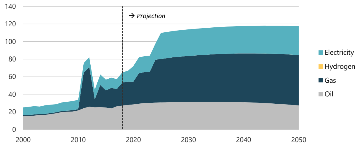
Figure 2-3. Energy demand in REF, 2000-2050 (PJ).
