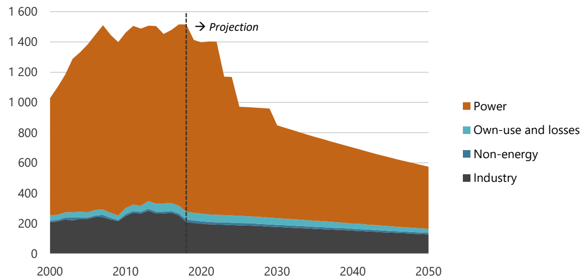
Figure 18-25. Coal consumption by sector in REF, 2000-2050 (PJ).
