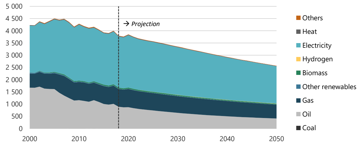
Figure 8-7. Buildings energy demand in REF, 2000-2050 (PJ).
