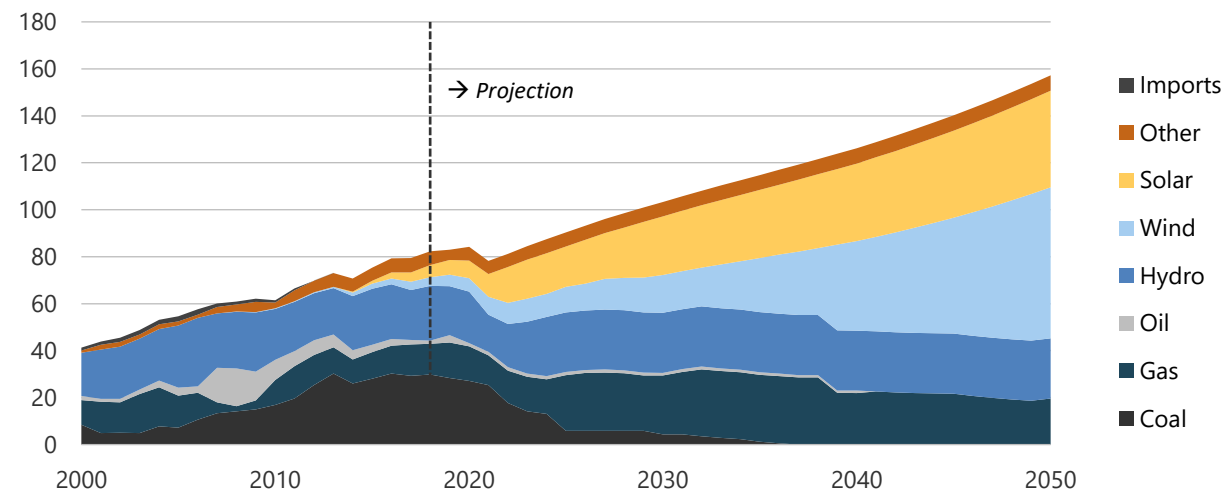
Figure 4-13. Electricity generation in REF, 2000-2050 (TWh).
