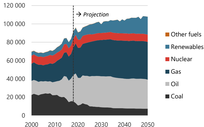
Figure 20-20. Energy production in REF, 2000-2050 (PJ).
