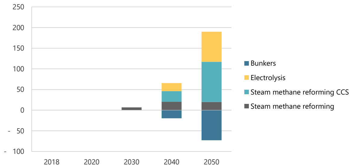
Figure 19-44. Hydrogen production, imports, and exports in CN, 2000-2050 (PJ).
