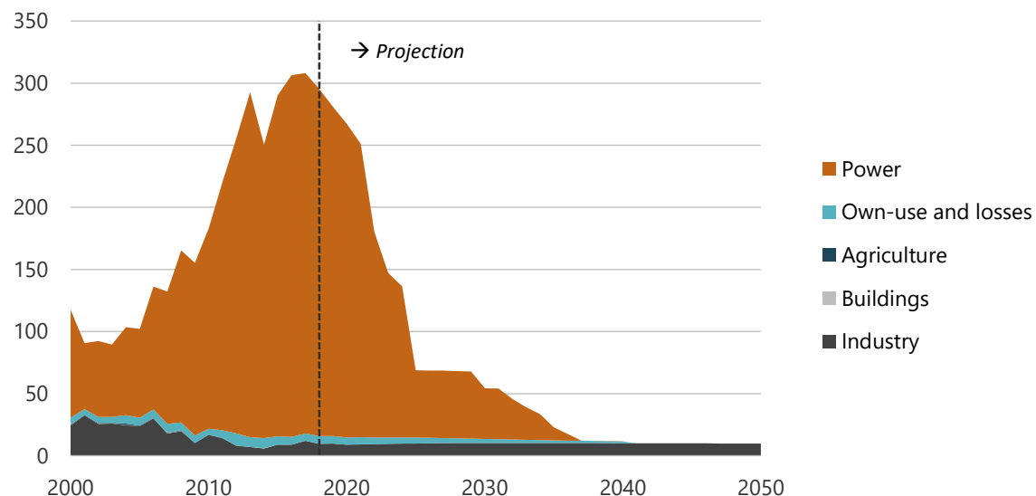
Figure 4-25. Coal consumption by sector in REF, 2000-2050 (PJ).
