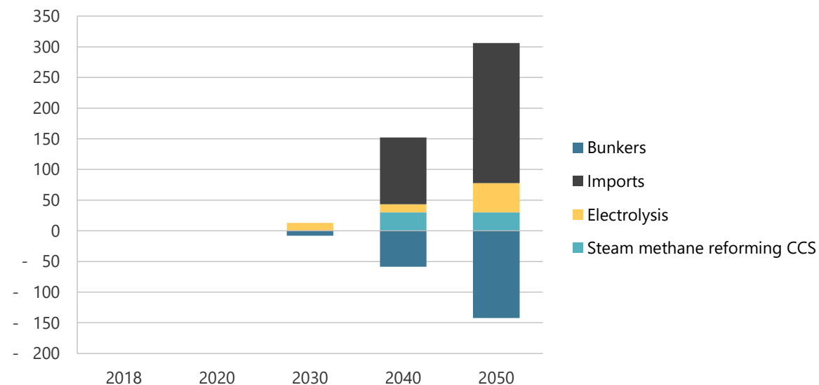
Figure 9-44. Hydrogen production, imports, and exports in CN, 2000-2050 (PJ).
