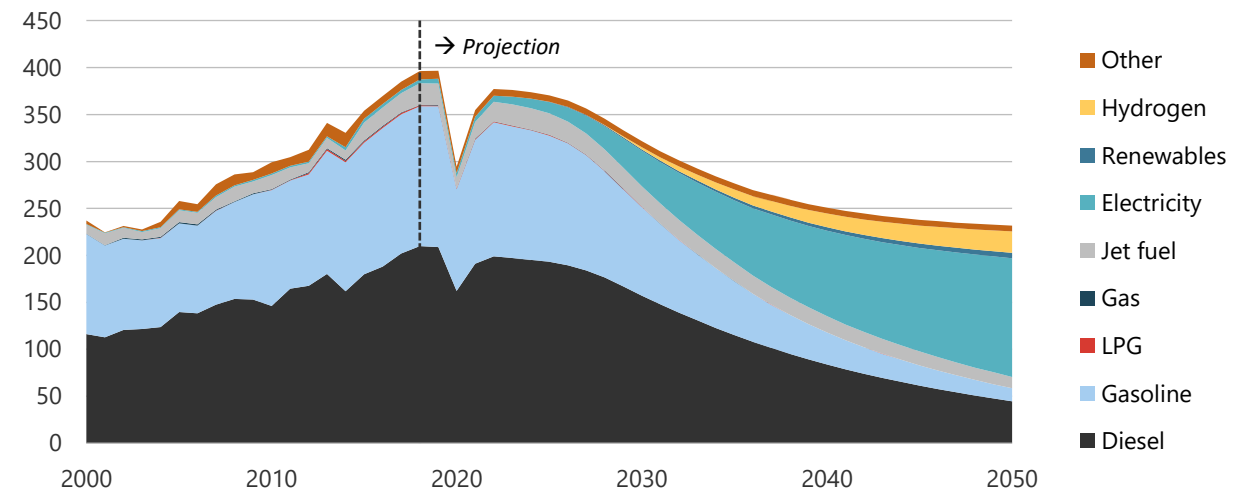
Figure 4-12. Transport energy demand in CN, 2000-2050 (PJ).
