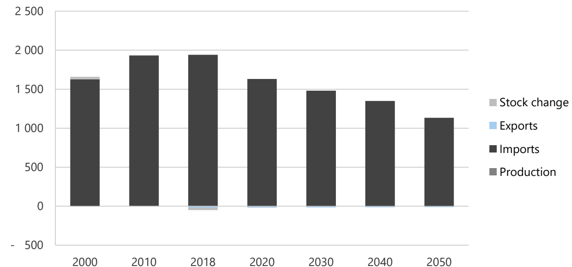
Figure 18-34. Crude oil and NGLs production, imports, and exports in REF, 2000-2050 (PJ).
