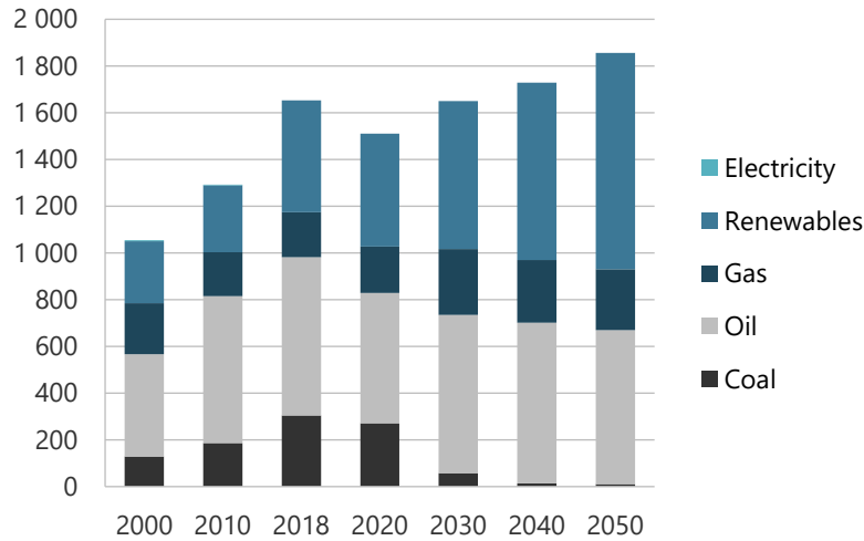
Figure 4-19. Total energy supply in REF, 2000-2050 (PJ).
