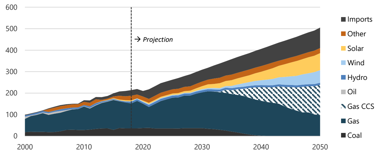
Figure 19-14. Electricity generation in CN, 2000-2050 (TWh).
