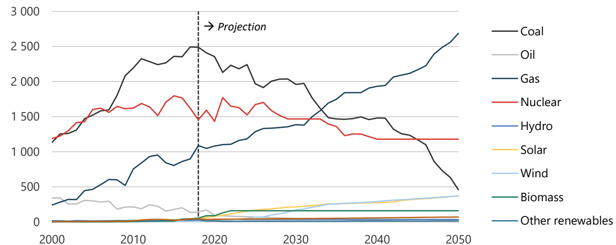
Figure 9-17. Fuel consumption by the power sector in REF, 2000-2050 (PJ).
