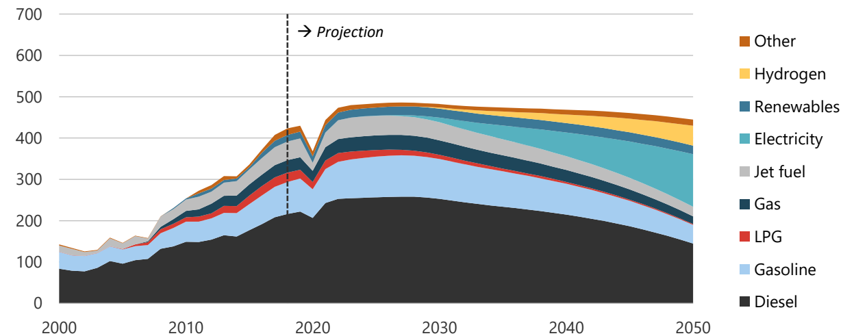
Figure 14-12. Transport energy demand in CN, 2000-2050 (PJ).
