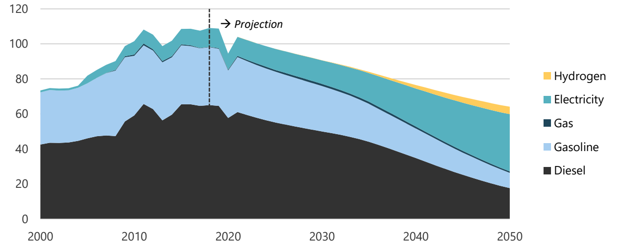
Figure 17-11. Transport energy demand in REF, 2000-2050 (PJ).
