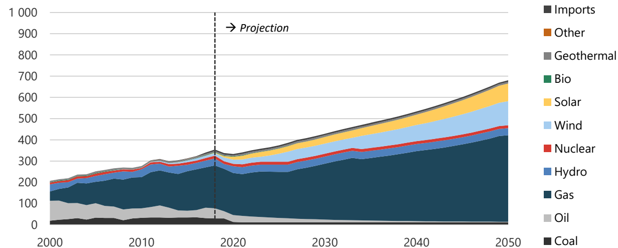
Figure 11-13. Electricity generation in REF, 2000-2050 (TWh).
