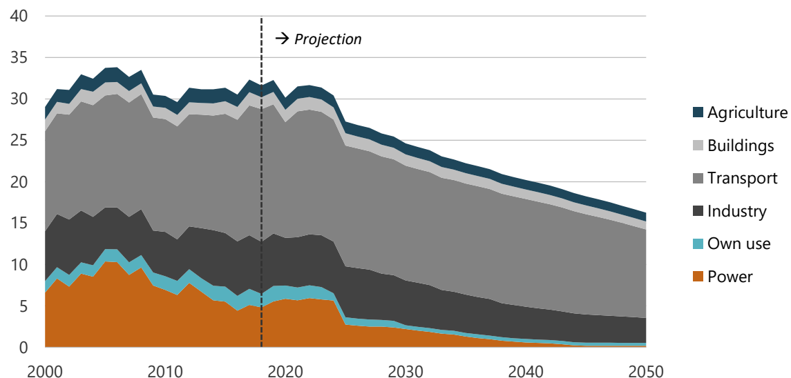
Figure 12-51. Gross CO 2 emissions in REF, 2000-2050 (million tonnes).
