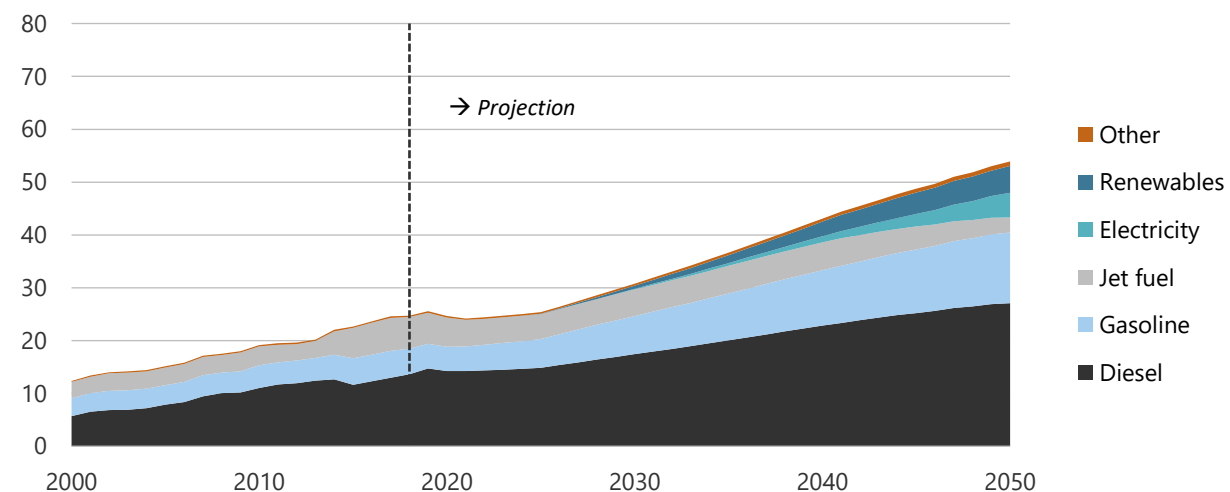
Figure 13-12. Transport energy demand in CN, 2000-2050 (PJ).
