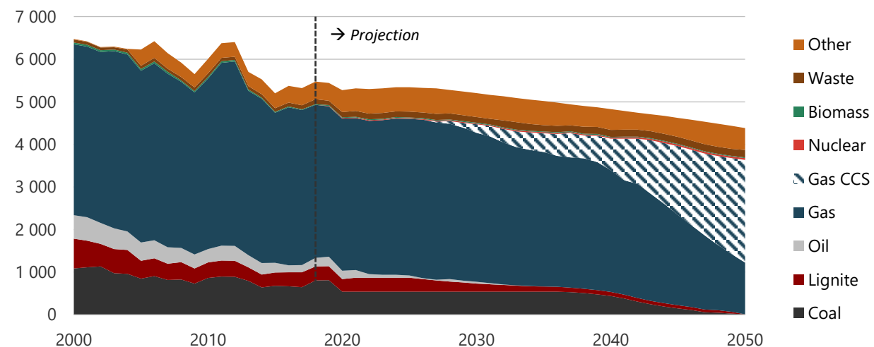
Figure 16-16. Heat generation in CN, 2000-2050 (PJ).
