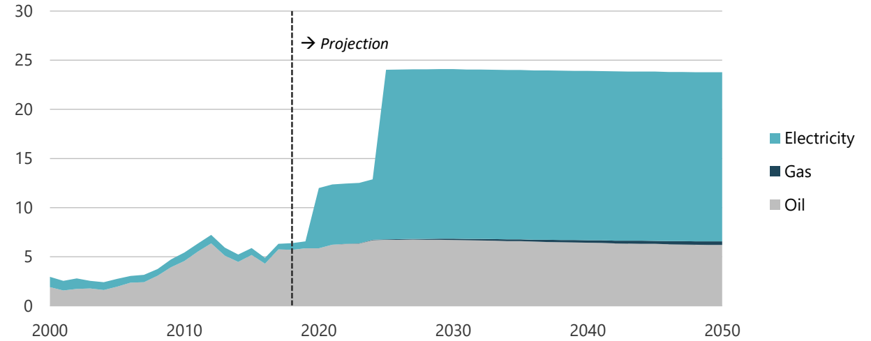
Figure 2-9. Industry energy demand in REF, 2000-2050 (PJ).
