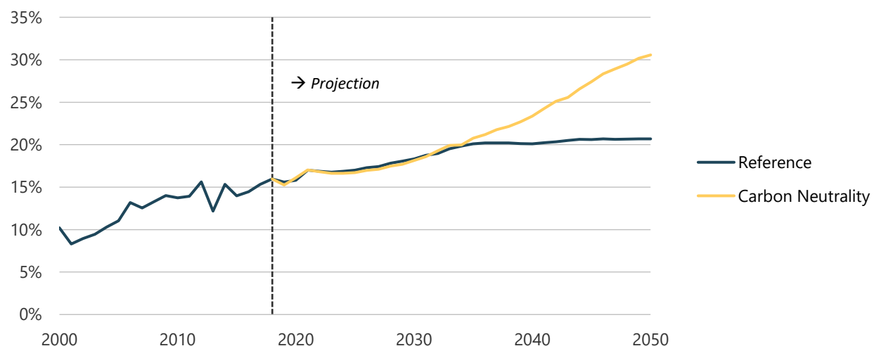
Figure 19-50. Modern renewables share in REF and CN, 2000-2050.
