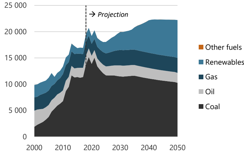
Figure 7-20. Energy production in REF, 2000-2050 (PJ).
