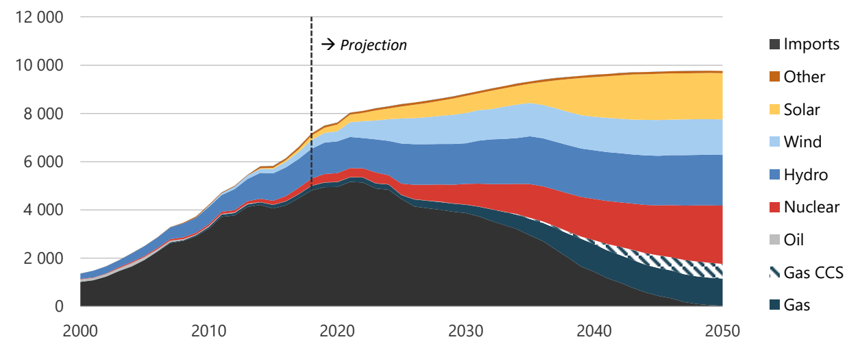
Figure 5-14. Electricity generation in CN, 2000-2050 (TWh).
