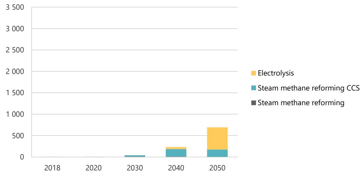
Figure 20-42. Hydrogen production, imports, and exports in REF, 2000-2050 (PJ).
