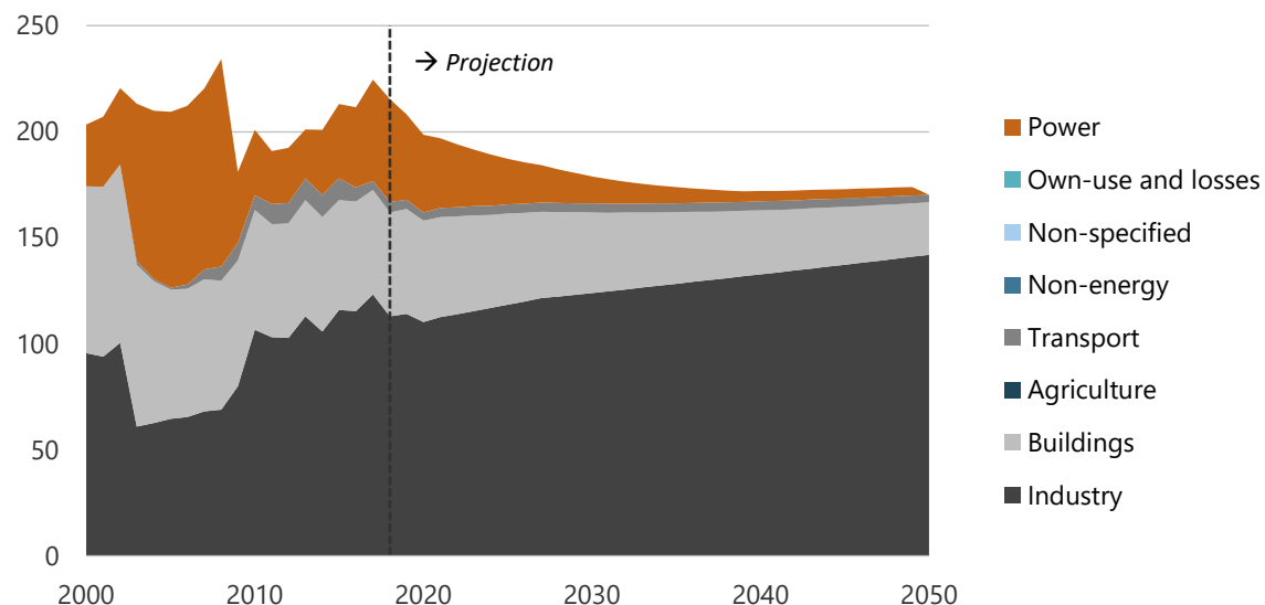
Figure 1-45. Bioenergy consumption by sector in REF, 2000-2050 (PJ).
