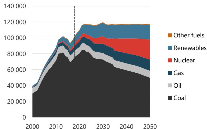
Figure 5-18. Energy production in REF, 2000-2050 (PJ).
