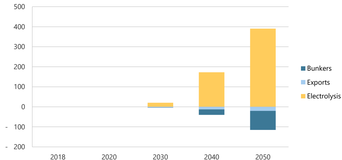
Figure 11-42. Hydrogen production, imports, and exports in CN, 2000-2050 (PJ).
