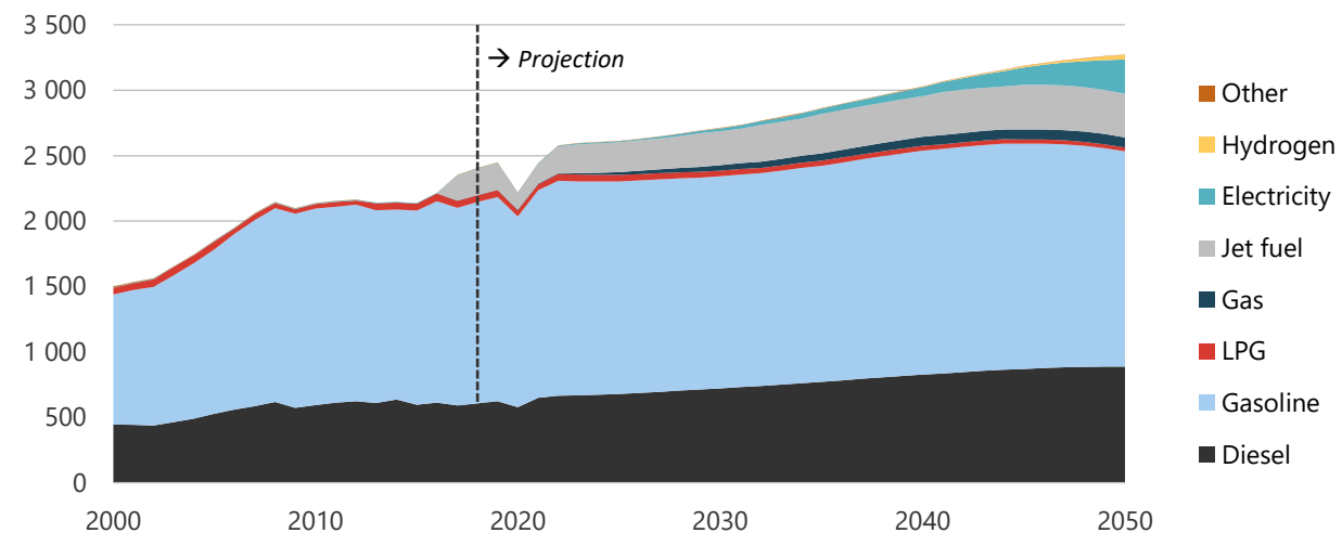
Figure 11-11. Transport energy demand in REF, 2000-2050 (PJ).
