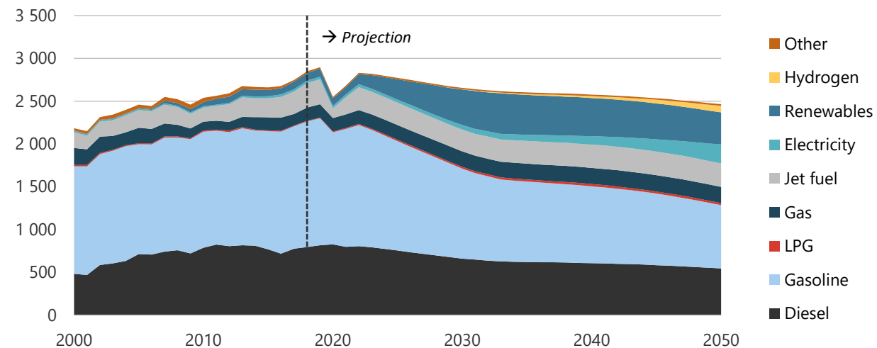
Figure 3-11. Transport energy demand in REF, 2000-2050 (PJ).
