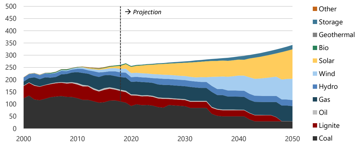
Figure 1-13. Electricity generation in REF, 2000-2050 (TWh).
