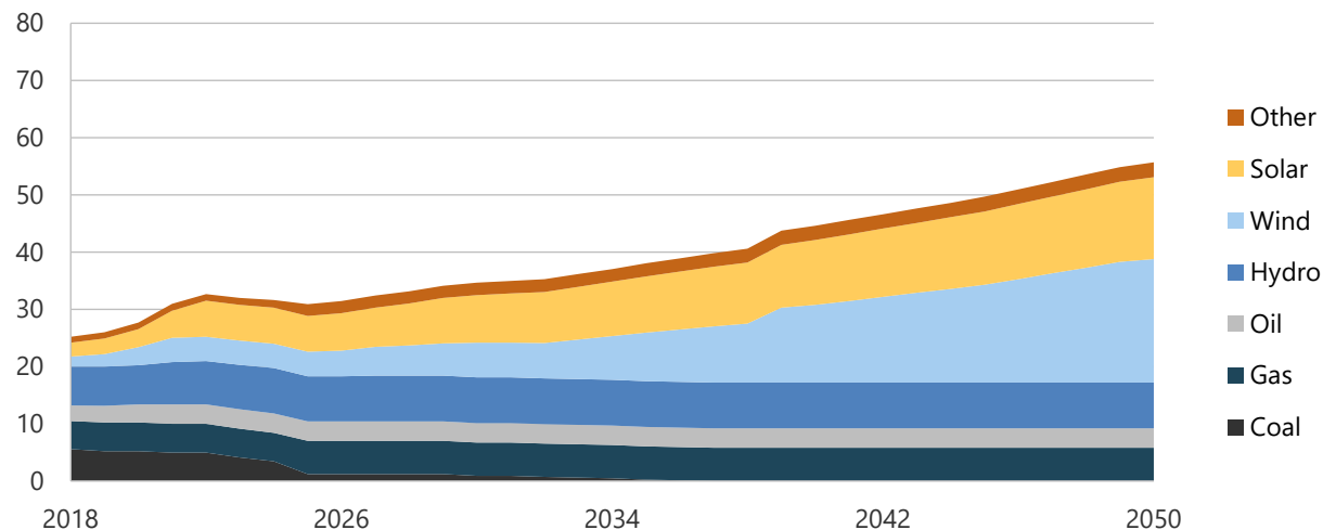
Figure 4-15. Generation capacity in REF, 2018-2050 (GW).
