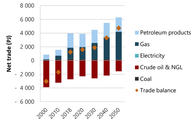
Figure 11-19. Net energy trade in REF, 2000-2050 (PJ).
