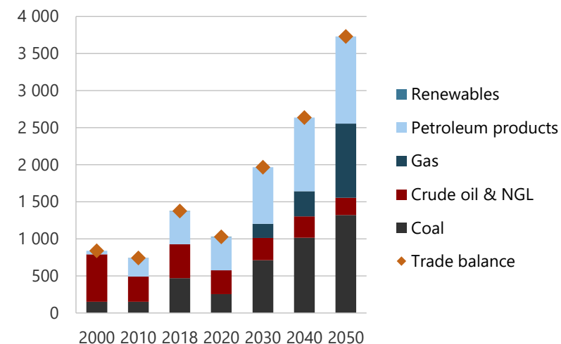
Figure 15-21. Net energy trade in REF, 2000-2050 (PJ).
