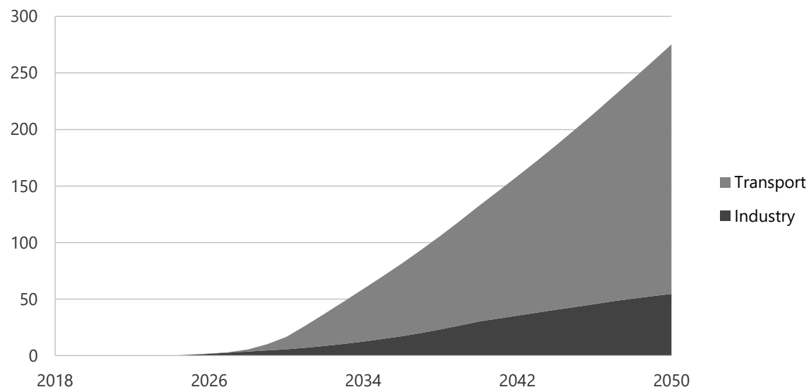
Figure 11-41. Hydrogen consumption by sector in CN, 2000-2050 (PJ).
