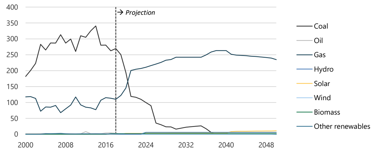
Figure 6-18. Fuel consumption by the power sector in CN, 2000-2050 (PJ).
