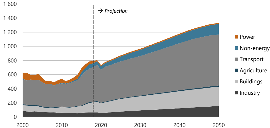
Figure 15-37. Refined products consumption by sector in REF, 2000-2050 (PJ).
