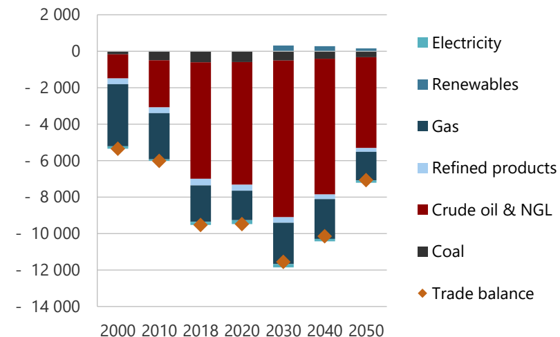
Figure 3-24. Net energy trade in CN, 2000-2050 (PJ).
