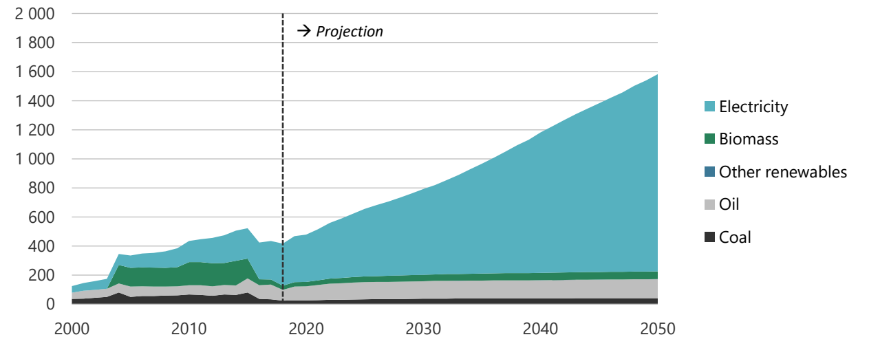
Figure 21-8. Buildings energy demand in CN, 2000-2050 (PJ).
