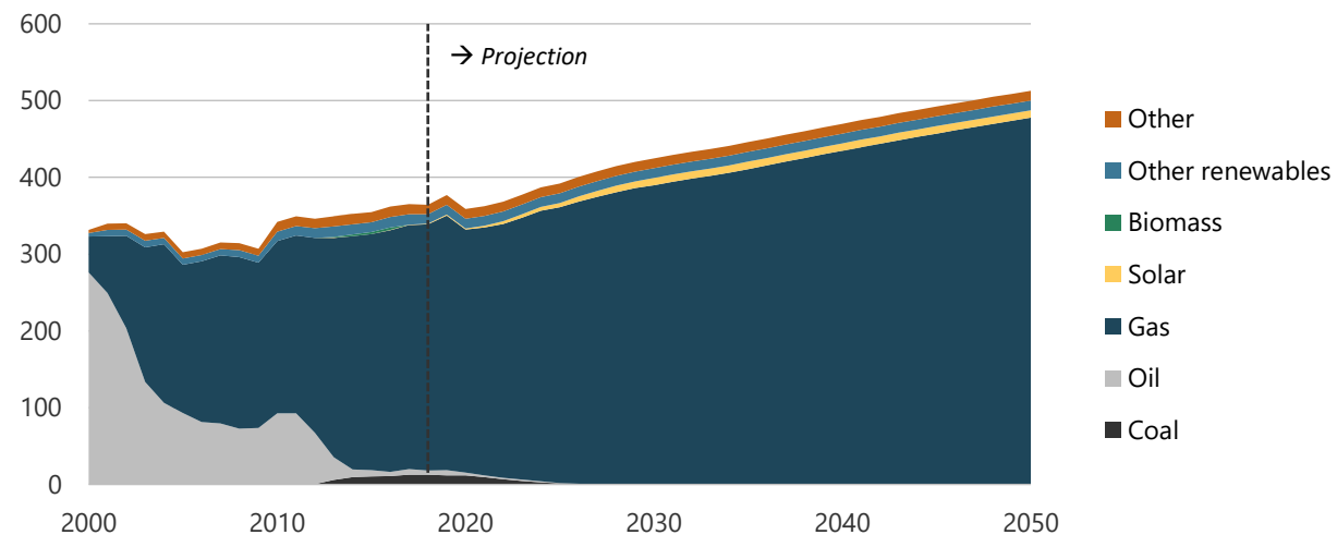
Figure 17-17. Fuel consumption by the power sector in REF, 2000-2050 (PJ).
