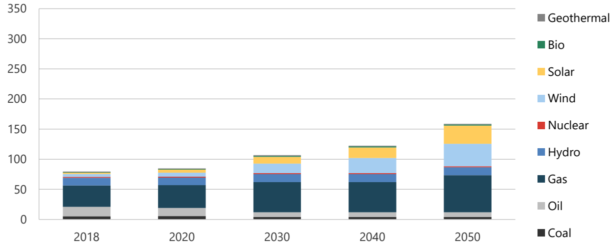
Figure 11-15. Generation capacity in REF, 2018-2050 (GW).
