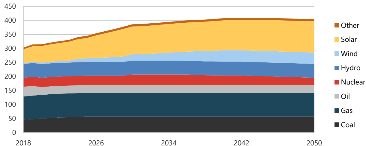
Figure 8-15. Generation capacity in REF, 2018-2050 (GW).
