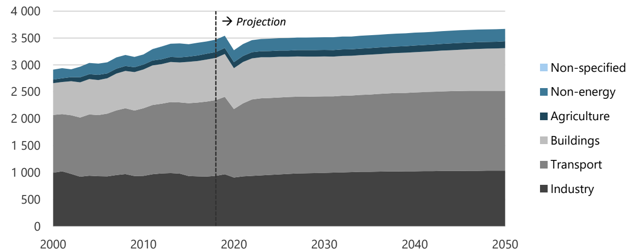
Figure 1-5. Energy demand by sector in REF, 2000-2050 (PJ).
