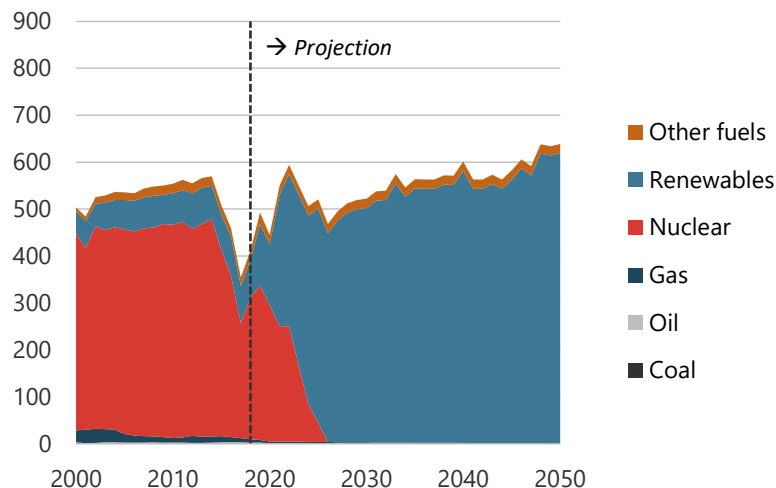
Figure 18-20. Energy production in REF, 2000-2050 (PJ).
