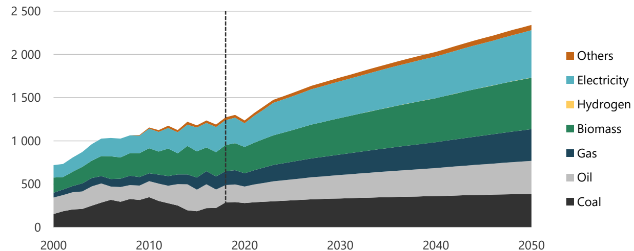
Figure 19-9. Industry energy demand in REF, 2000-2050 (PJ).
