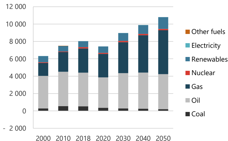
Figure 11-17. Total energy supply in REF, 2000-2050 (PJ).
