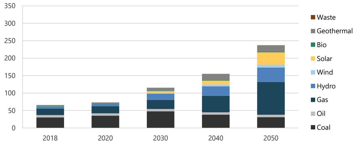
Figure 7-15. Generation capacity in REF, 2018-2050 (GW).
