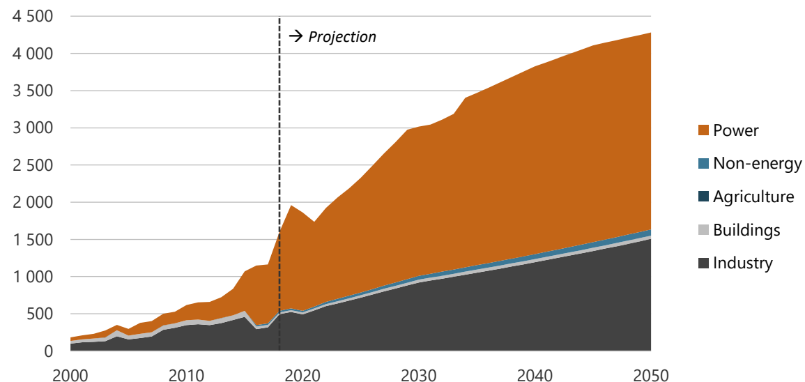
Figure 21-25. Coal consumption by sector in REF, 2000-2050 (PJ).
