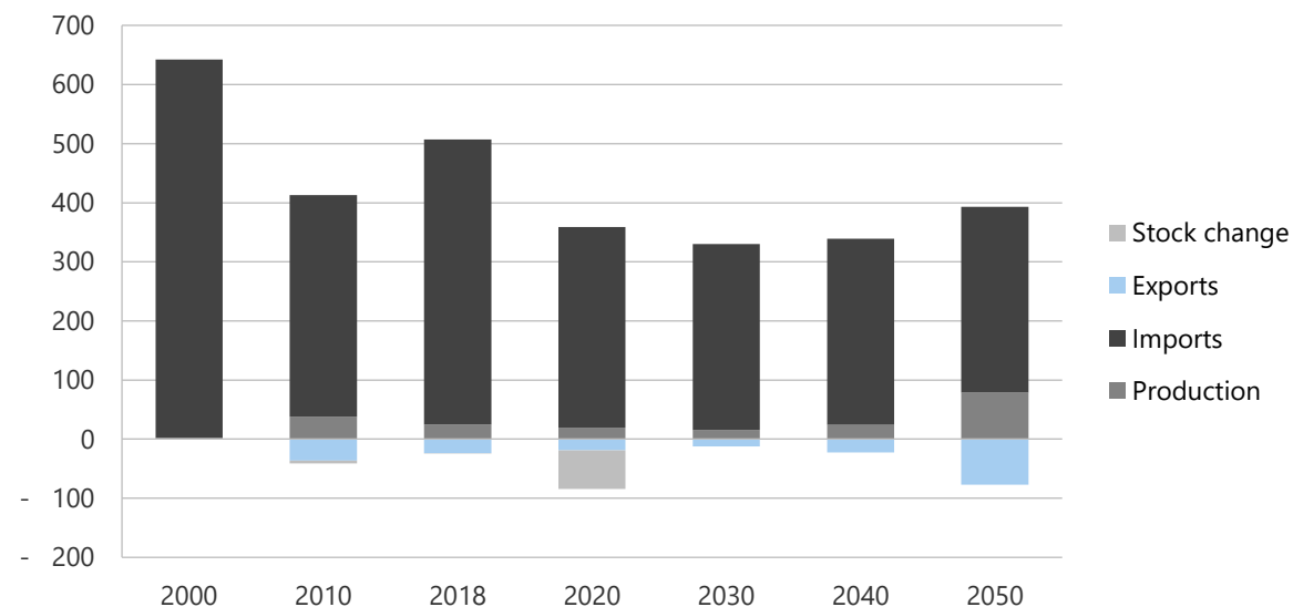
Figure 15-36. Crude oil and NGL production, imports, and exports in CN, 2000-2050 (PJ).
