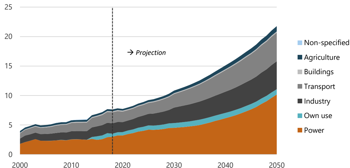
Figure 13-37. Gross CO 2 emissions in REF, 2000-2050 (million tonnes).
