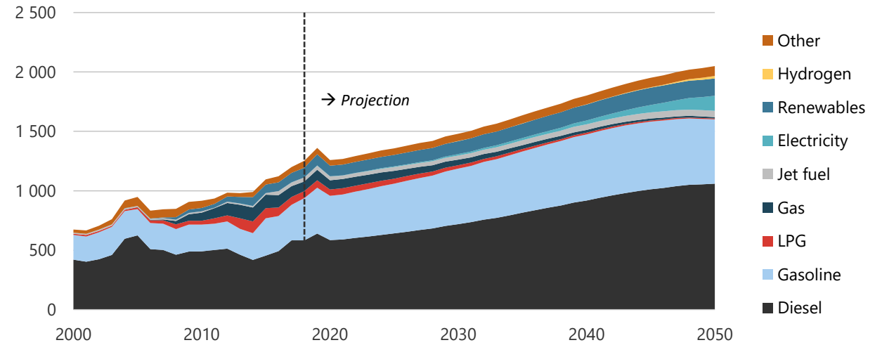
Figure 19-11. Transport energy demand in REF, 2000-2050 (PJ).
