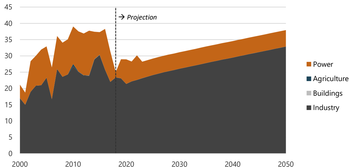
Figure 14-23. Coal consumption by sector in REF, 2000-2050 (PJ).
