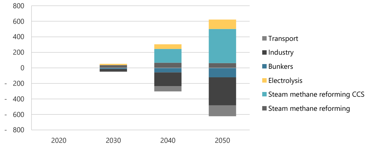
Figure 16-40. Hydrogen production, consumption, imports, and exports in CN, 2000-2050 (PJ).
