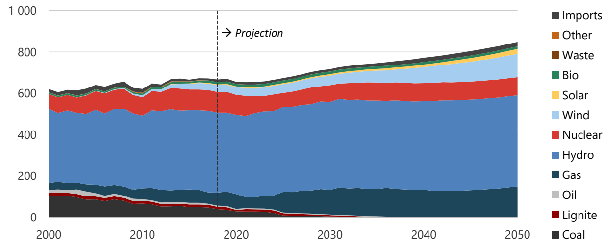
Figure 3-13. Electricity generation in REF, 2000-2050 (TWh).
