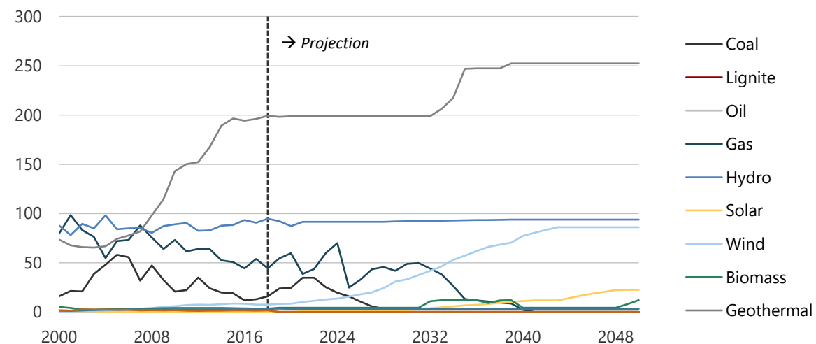
Figure 12-18. Fuel consumption by the power sector in CN, 2000-2050 (PJ).
