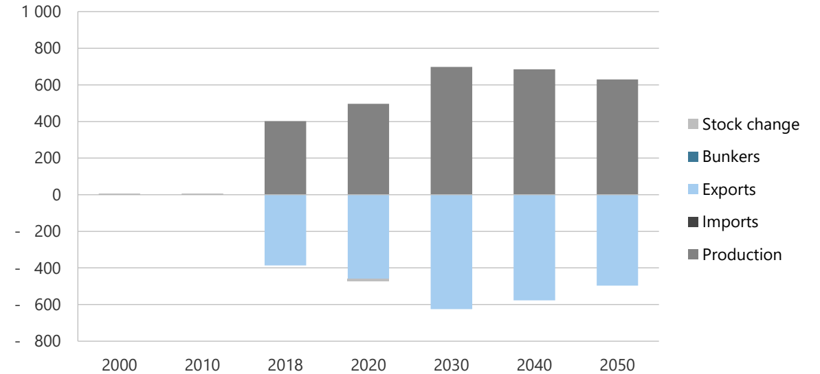
Figure 13-26. Natural gas production, imports, and exports in CN, 2000-2050 (PJ).
