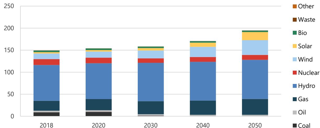
Figure 3-15. Generation capacity in REF, 2017-2050 (GW).
