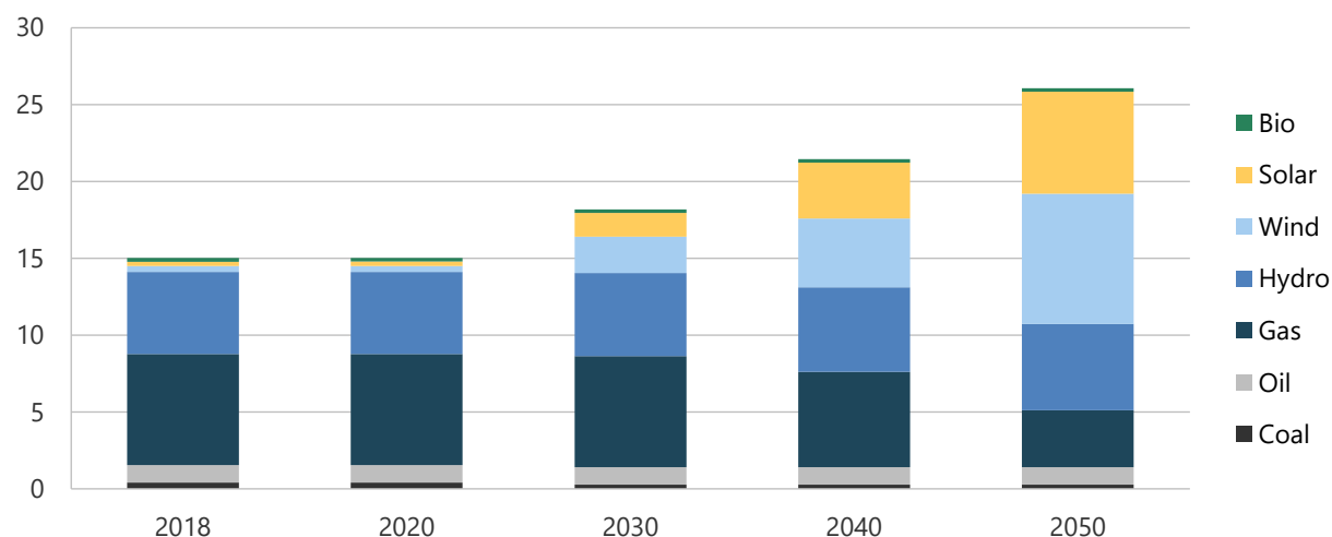
Figure 14-16. Generation capacity in CN, 2018-2050 (GW).
