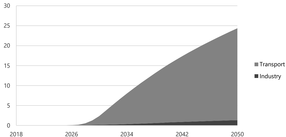
Figure 4-43. Hydrogen consumption by sector in CN, 2000-2050 (PJ).
