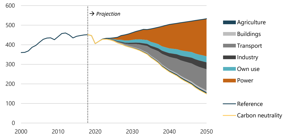
Figure 11-50. Change in gross CO 2 emissions, 2000-2050 (million tonnes).
