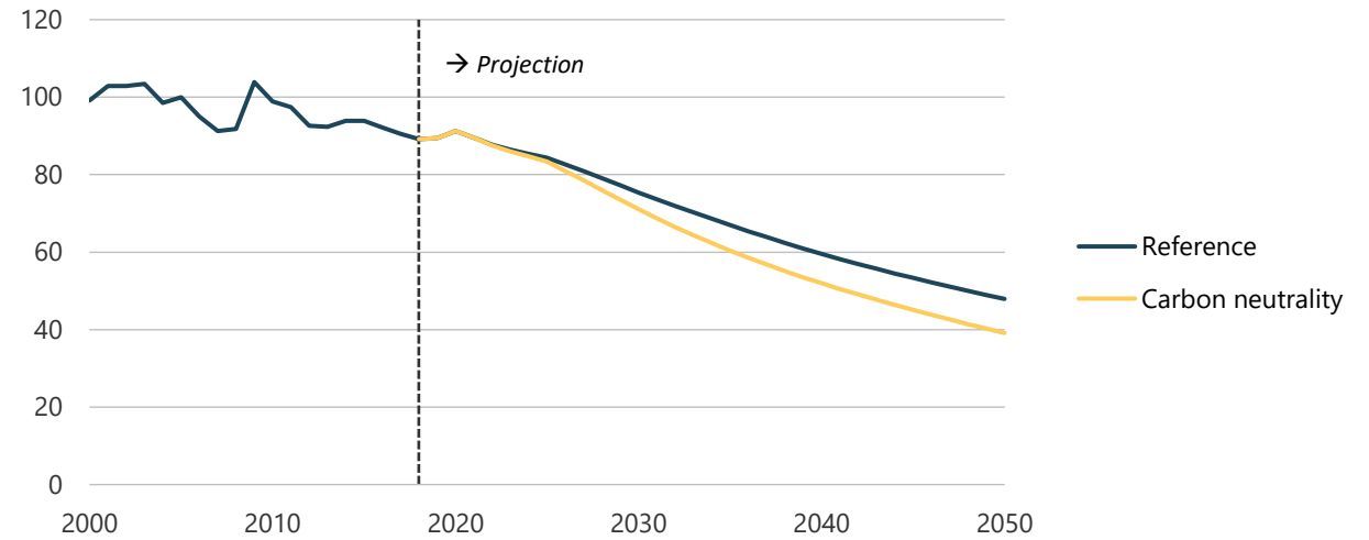
Figure 17-49. Final energy intensity in REF and CN (2005=100).
