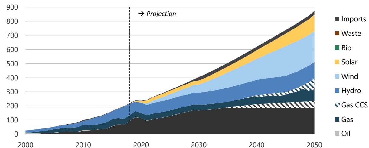
Figure 21-14. Electricity generation in CN, 2000-2050 (TWh).
