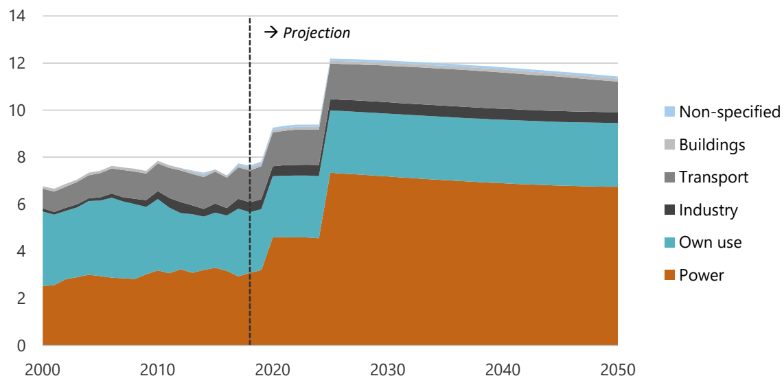
Figure 2-45. Gross CO 2 emissions in REF, 2000-2050 (million tonnes).
