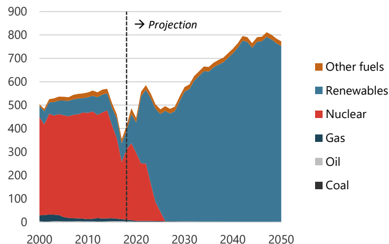
Figure 18-23. Energy production in CN, 2000-2050 (PJ).
