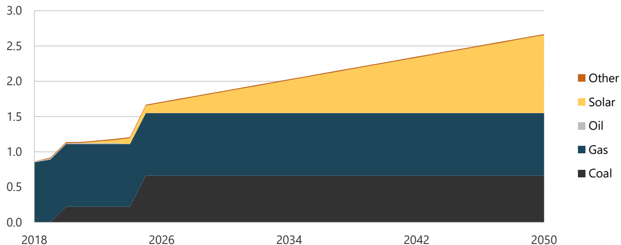
Figure 2-15. Generation capacity in REF, 2018-2050 (GW).
