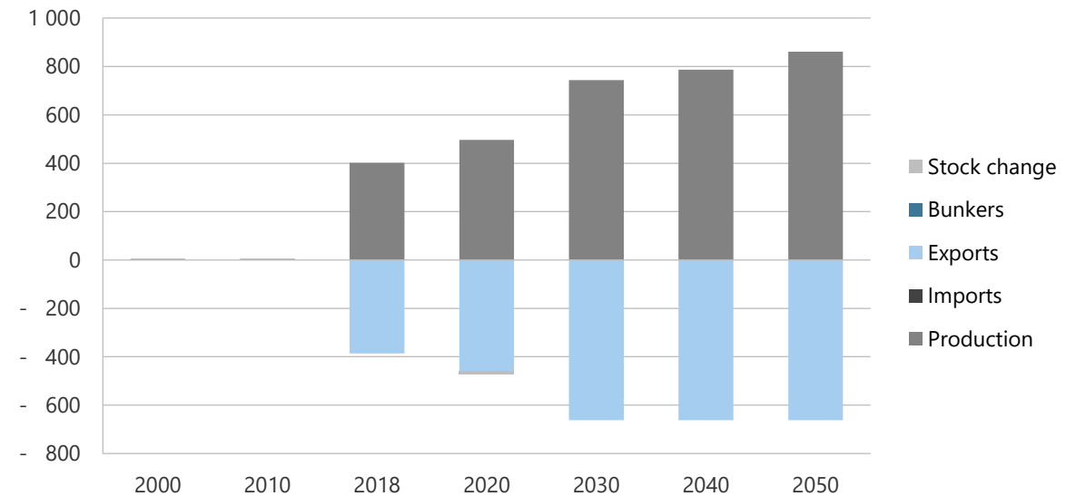
Figure 13-24. Natural gas production, imports, and exports in REF, 2000-2050 (PJ).
