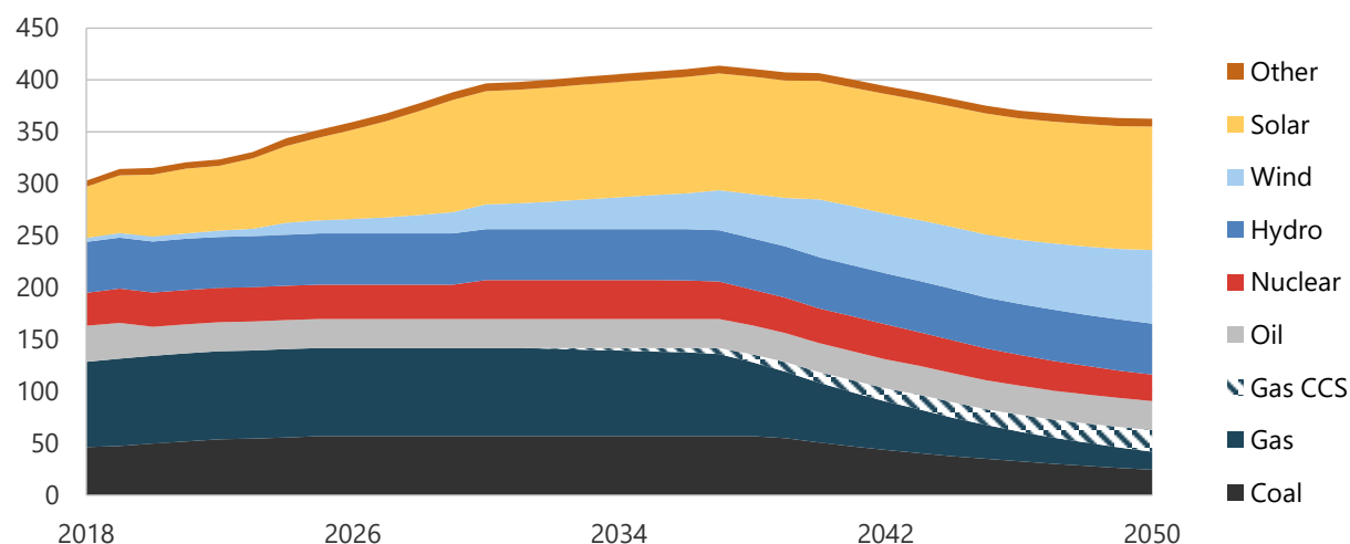
Figure 8-16. Generation capacity in CN, 2018-2050 (GW).
