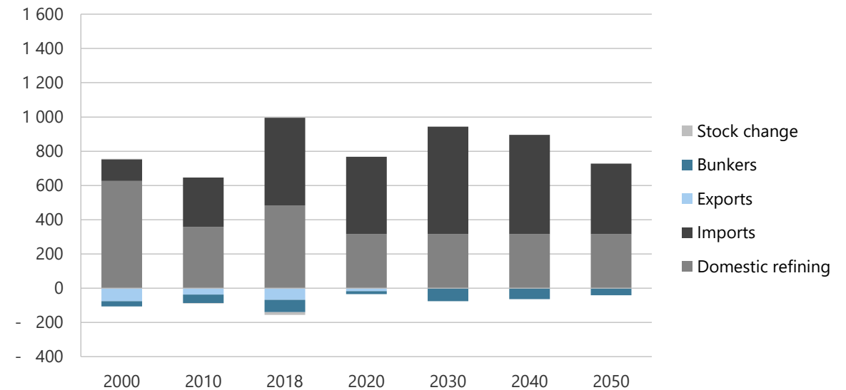
Figure 15-40. Refined products production, imports, and exports in CN, 2000-2050 (PJ).
