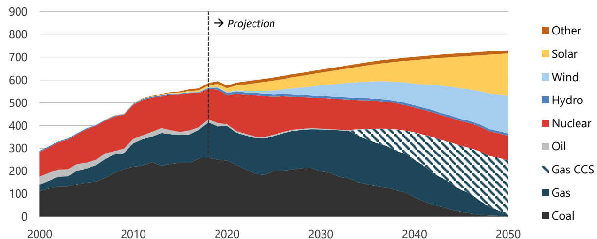
Figure 9-14. Electricity generation in CN, 2000-2050 (TWh).
