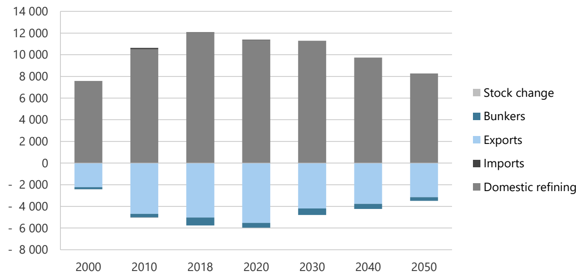
Figure 16-38. Refined product production, imports, and exports in CN, 2000-2050 (PJ).
