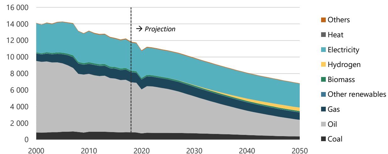
Figure 8-4. Energy demand in CN, 2000-2050 (PJ).
