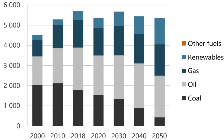
Figure 1-19. Total energy supply in REF, 2000-2050 (PJ).
