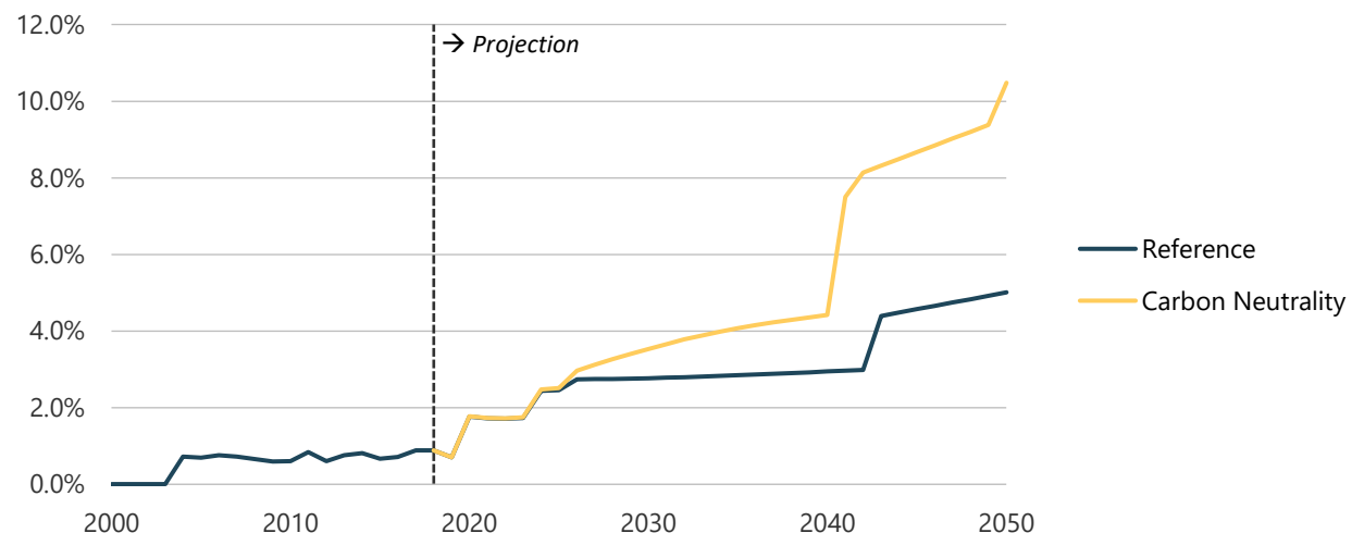
Figure 6-50. Modern renewables share in REF and CN, 2000-2050.
