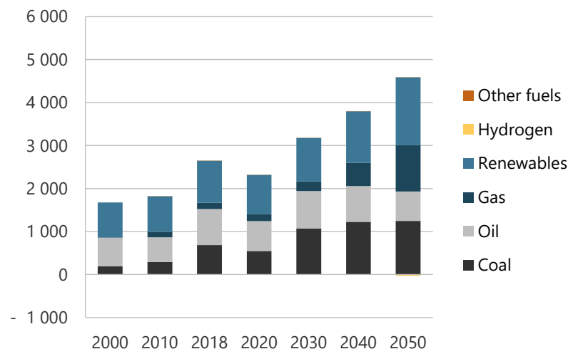
Figure 15-22. Total energy supply in CN, 2000-2050 (PJ).
