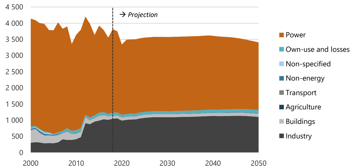
Figure 16-25. Coal consumption by sector in REF, 2000-2050 (PJ).
