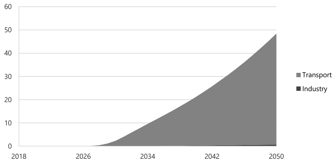
Figure 14-39. Hydrogen consumption by sector in CN, 2000-2050 (PJ).
