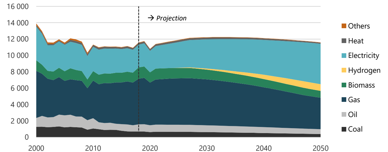
Figure 20-10. Industry energy demand in CN, 2000-2050 (PJ).
