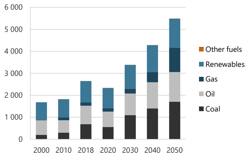
Figure 15-19. Total energy supply in REF, 2000-2050 (PJ).
