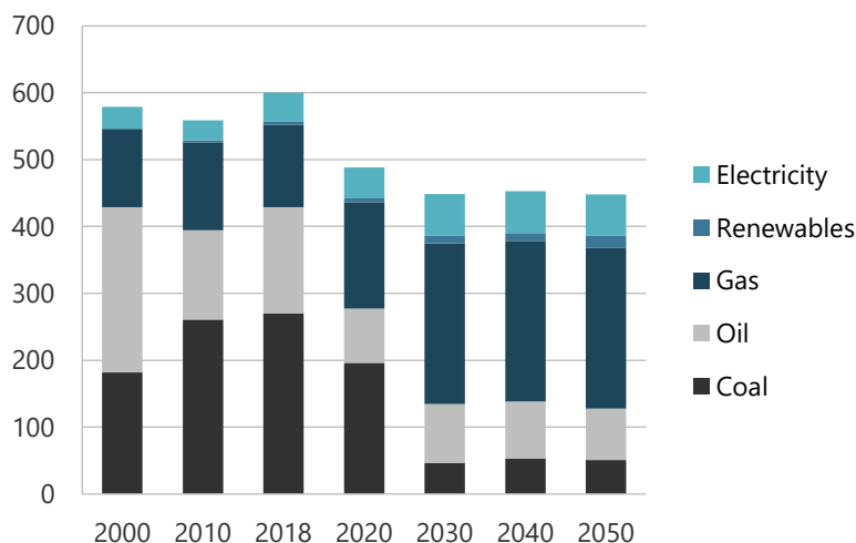
Figure 6-19. Total energy supply in REF, 2000-2050 (PJ).
