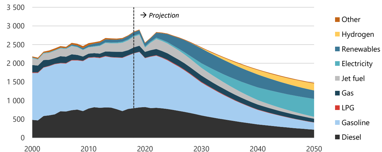
Figure 3-12. Transport energy demand in CN, 2000-2050 (PJ).
