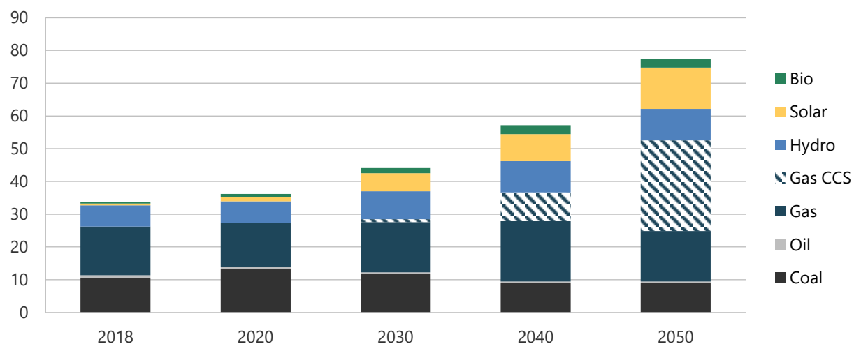
Figure 10-16. Generation capacity in CN, 2018-2050 (GW).
