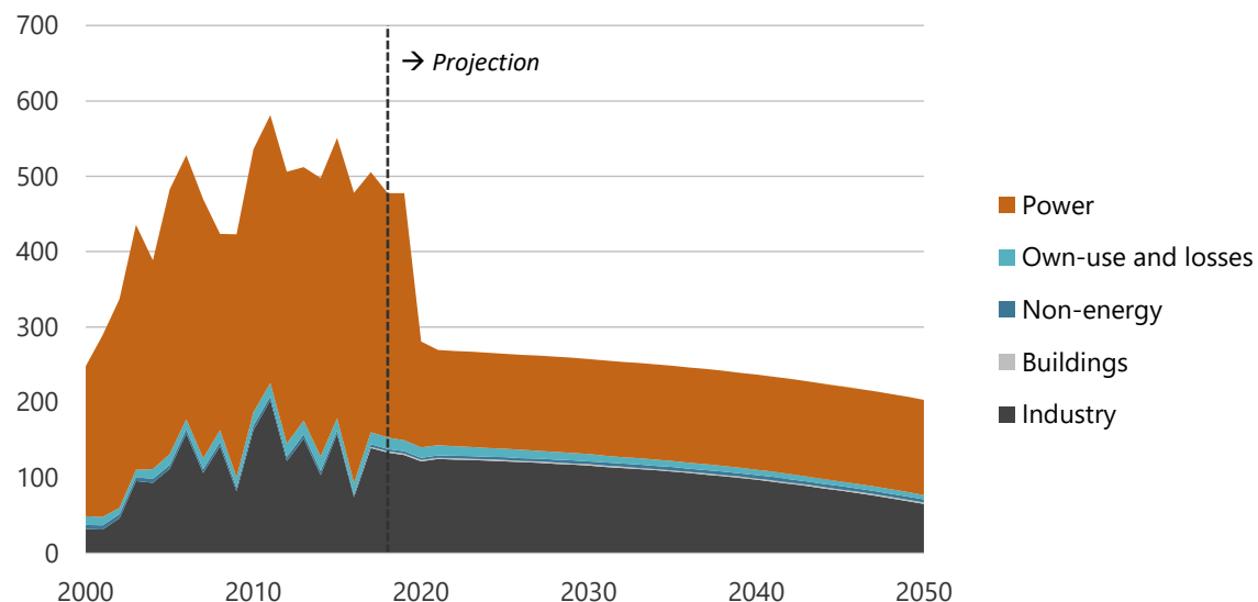
Figure 11-23. Coal consumption by sector in REF, 2000-2050 (PJ).
