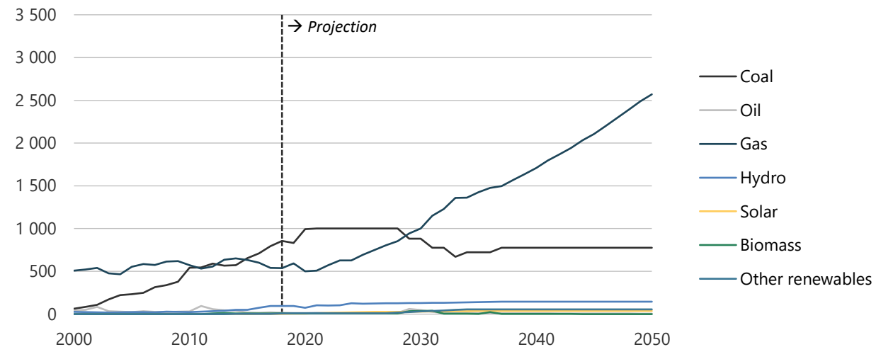
Figure 10-17. Fuel consumption by the power sector in REF, 2000-2050 (PJ).
