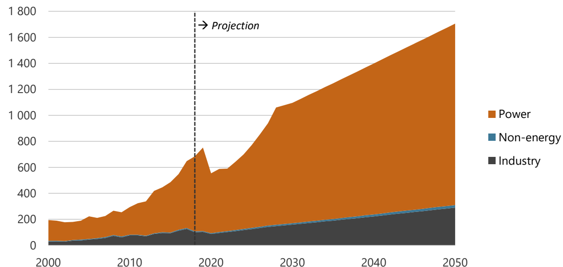
Figure 15-25. Coal consumption by sector in REF, 2000-2050 (PJ).
