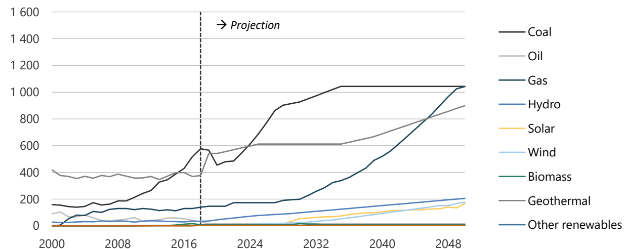
Figure 15-18. Fuel consumption by the power sector in CN, 2000-2050 (PJ).
