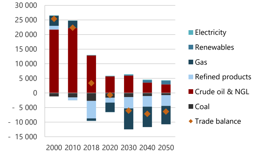
Figure 20-24. Net energy trade in CN, 2000-2050 (PJ).
