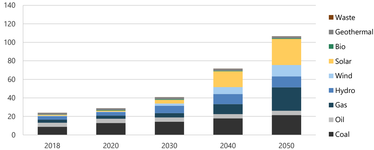
Figure 15-15. Generation capacity in REF, 2018-2050 (GW).
