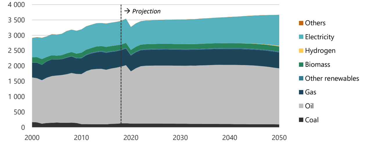
Figure 1-3. Energy demand in REF, 2000-2050 (PJ).
